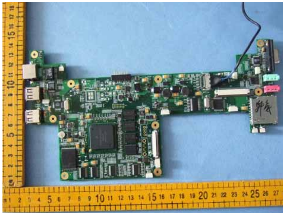
Figure 11 PCB of the EUT Front-View 1
