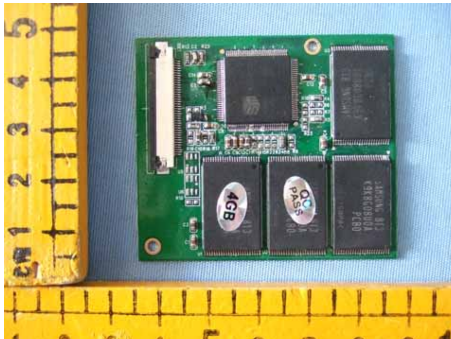
Figure 13 PCB of the EUT Front-View 2
