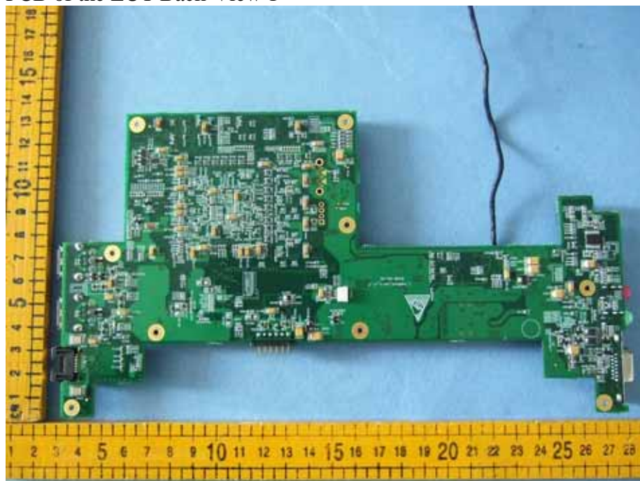
Figure 12 PCB of the EUT Back-View 1
