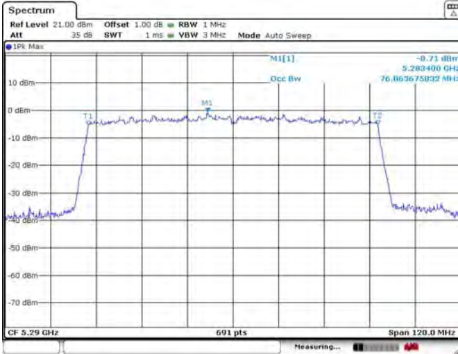
99% Occupied Bandwidth
