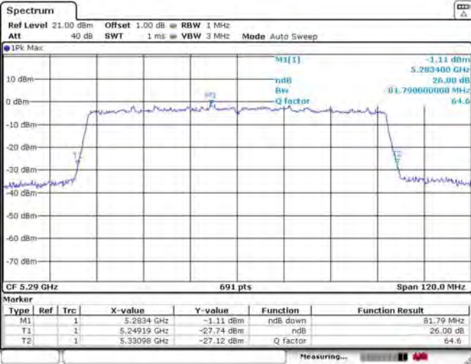
26dB Bandwidth
