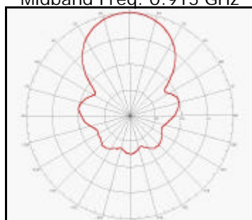
Azimuth Radiation Pattern Midband Freq. 0.915 GHz
