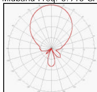
Elevation Radiation Pattern Midband Freq. 0.915 GHz
