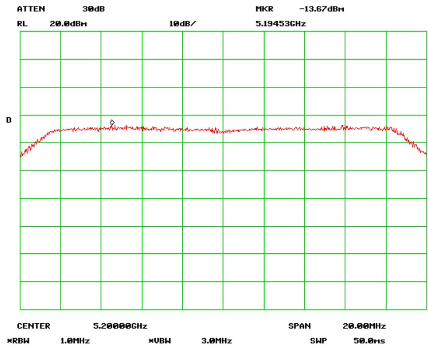
PSD Mid Channel (802.11n-20MHz) chain 0
