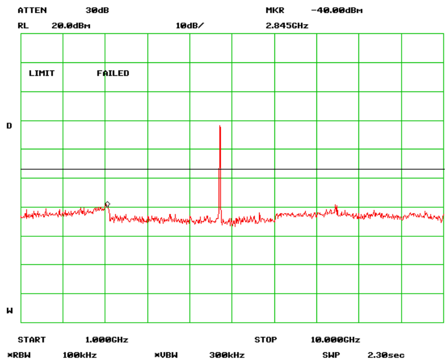
802.11a High Channel -2
