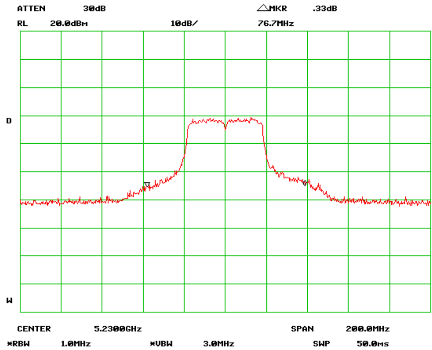
26 dB Bandwidth - High Channel (802.11n-40MHz)
