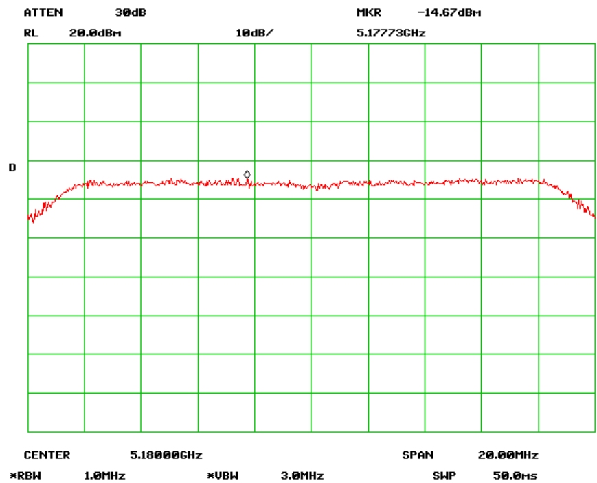
PSD Low Channel (802.11n-20MHz) chain 1
