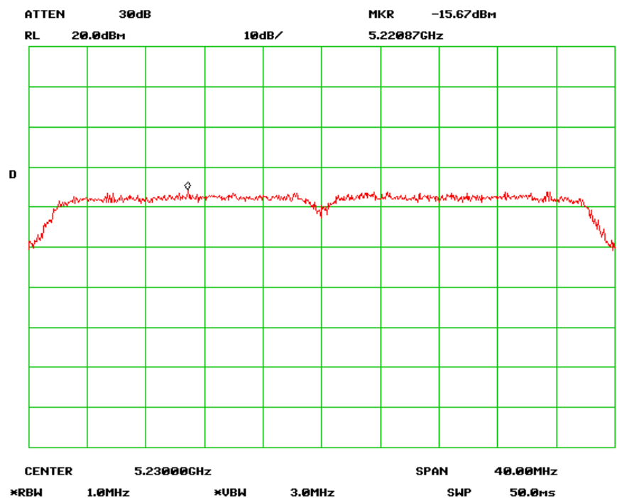
PSD High Channel (802.11n-40MHz) chain 0
