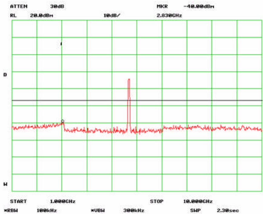
802.11n-40MHz Mid Channel -2
