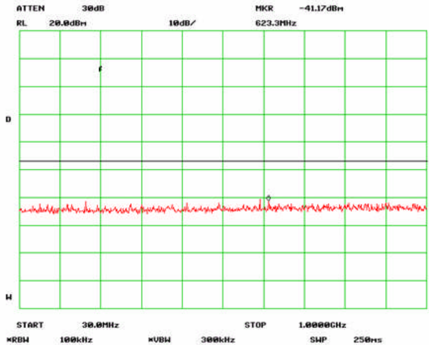
802.11n-20MHz Low Channel -1
