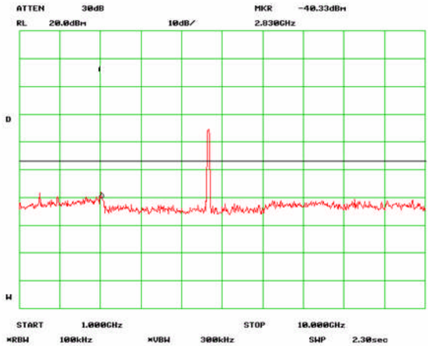
802.11n-40MHz Low Channel -2
