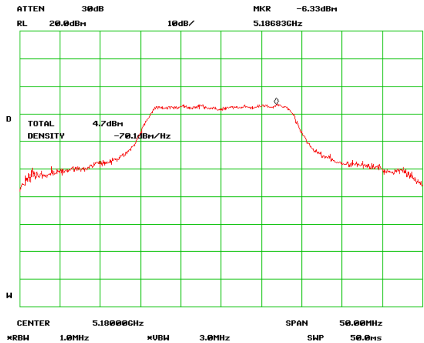
Output Power Low Channel (802.11n-20MHz) channel 1
