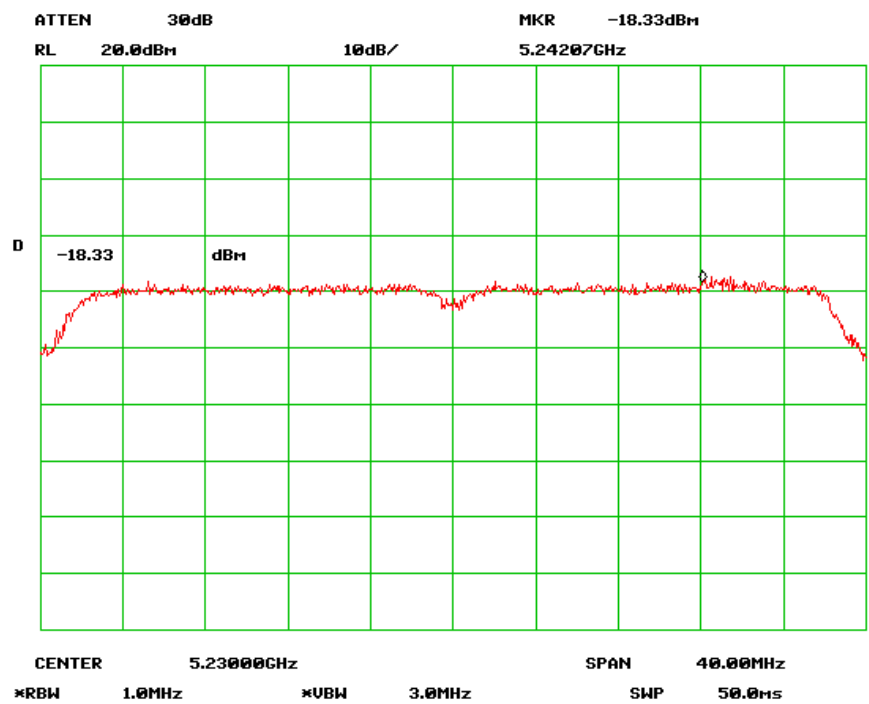
PSD High Channel (802.11n-40MHz) chain 1
