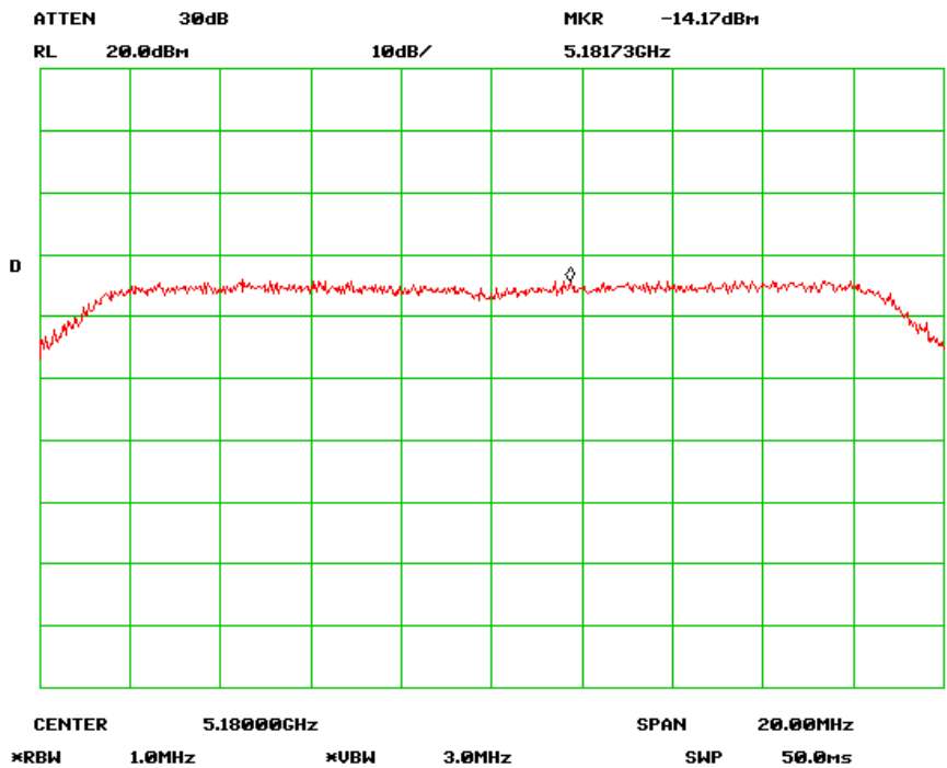
PSD Low Channel (802.11n-20MHz) chain 0
