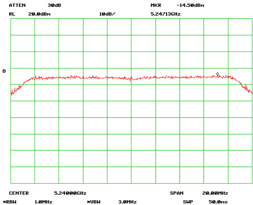
PSD High Channel (802.11n-20MHz) chain 1
