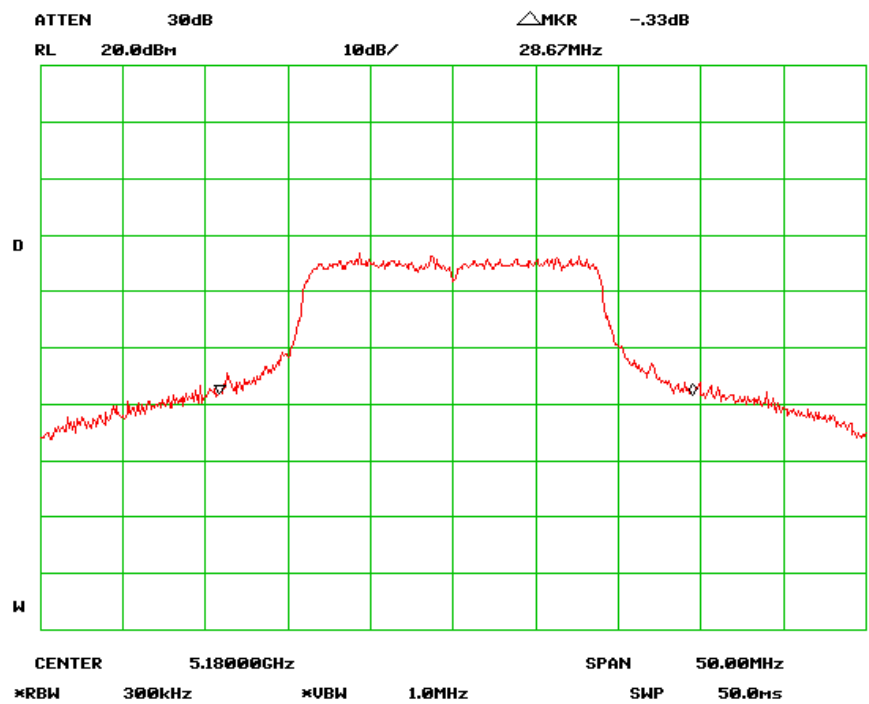
26 dB Bandwidth - Low Channel (802.11n-20MHz)
