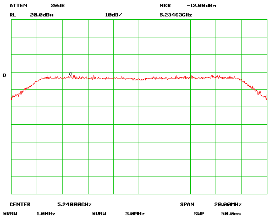
PSD High Channel (802.11a)
