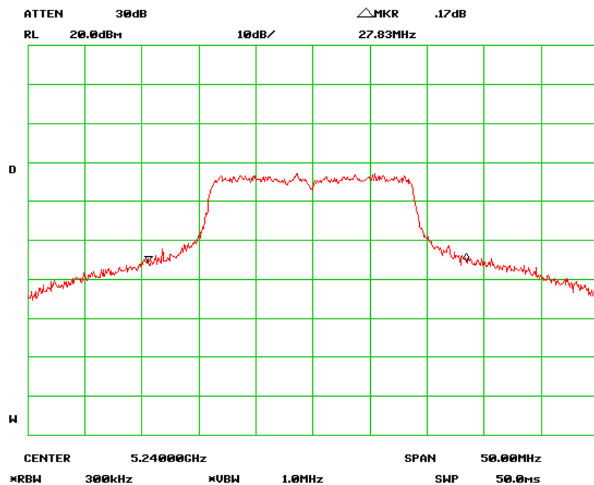
26 dB Bandwidth - High Channel (802.11n-20MHz)
