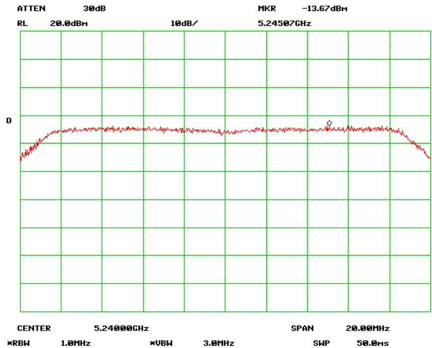
PSD High Channel (802.11n-20MHz) chain 0
