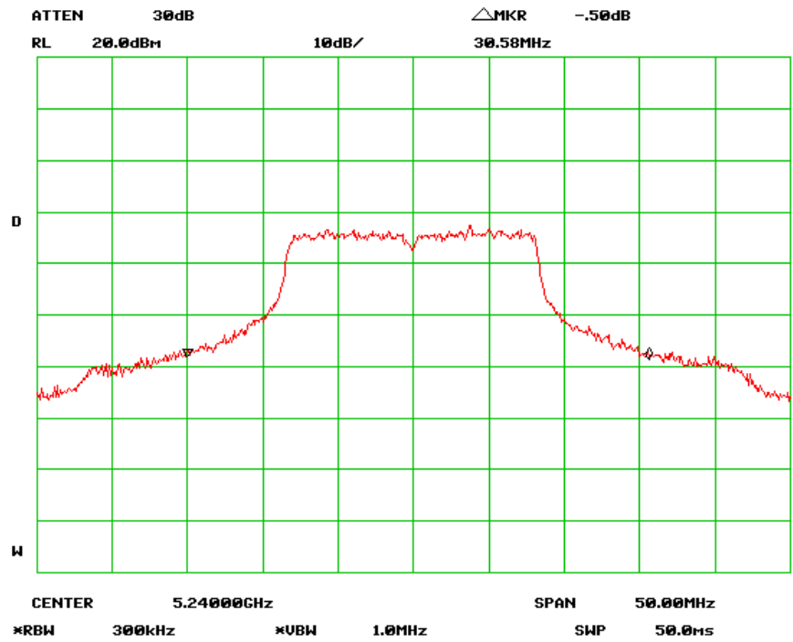
26 dB Bandwidth - High Channel (802.11a)
