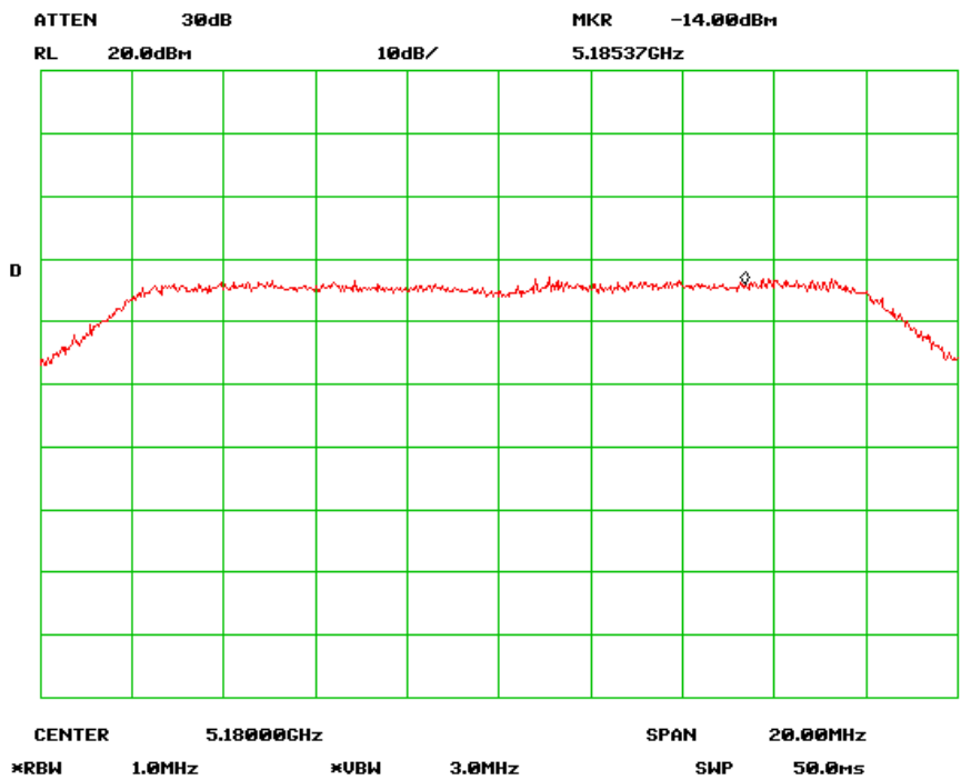
PSD Low Channel (802.11a)
