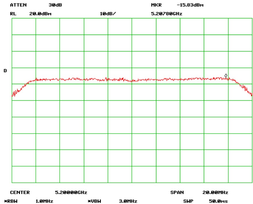
PSD Mid Channel (802.11n-20MHz) chain 1
