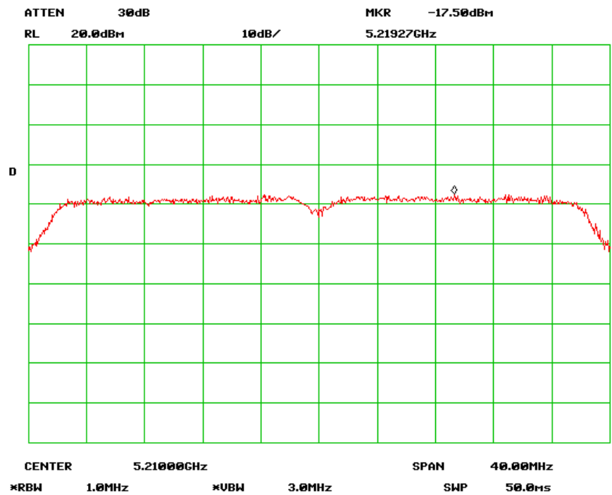
PSD Mid Channel (802.11n-40MHz) chain 0
