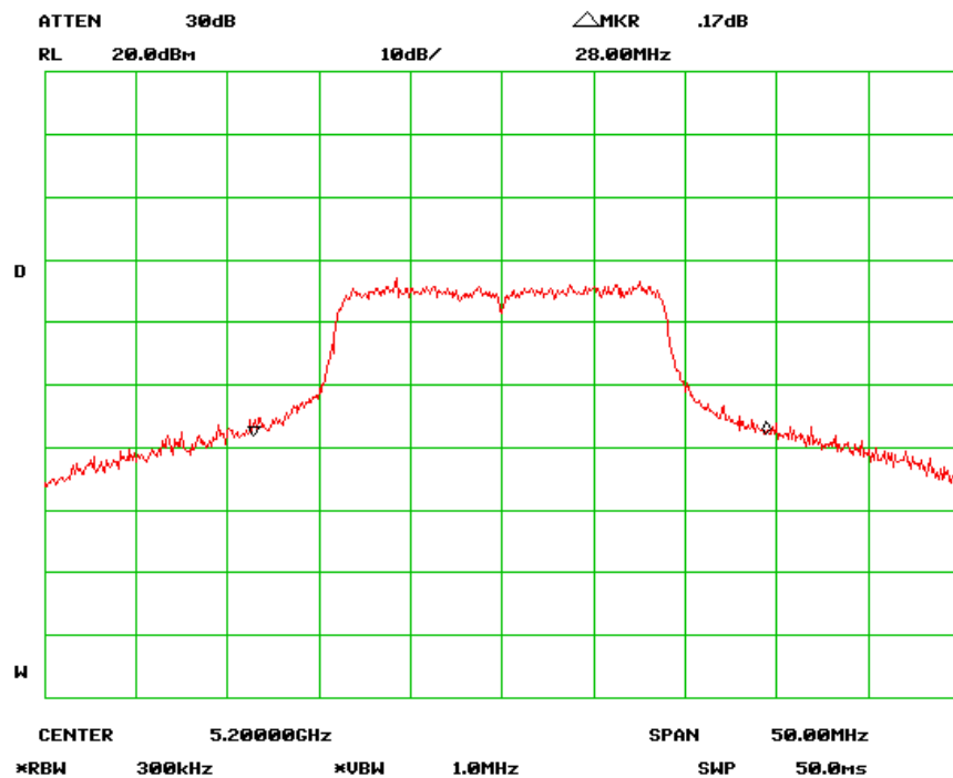
26 dB Bandwidth - Mid Channel (802.11n-20MHz)
