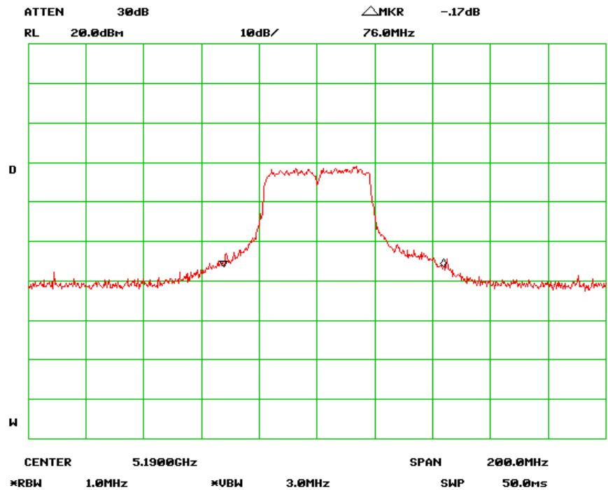
26 dB Bandwidth - Low Channel (802.11n-40MHz)
