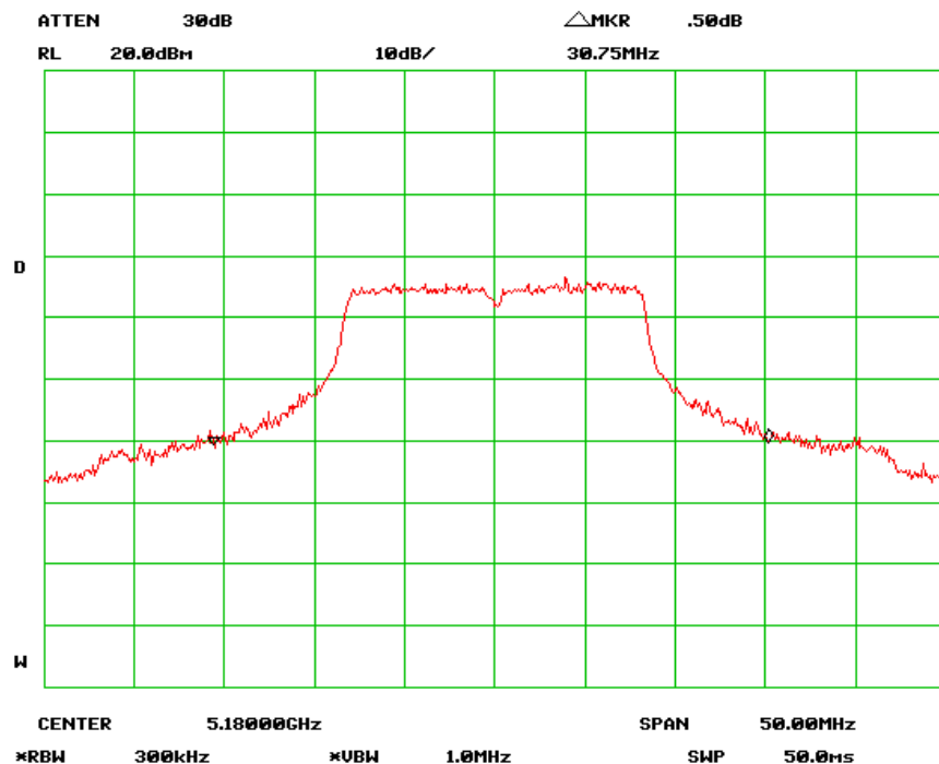
26 dB Bandwidth - Low Channel (802.11a)
