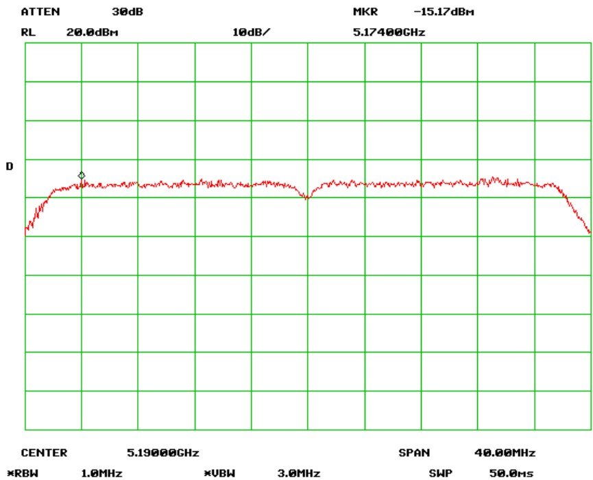
PSD Low Channel (802.11n-40MHz) chain 0
