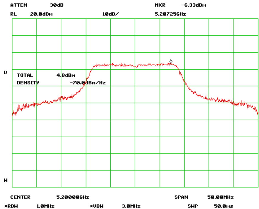
Output Power Mid Channel (802.11n-20MHz) channel 1
