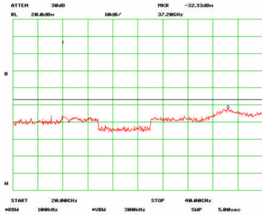
802.11n-40MHz High Channel -4
