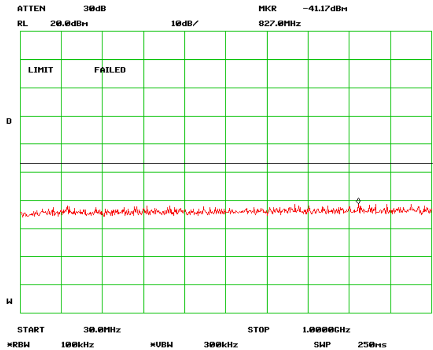
802.11a High Channel -1
