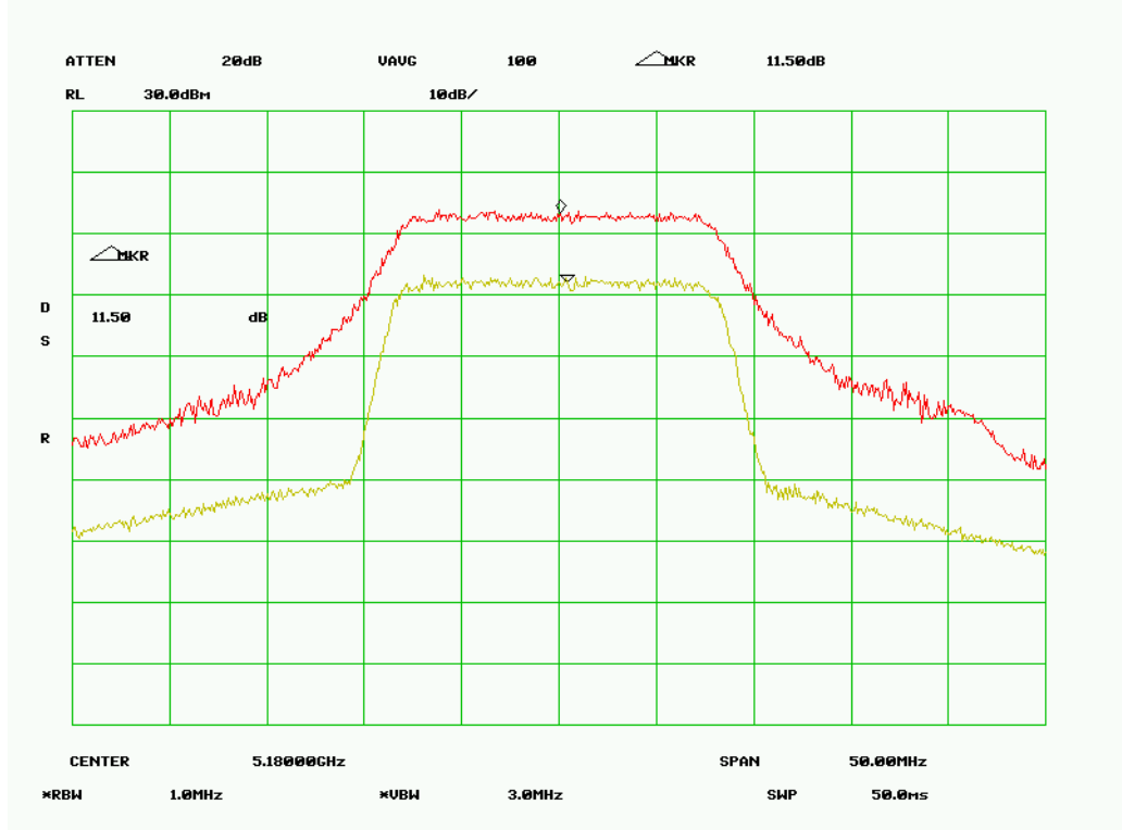
Peak Excursion ratio, 802.11a Low Channel
