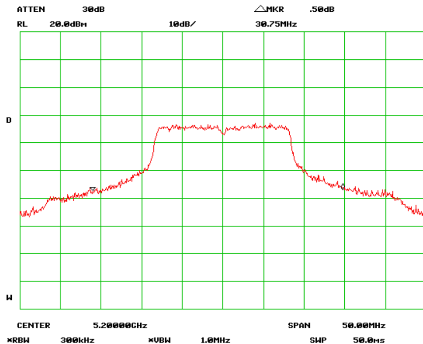
26 dB Bandwidth - Mid Channel (802.11a)
