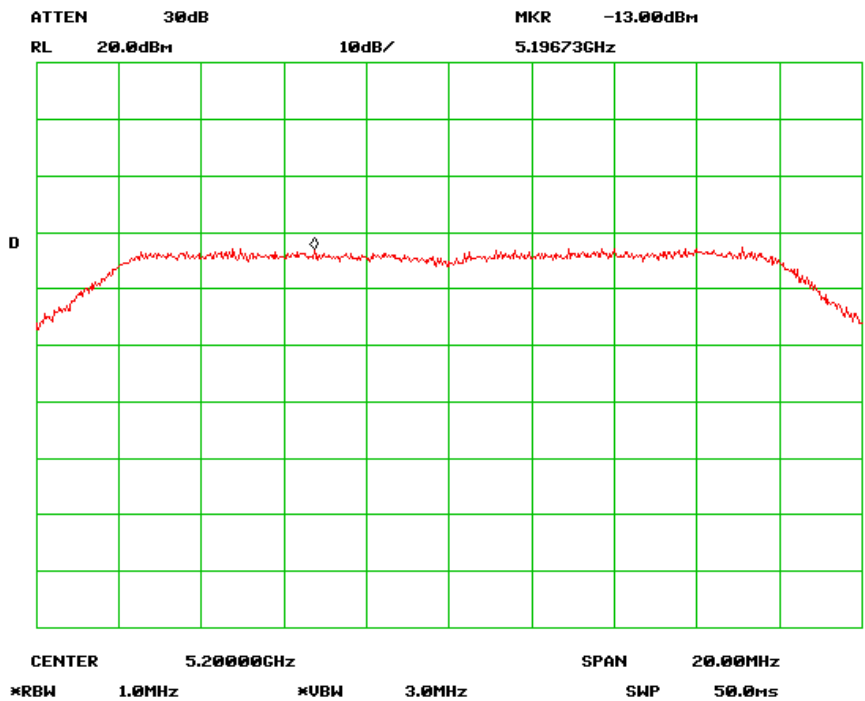
PSD Mid Channel (802.11a)
