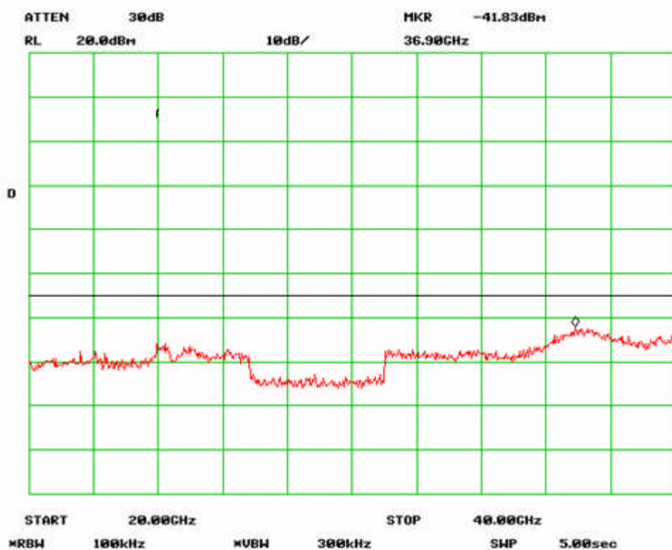
Antenna Port Emission Mid-4 Channel (802.11a)
