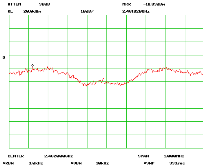
PSD - High Channel (802.11n-20MHz) chain 1
