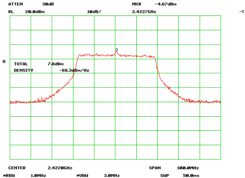
Output Power Low Channel (802.11n-40MHz) chain 0
