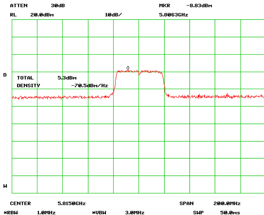
Output Power High Channel (802.11n-40MHz) chain 0
