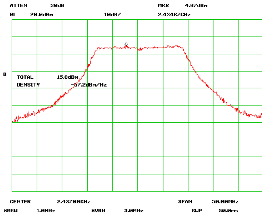
Output Power Mid Channel (802.11n-20MHz) chain 1
