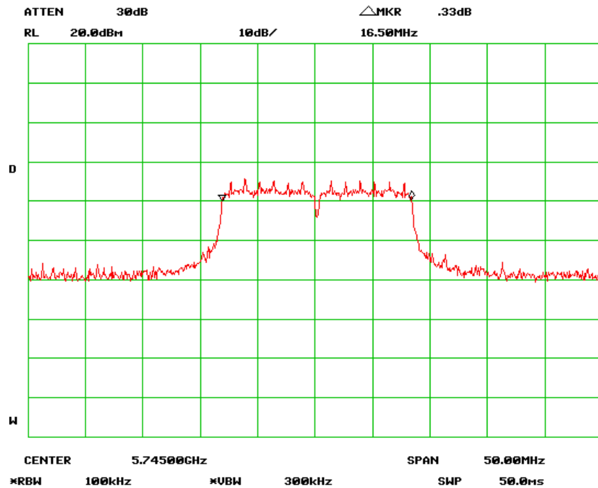
6dB Bandwidth – Low Channel (802.11a)
