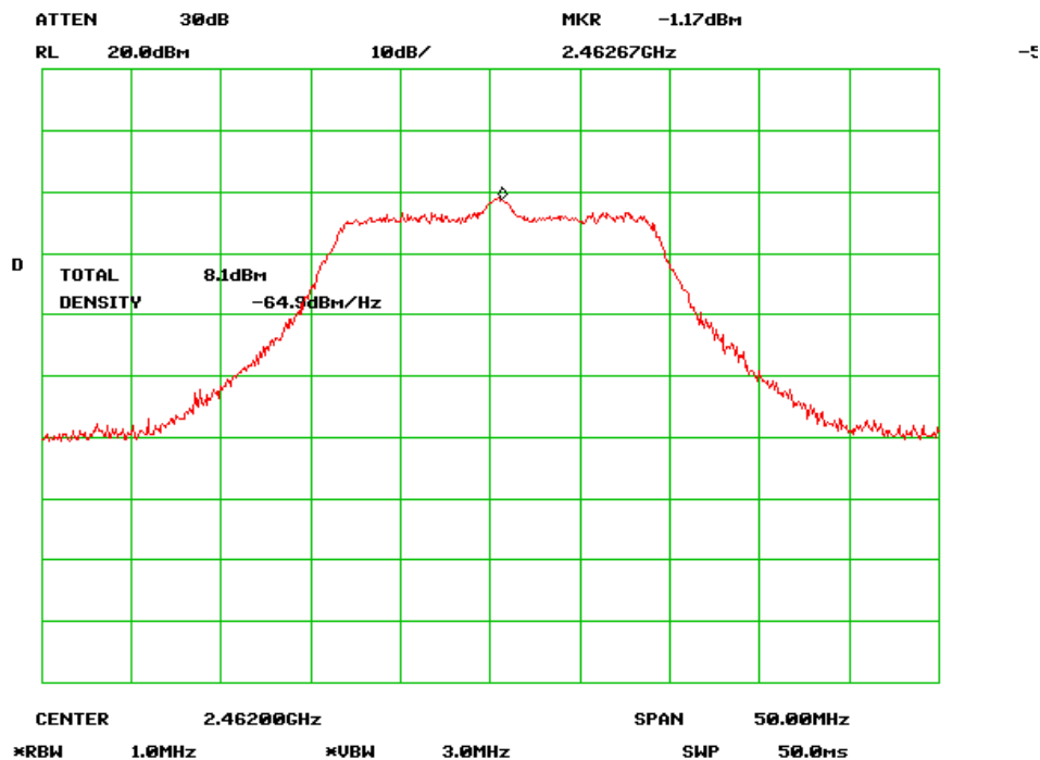
Output Power High Channel (802.11n-20MHz) chain 0
