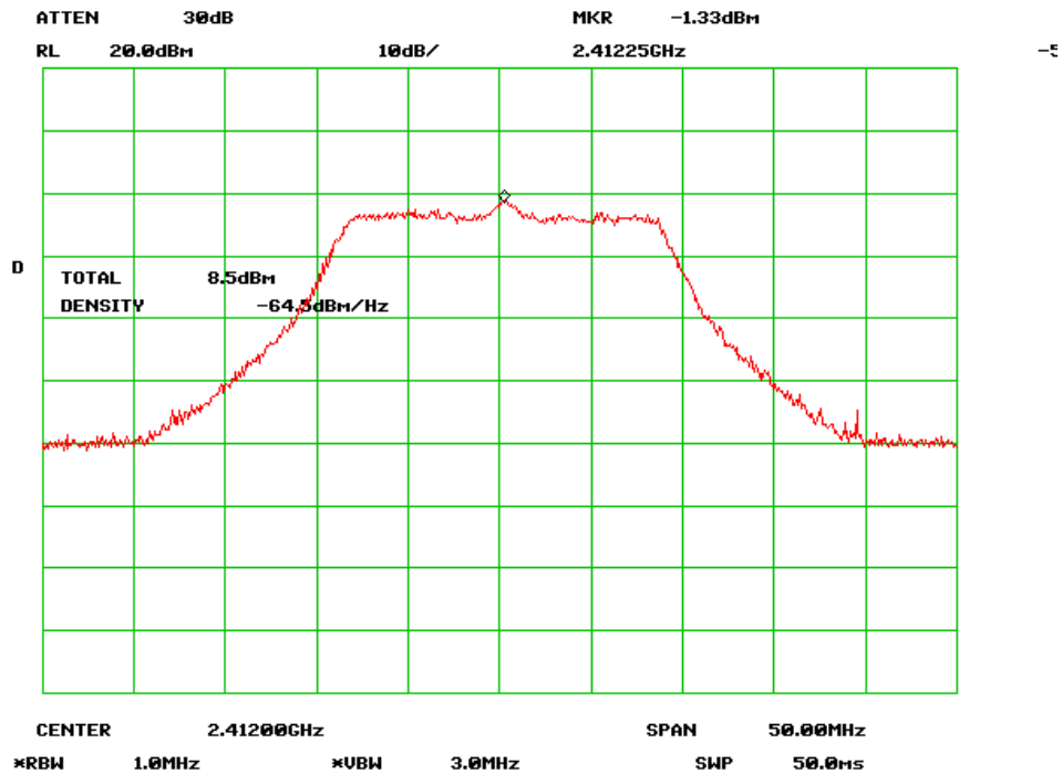
Output Power Low Channel (802.11n-20MHz) chain 0
