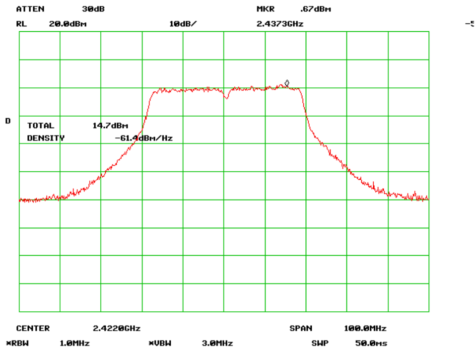
Output Power Low Channel (802.11n-40MHz) chain 1
