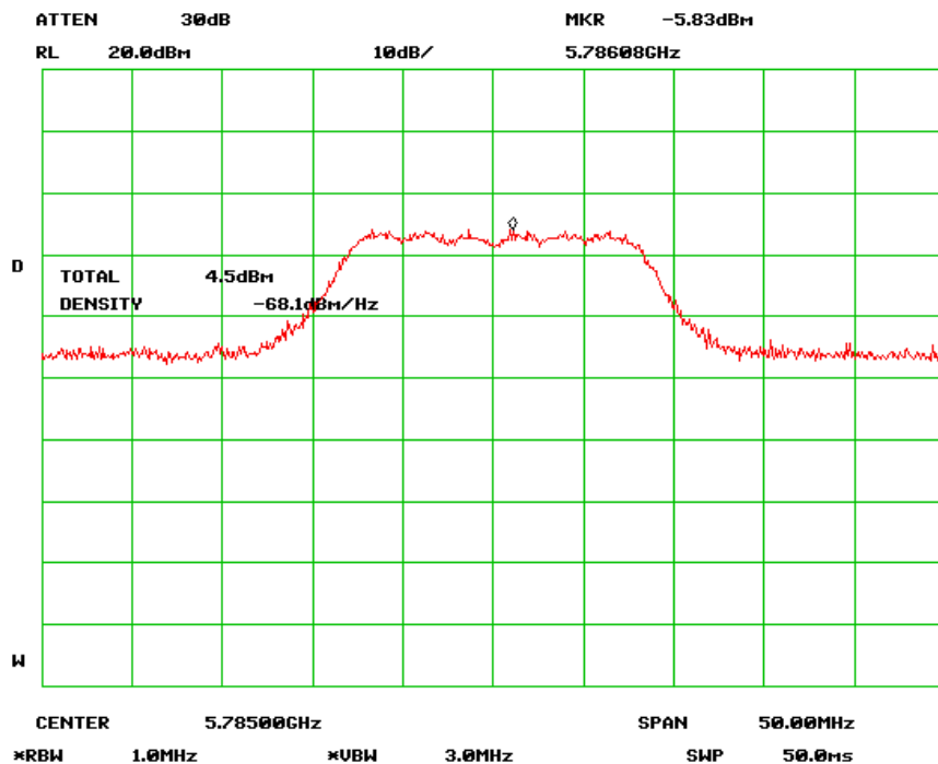
Output Power Mid Channel (802.11n-20MHz) chain 0
