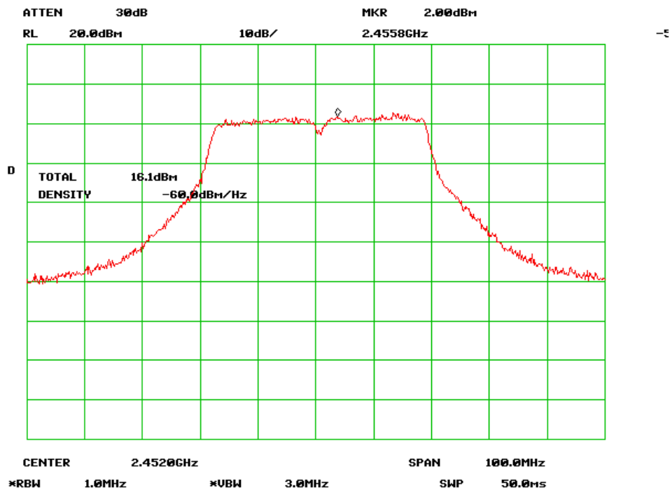
Output Power High Channel (802.11n-40MHz) chain 1
