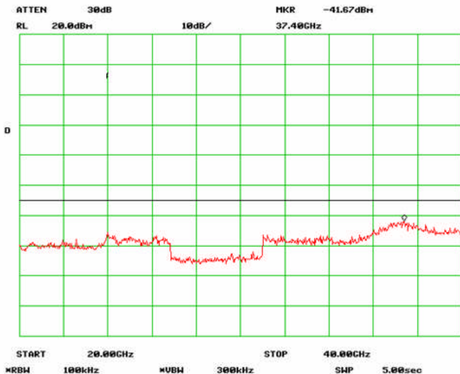
Antenna Port Emission Low-4 Channel (802.11a)
