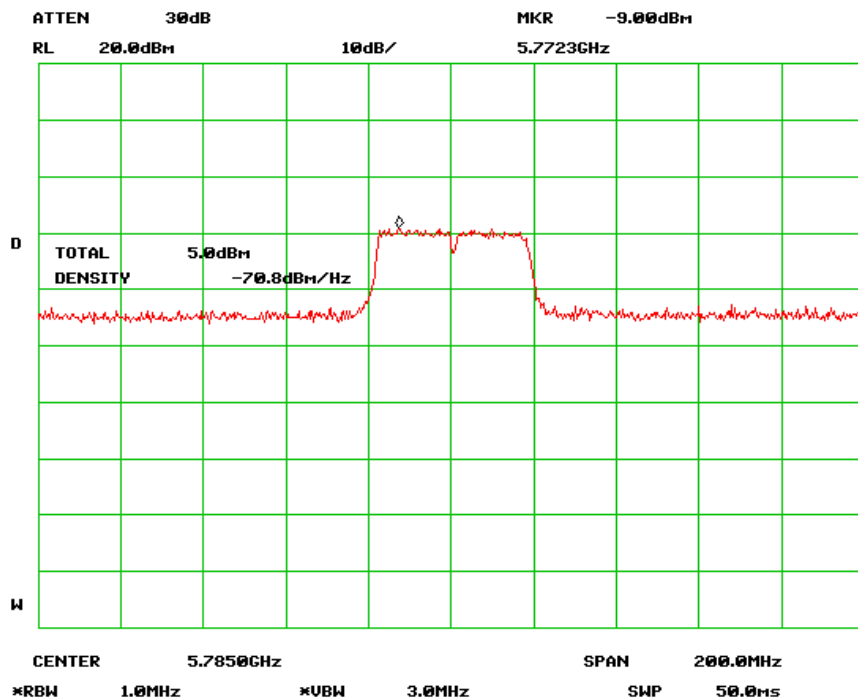
Output Power Mid Channel (802.11n-40MHz) chain 0
