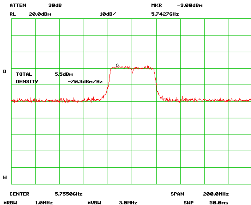
Output Power Low Channel (802.11n-40MHz) chain 1
