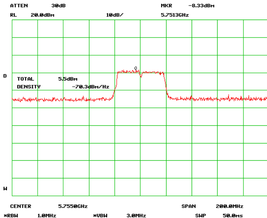
Output Power Low Channel (802.11n-40MHz) chain 0
