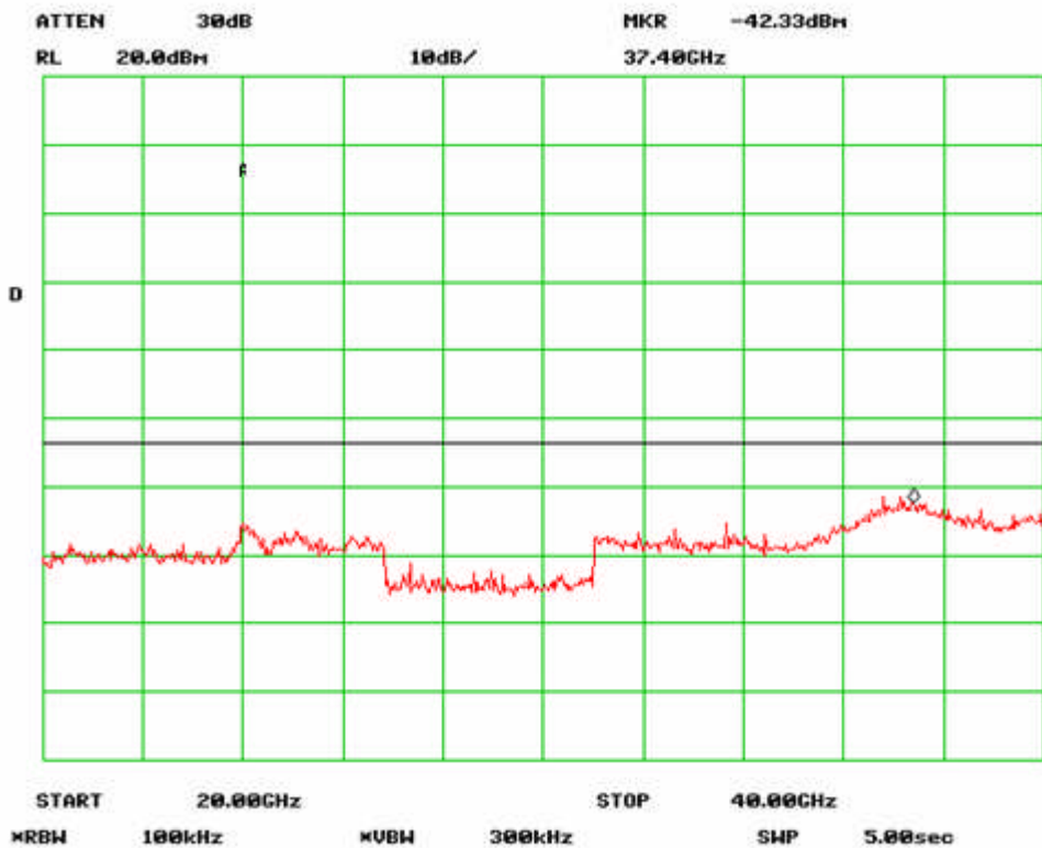
Antenna Port Emission High-4 Channel (802.11a)
