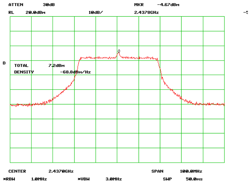
Output Power Mid Channel (802.11n-40MHz) chain 0
