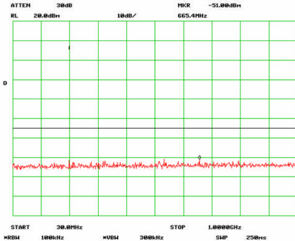
Antenna Port Emission Mid-1 Channel (802.11a)
