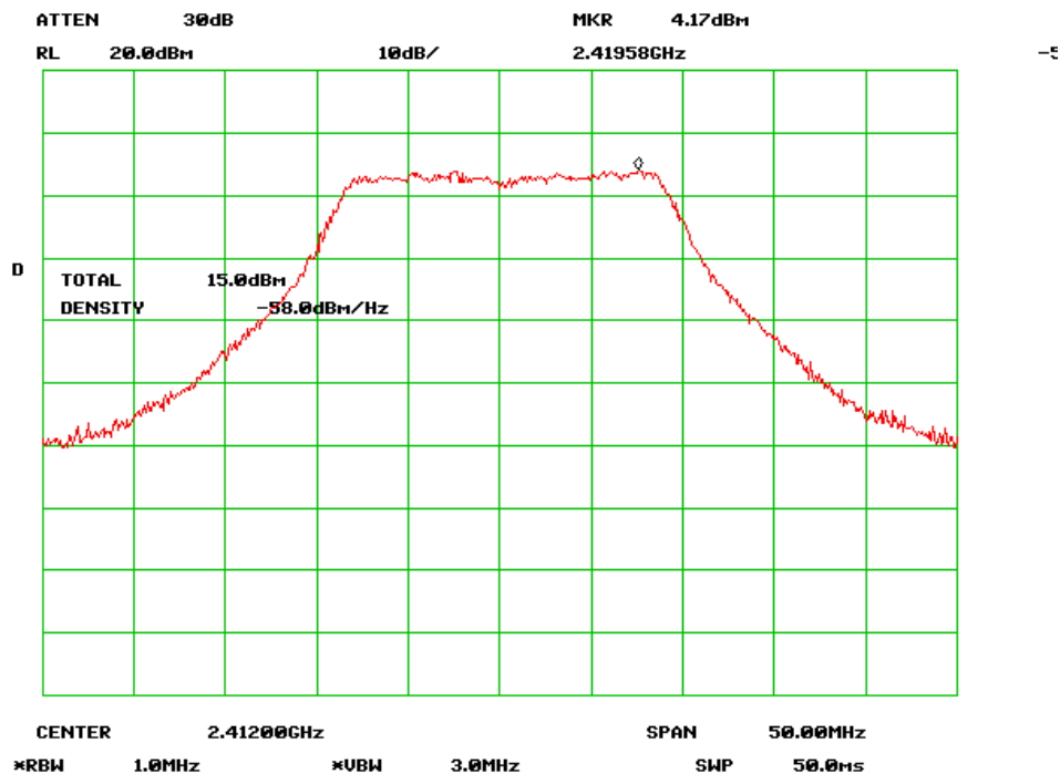
Output Power Low Channel (802.11n-20MHz) chain 1
