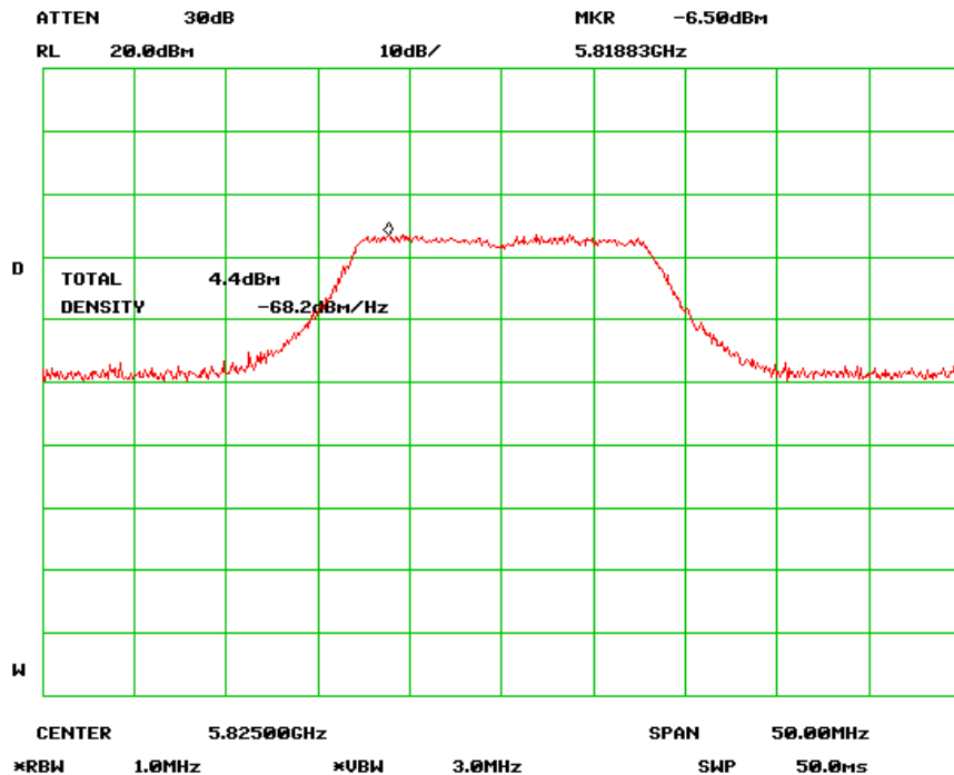
Output Power High Channel (802.11n-20MHz) chain 1
