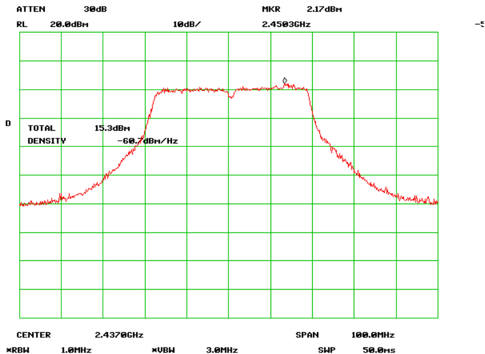
Output Power Mid Channel (802.11n-40MHz) chain 1
