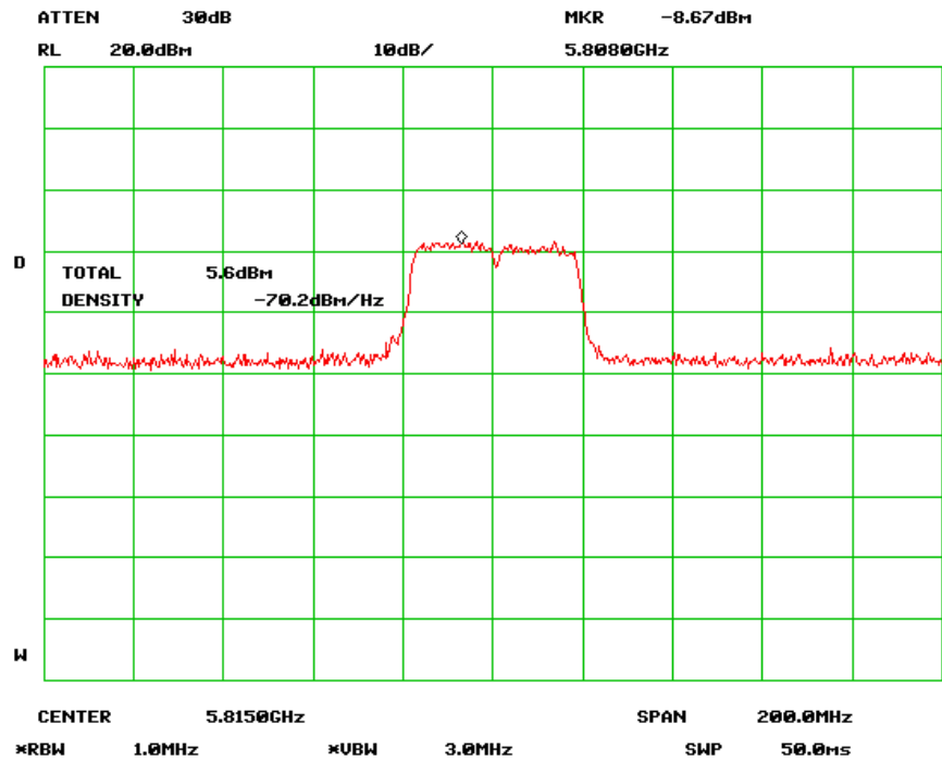
Output Power High Channel (802.11n-40MHz) chain 1
