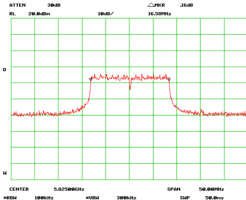
6dB Bandwidth – High Channel (802.11a)
