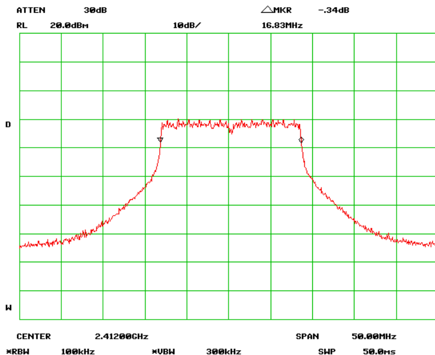
6dB Bandwidth – Low Channel (802.11g)
