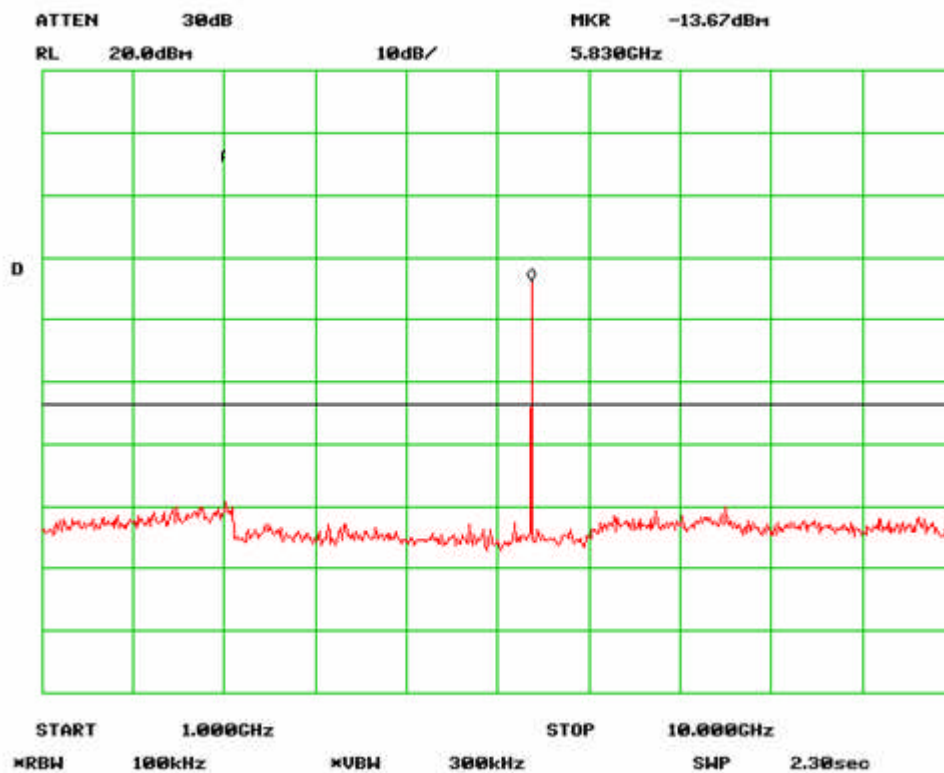
Antenna Port Emission High-2 Channel (802.11a)
