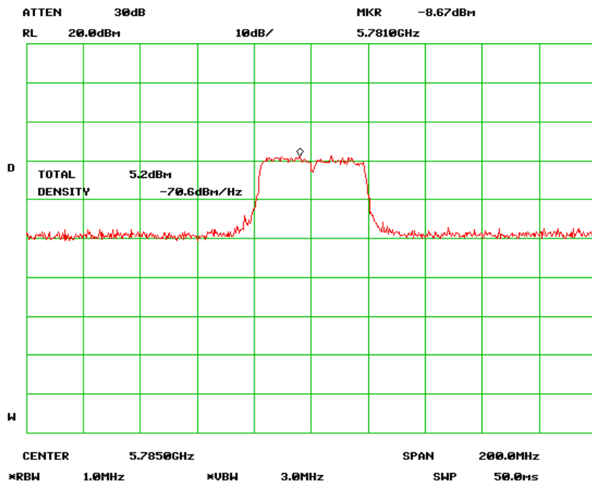
Output Power Mid Channel (802.11n-40MHz) chain 1
