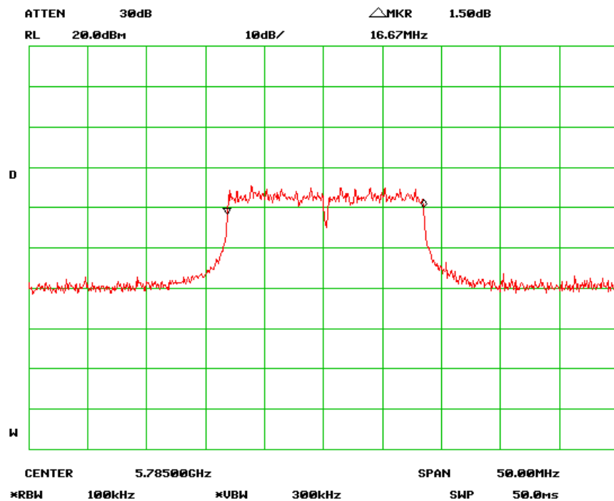
6dB Bandwidth – Mid Channel (802.11a)
