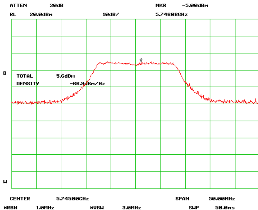
Output Power Low Channel (802.11n-20MHz) chain 1
