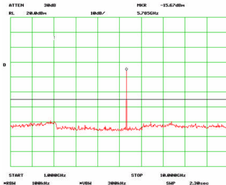
Antenna Port Emission Mid-2 Channel (802.11a)
