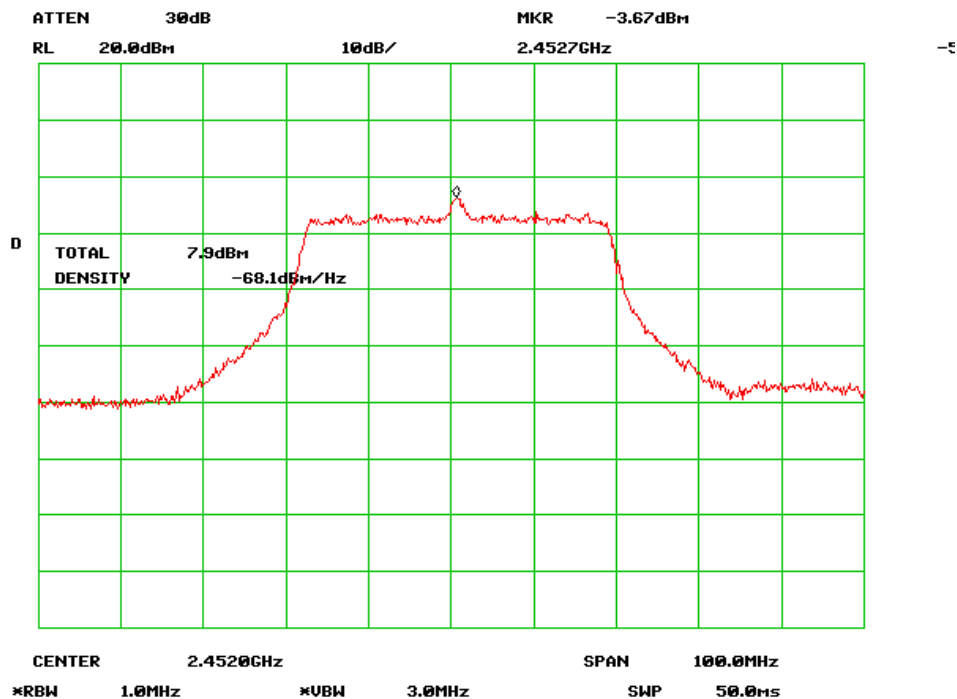
Output Power High Channel (802.11n-40MHz) chain 0
