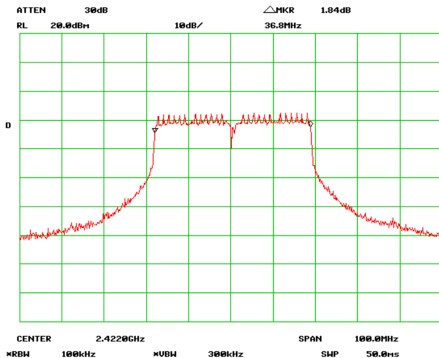
6dB Bandwidth – Low Channel (802.11n-40MHz)
