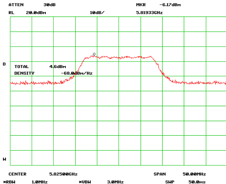
Output Power High Channel (802.11n-20MHz) chain 0
