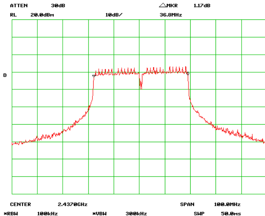
6dB Bandwidth – Mid Channel (802.11n-40MHz)
