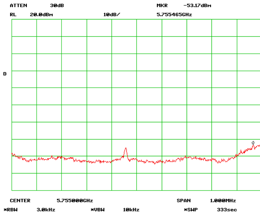
PSD - Low Channel (802.11n-40MHz) chain 0
