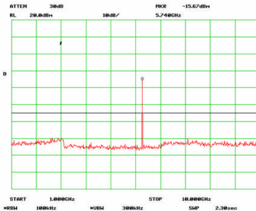
Antenna Port Emission Low-2 Channel (802.11a)
