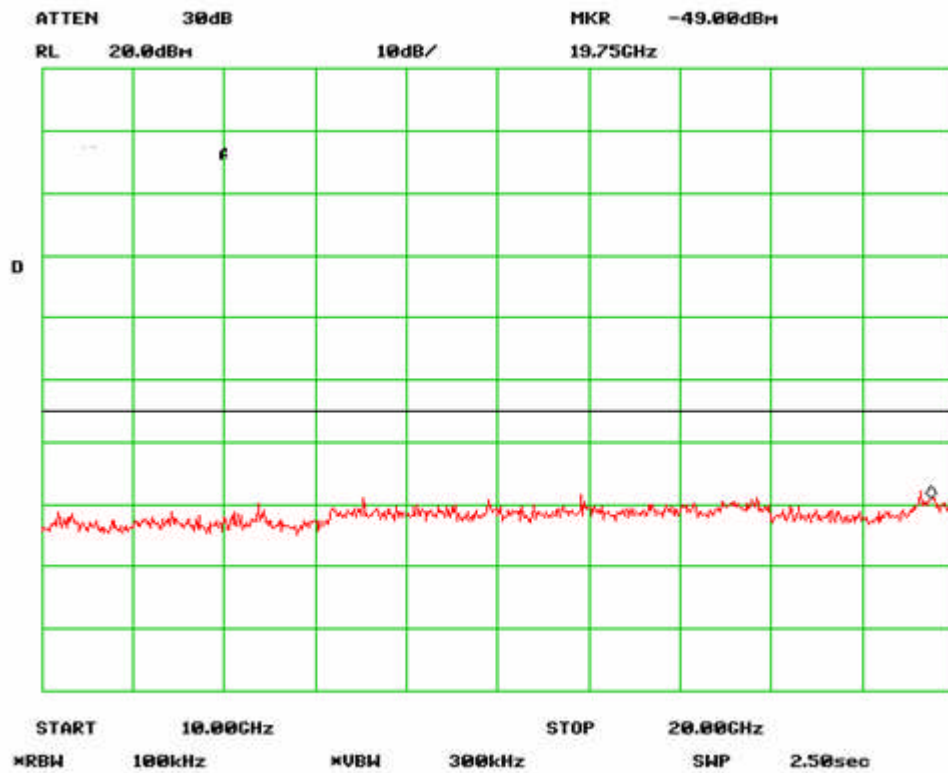
Antenna Port Emission Mid-3 Channel (802.11a)
