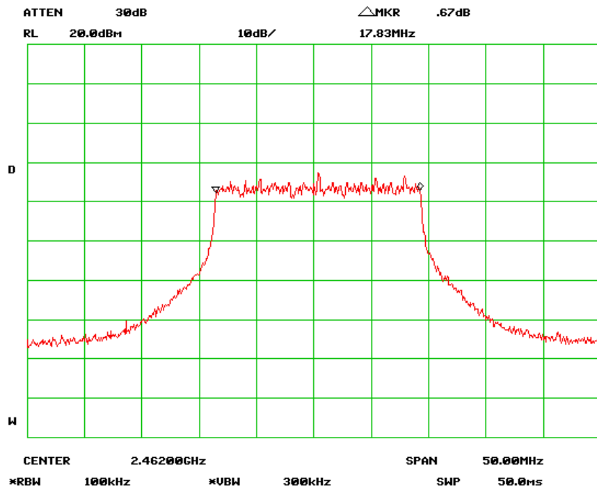
6dB Bandwidth – High Channel (802.11n-20MHz)
