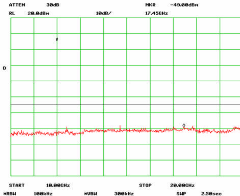
Antenna Port Emission Low-3 Channel (802.11a)
