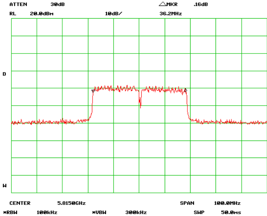
6dB Bandwidth – High Channel (802.11n-40MHz)
