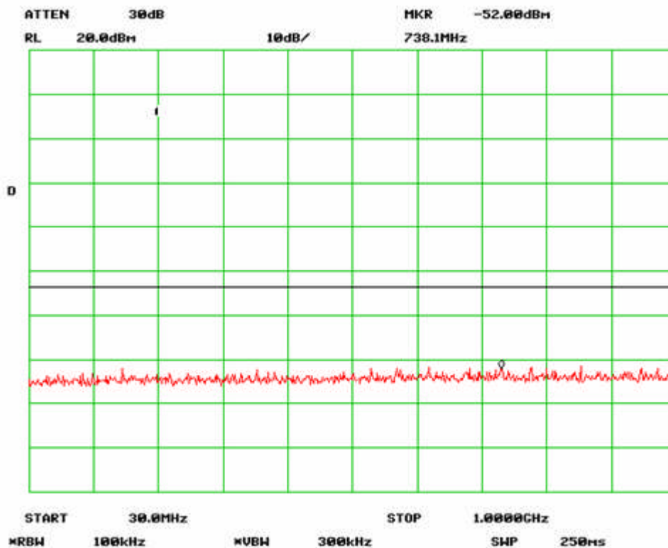
Antenna Port Emission High-1 Channel (802.11n-20MHz)
