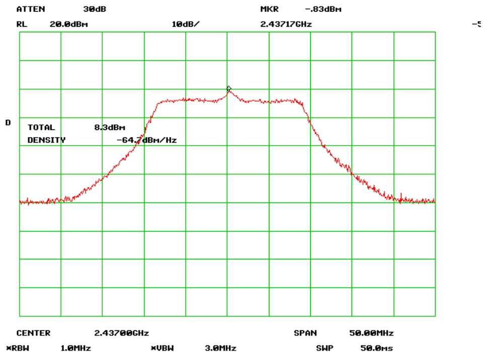
Output Power Mid Channel (802.11n-20MHz) chain 0
