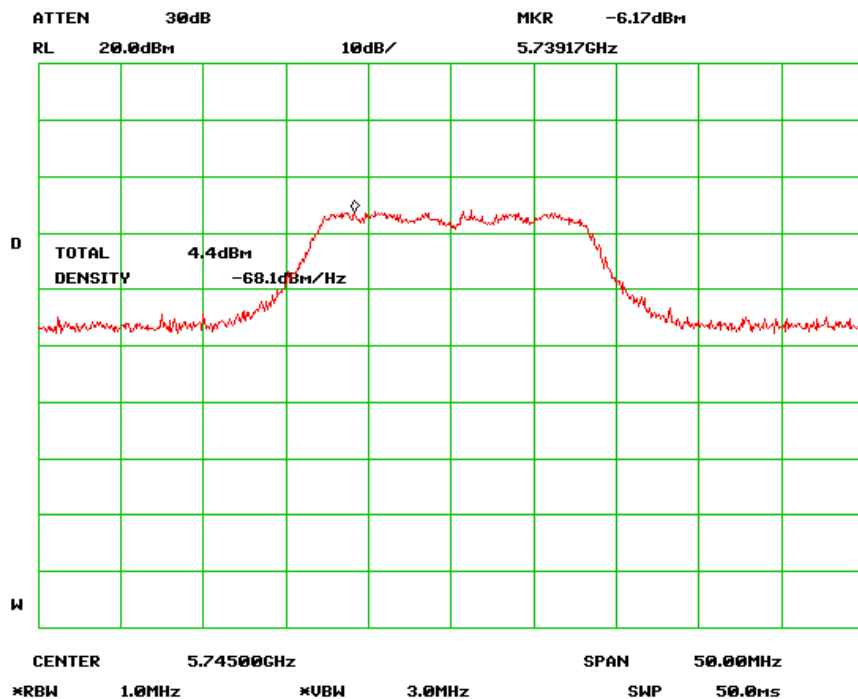
Output Power Low Channel (802.11n-20MHz) chain 0
