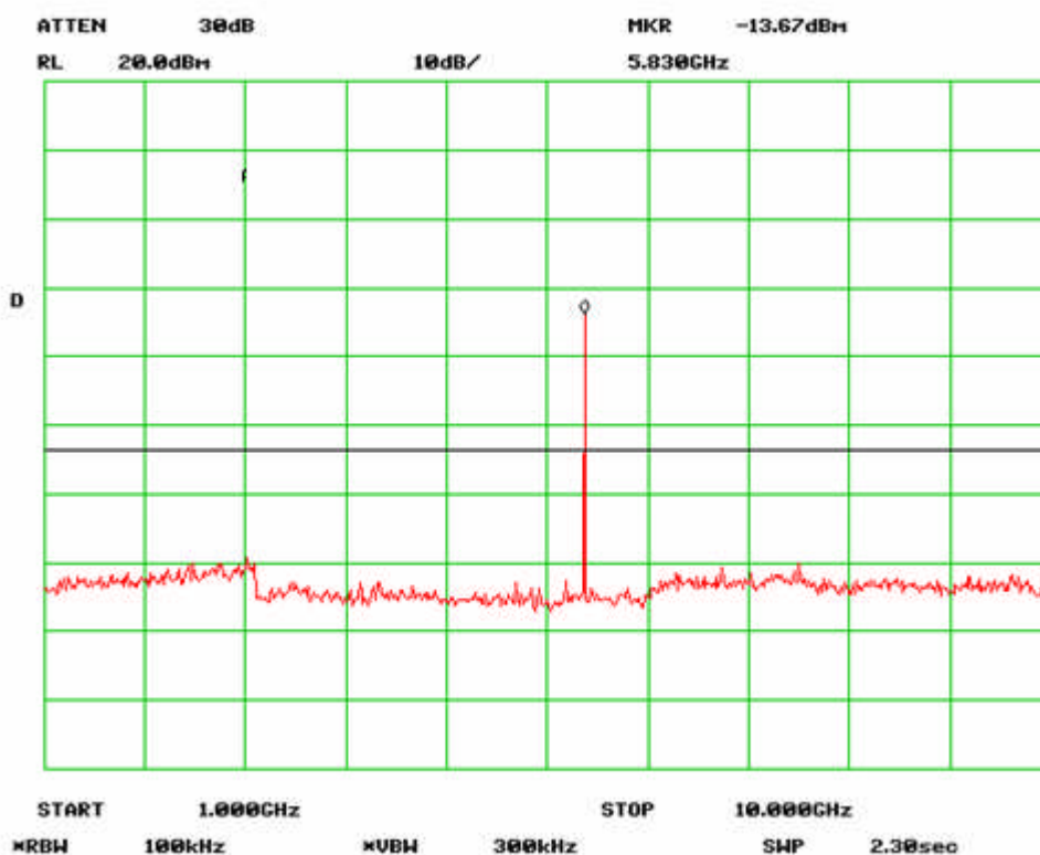
Antenna Port Emission High-2 Channel (802.11n-20MHz)
