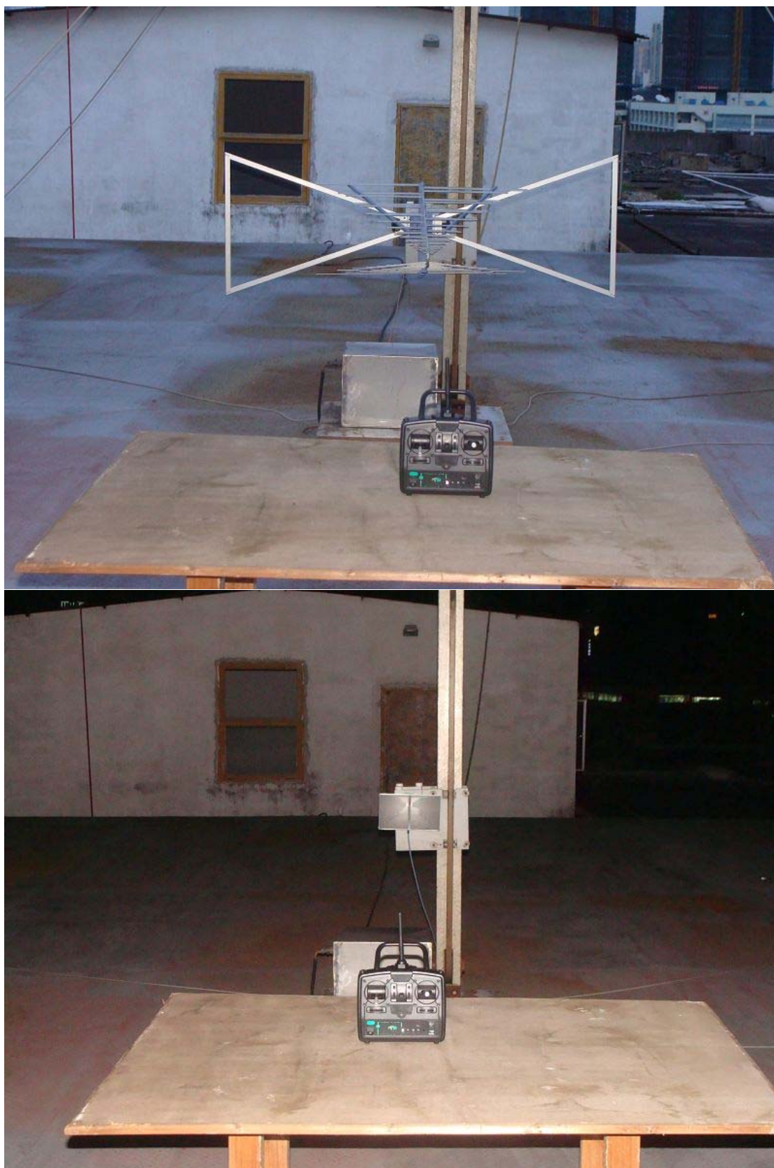
Radiated Emissions
