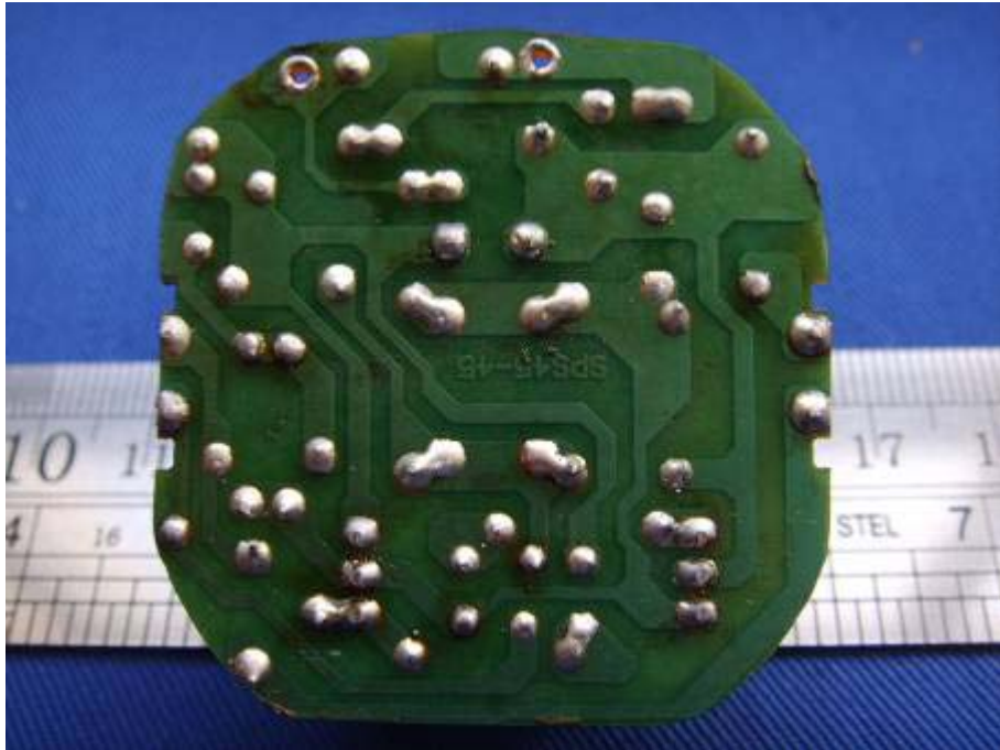
EUT–Solder View (SPS R40)
