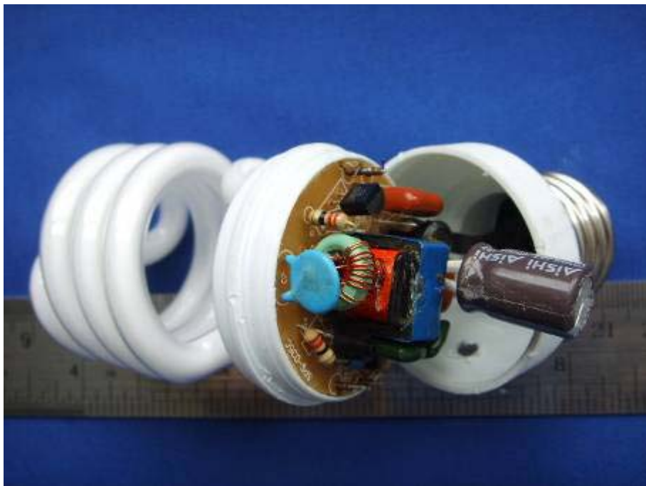
EUT – Uncovered View (SPS T2 11SM/ SPS T2 13SM)
