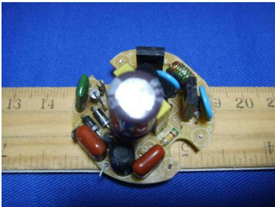
EUT –Components View (SPS T2 13S/ SPS T2 15S)
