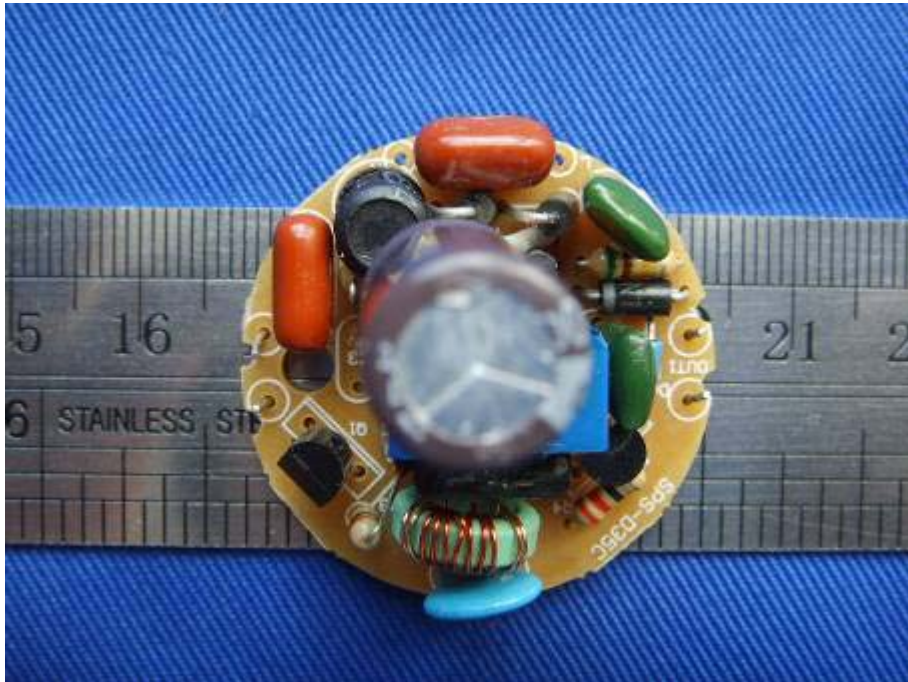
EUT –Components View (SPS T2 11SM/ SPS T2 13SM)
