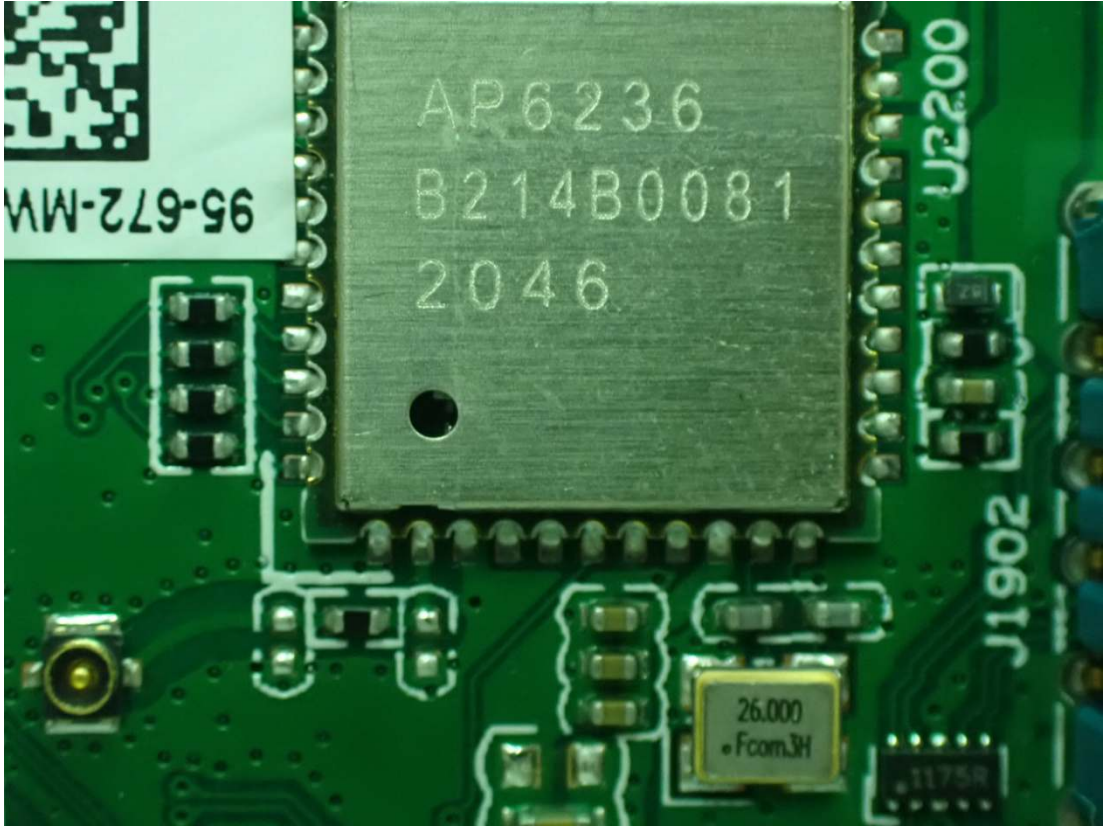
Figure 44 WLAN Combo View
