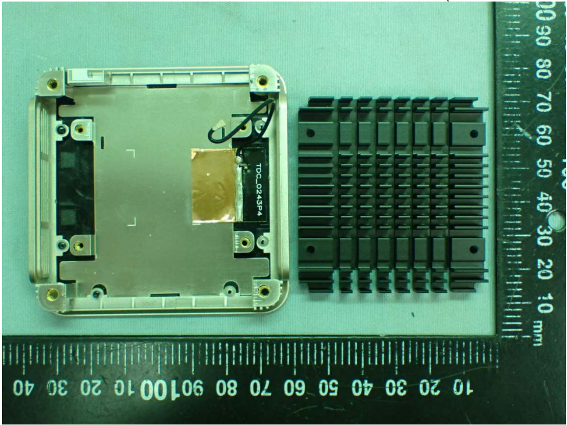
Figure 20 Internal View (Removed Cover)
