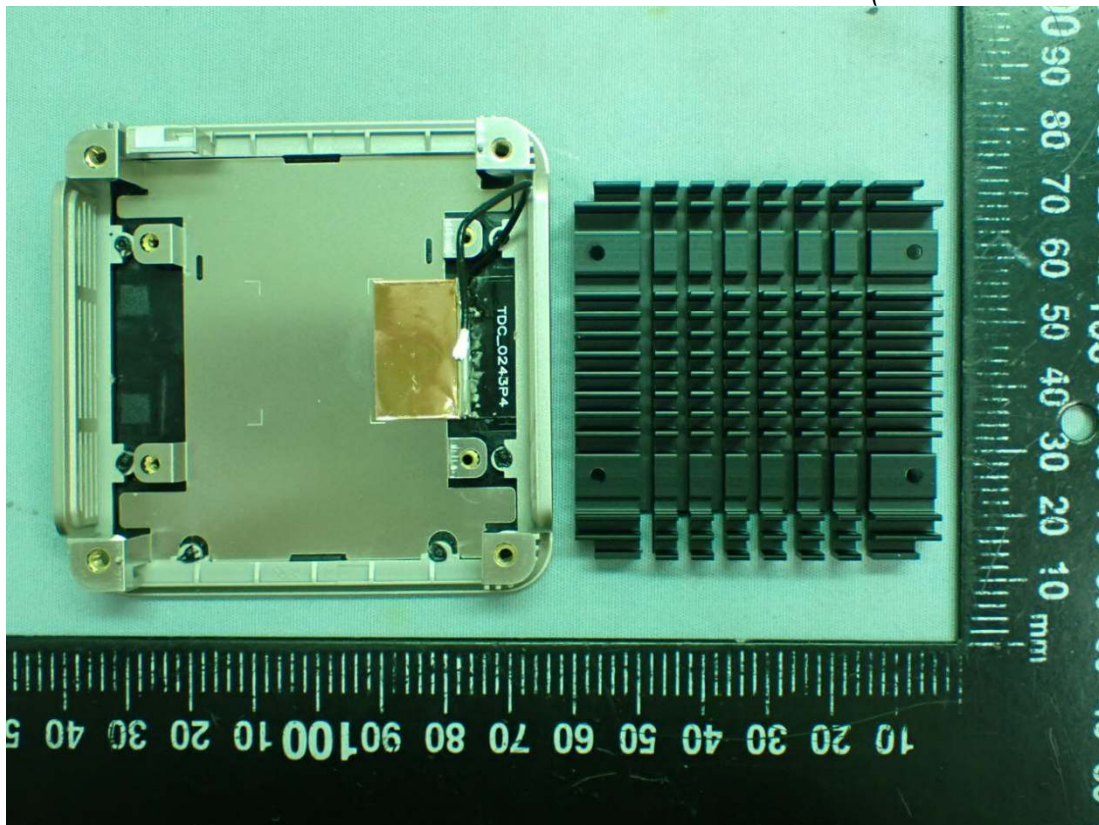
Figure 36 Internal View (Removed Cover)
