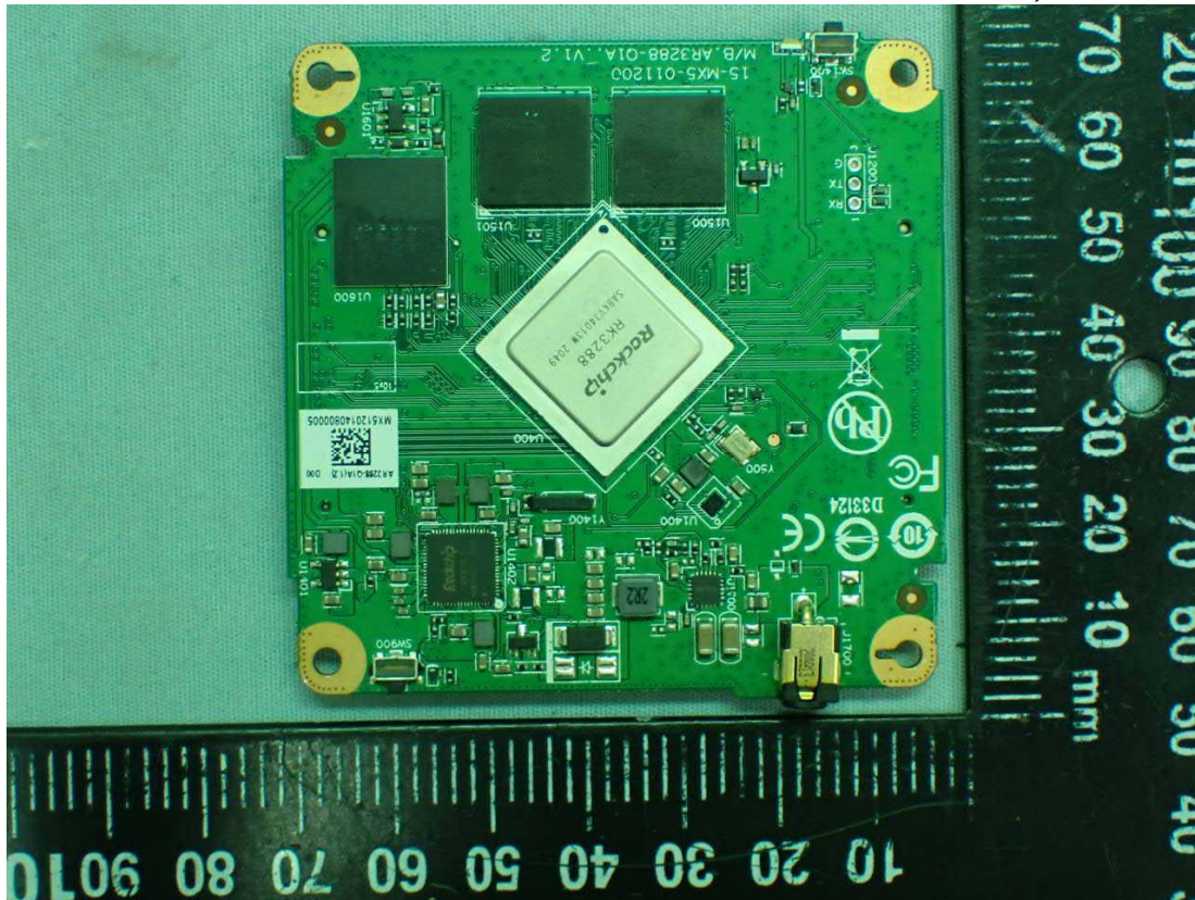
Figure 21 Mother Board, Front View
