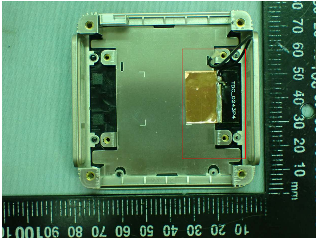
Figure 31 RF Antenna Location
