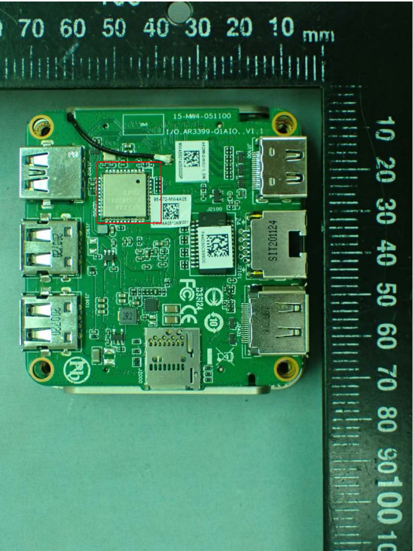
Figure 39 I/O Board, Front View (RF Antenna Location)
