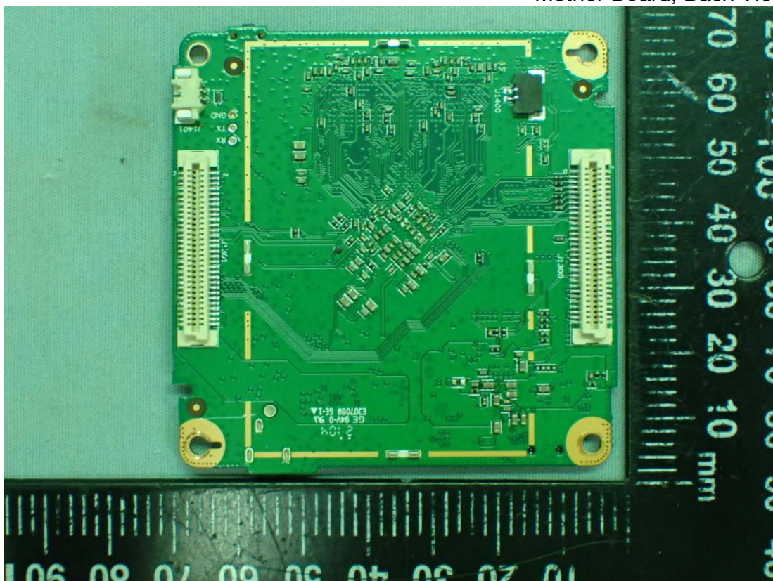
Figure 22 Mother Board, Back View
