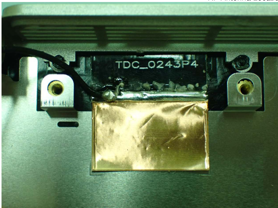
Figure 48 RF Antenna Location
