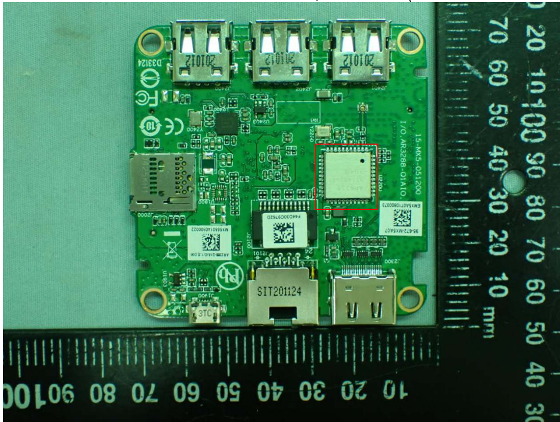
Figure 23 I/O Board, Front View (RF Antenna Location)
