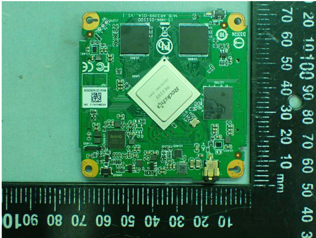
Figure 37 Mother Board, Front View
