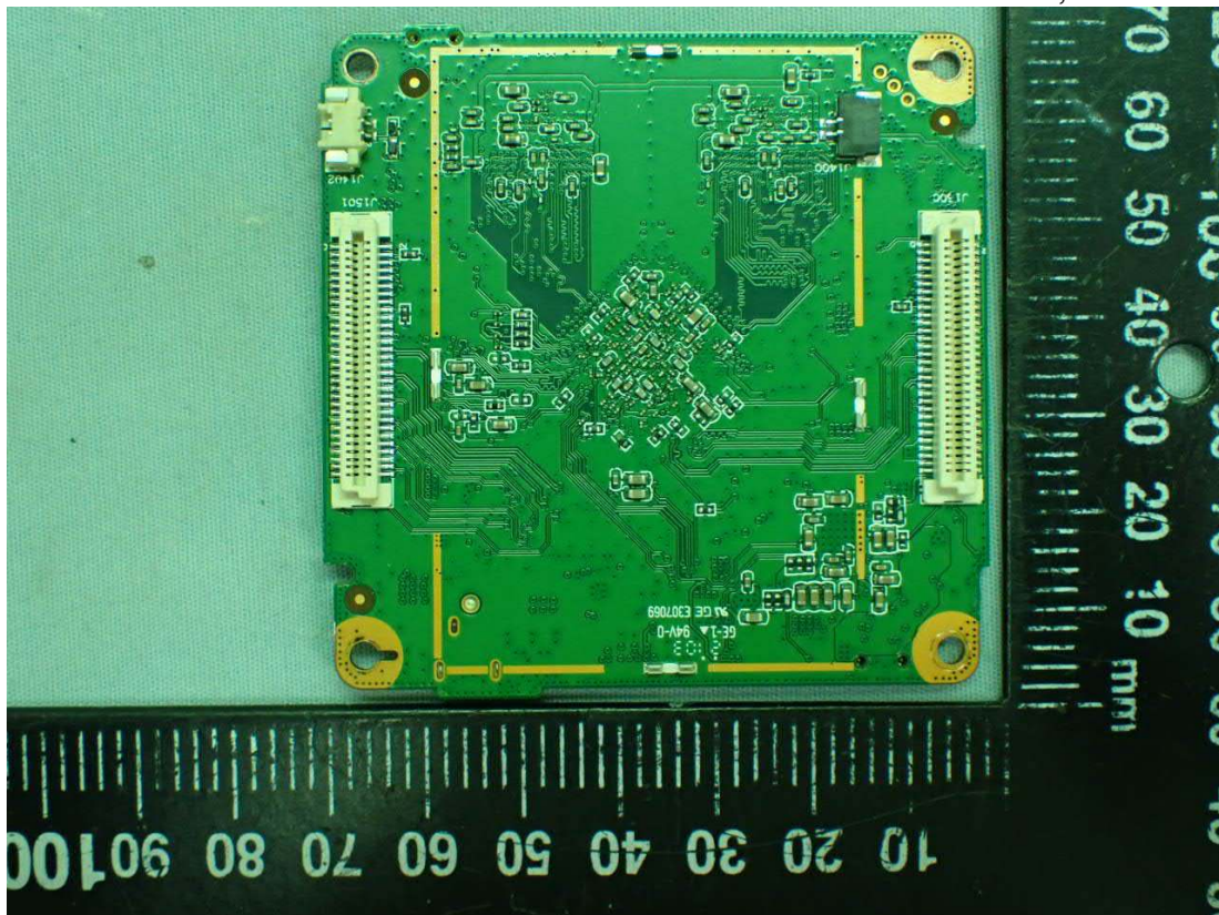
Figure 38 Mother Board, Back View
