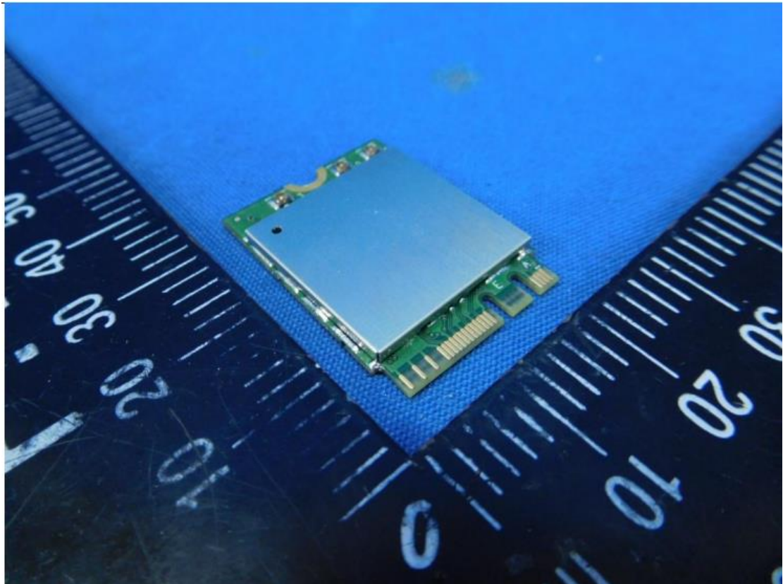
Realtek RTL8822CE
