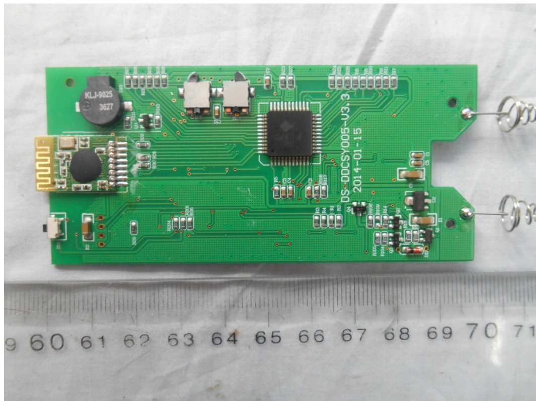
FIGURE 5 REMOTE CONTROLLER (M/N: SFD-Y-14) MAIN BOARD (COMPONENT SIDE)
