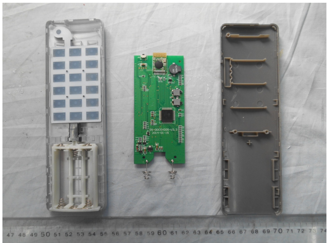
FIGURE 4 REMOTE CONTROLLER (M/N: SFD-Y-14) COVER REMOVED
