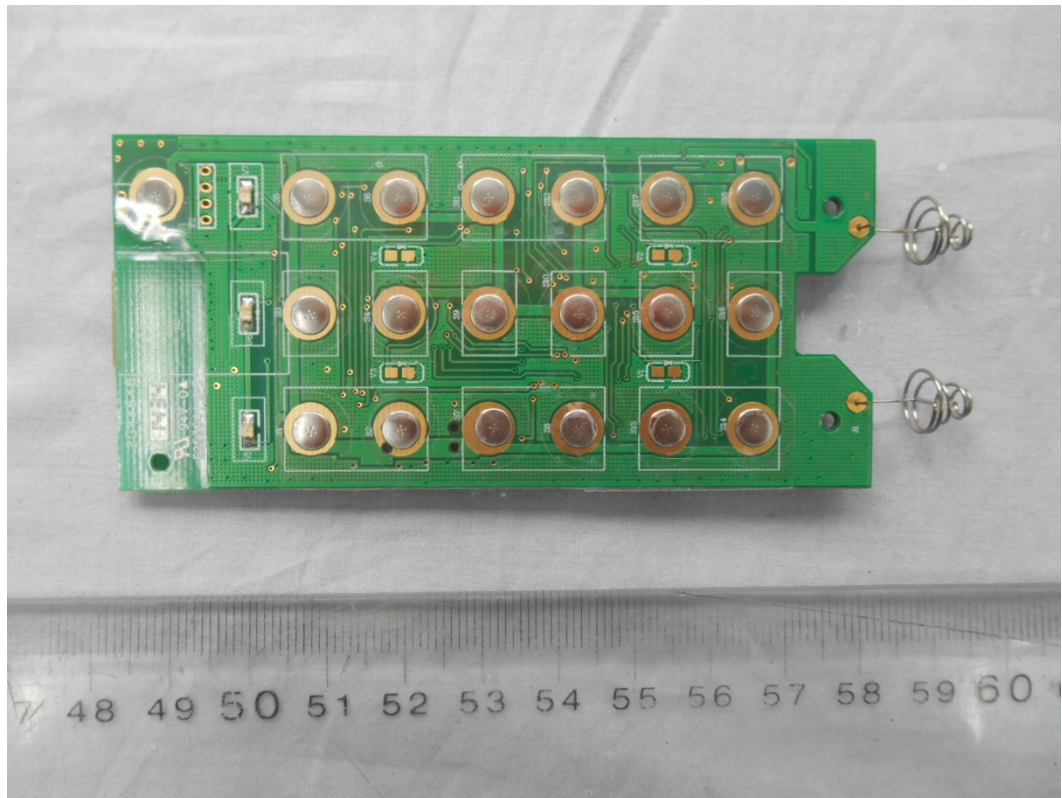
FIGURE 13 REMOTE CONTROLLER (M/N: SFD-Y-18) MAIN BOARD (SOLDERED SIDE)
