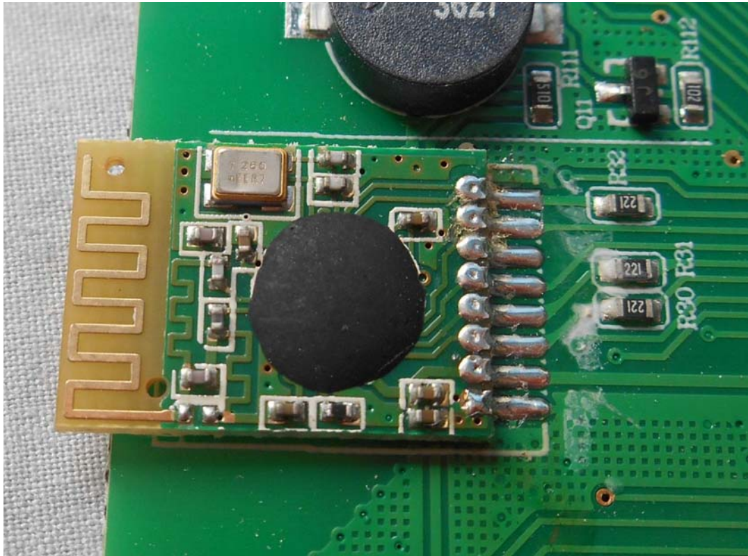
FIGURE 7 REMOTE CONTROLLER (M/N: SFD-Y-14) RF MODULE (FRONT SIDE)
