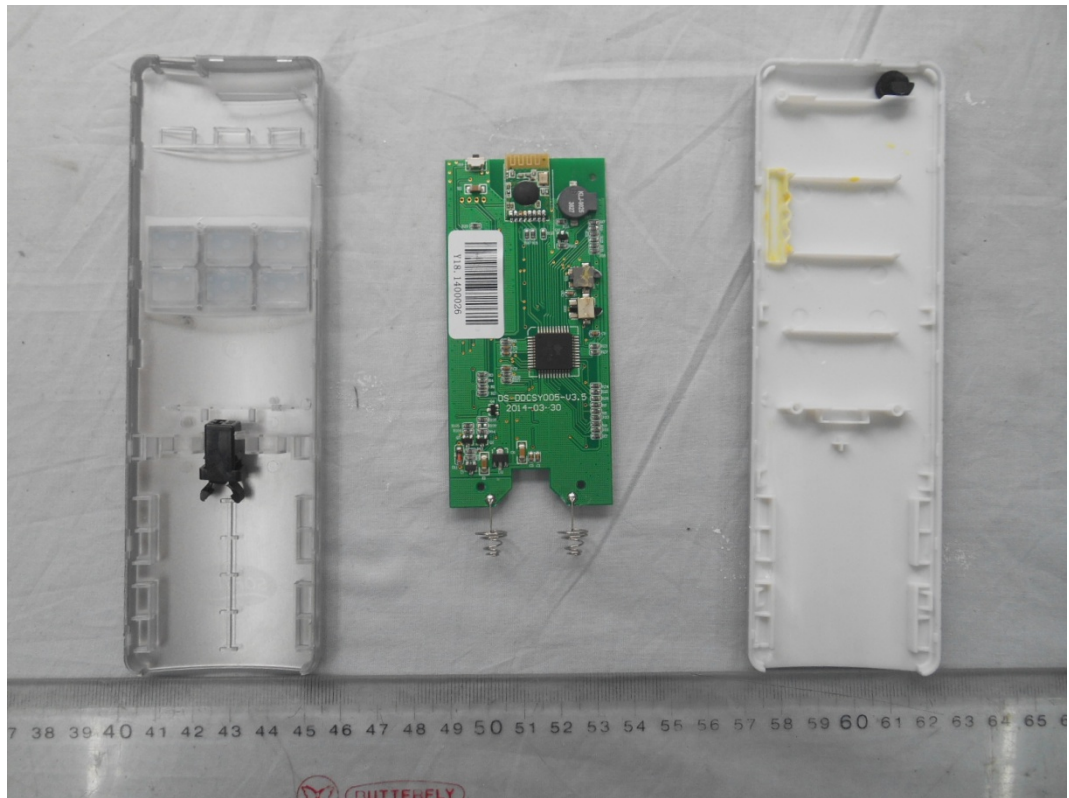
FIGURE 11 REMOTE CONTROLLER (M/N: SFD-Y-18) COVER REMOVED
