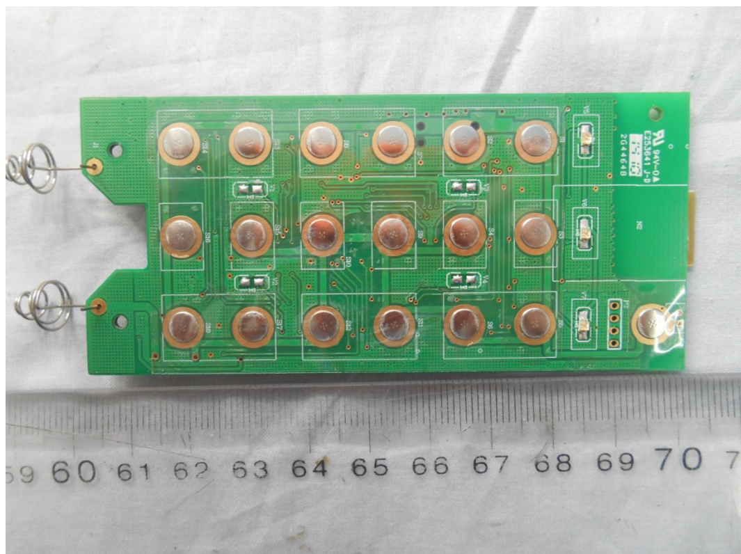
FIGURE 6 REMOTE CONTROLLER (M/N: SFD-Y-14) MAIN BOARD (SOLDERED SIDE)
