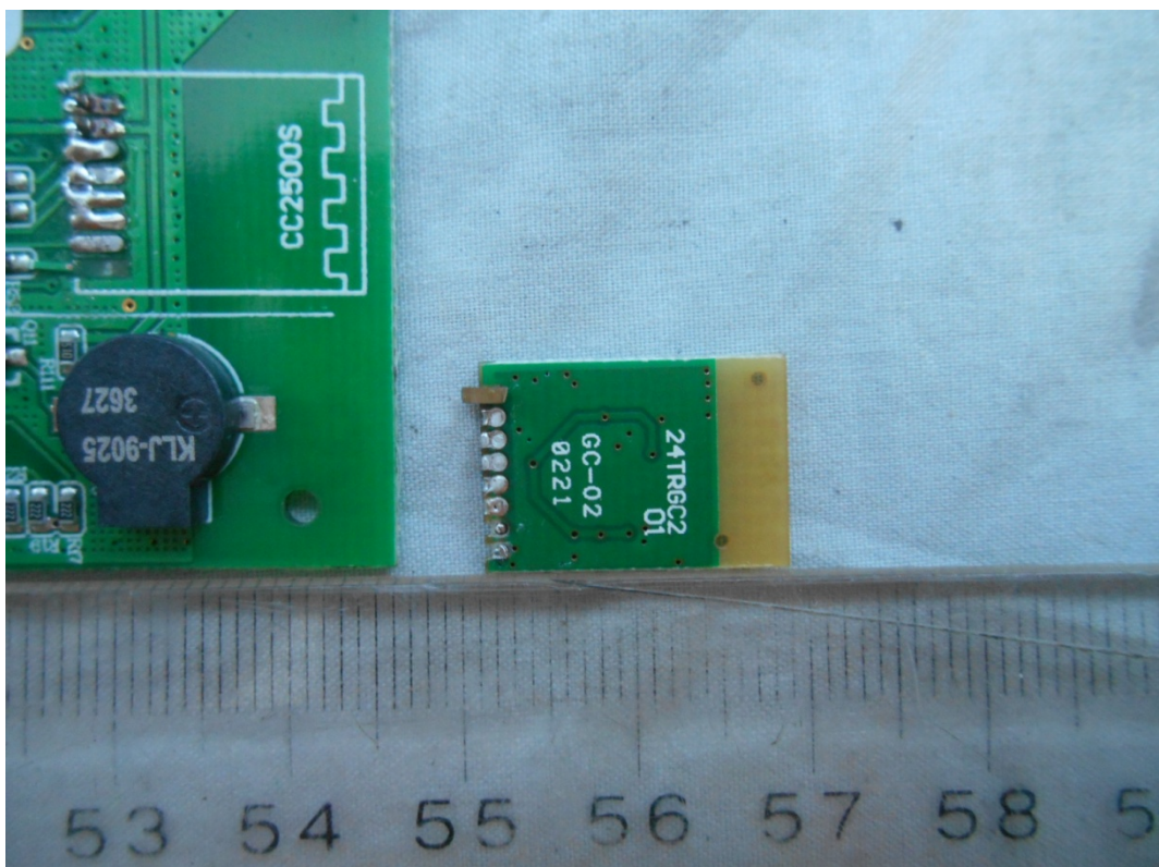
FIGURE 8 REMOTE CONTROLLER (M/N: SFD-Y-14) RF MODULE (BACK SIDE)
