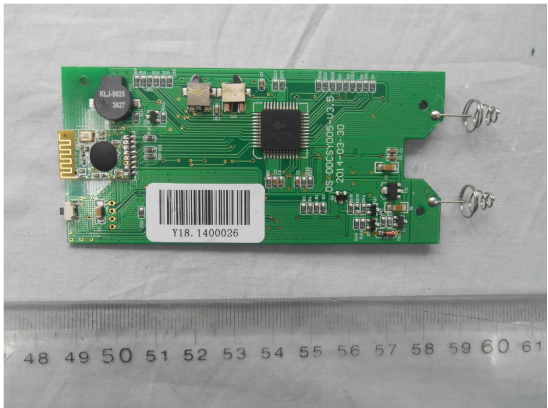
FIGURE 12 REMOTE CONTROLLER (M/N: SFD-Y-18) MAIN BOARD (COMPONENT SIDE)
