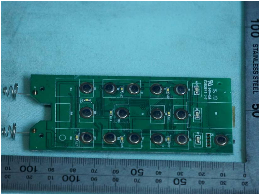
FIGURE 3 REMOTE CONTROLLER (M/N: SFD-Y-13) MAIN BOARD (SOLDERED SIDE)
