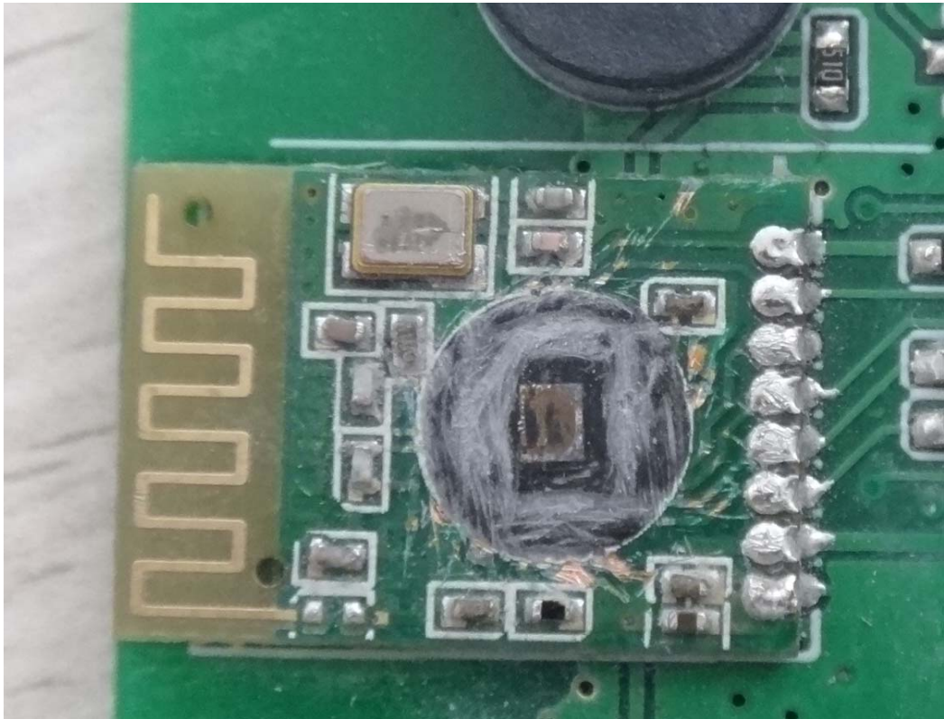
FIGURE 5 REMOTE CONTROLLER (M/N: SFD-Y-13) RF MODULE (CHIP RUBBER REMOVED)
