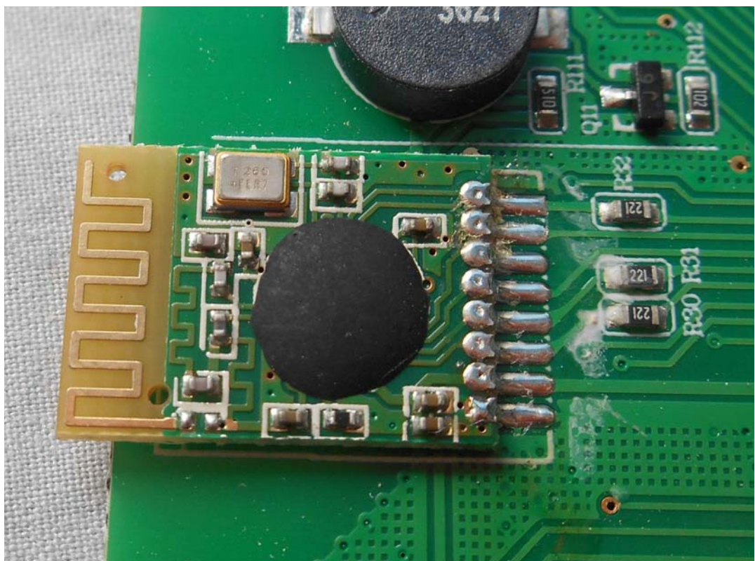
FIGURE 4 REMOTE CONTROLLER (M/N: SFD-Y-13) RF MODULE (FRONT SIDE)
