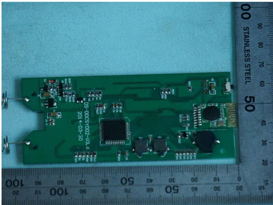
FIGURE 2 REMOTE CONTROLLER (M/N: SFD-Y-13) MAIN BOARD (COMPONENT SIDE)
