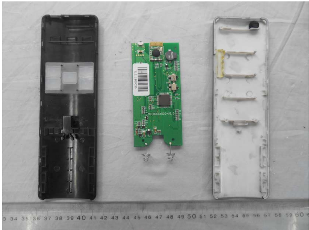
FIGURE 7 REMOTE CONTROLLER (M/N: SFD-Y-15) COVER REMOVED
