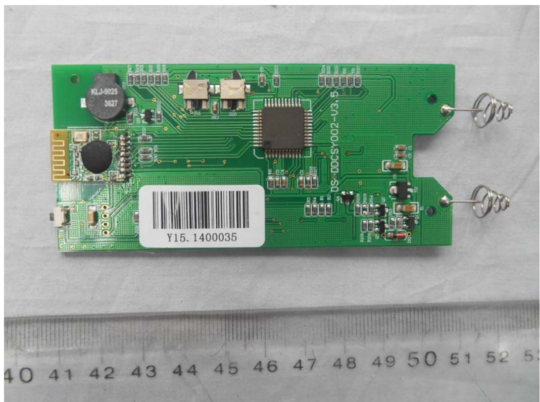
FIGURE 8 REMOTE CONTROLLER (M/N: SFD-Y-15) MAIN BOARD (COMPONENT SIDE)
