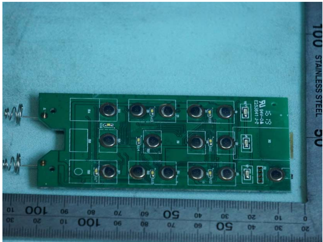
FIGURE 9 REMOTE CONTROLLER (M/N: SFD-Y-15) MAIN BOARD (SOLDERED SIDE)
