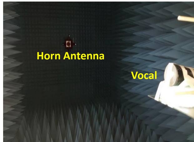
Measurement Setup
