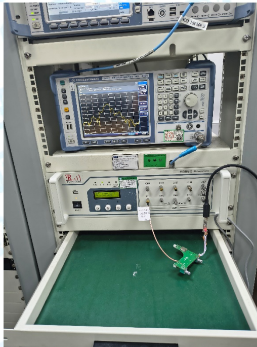
Photo of Setup for Conducted Measurement
