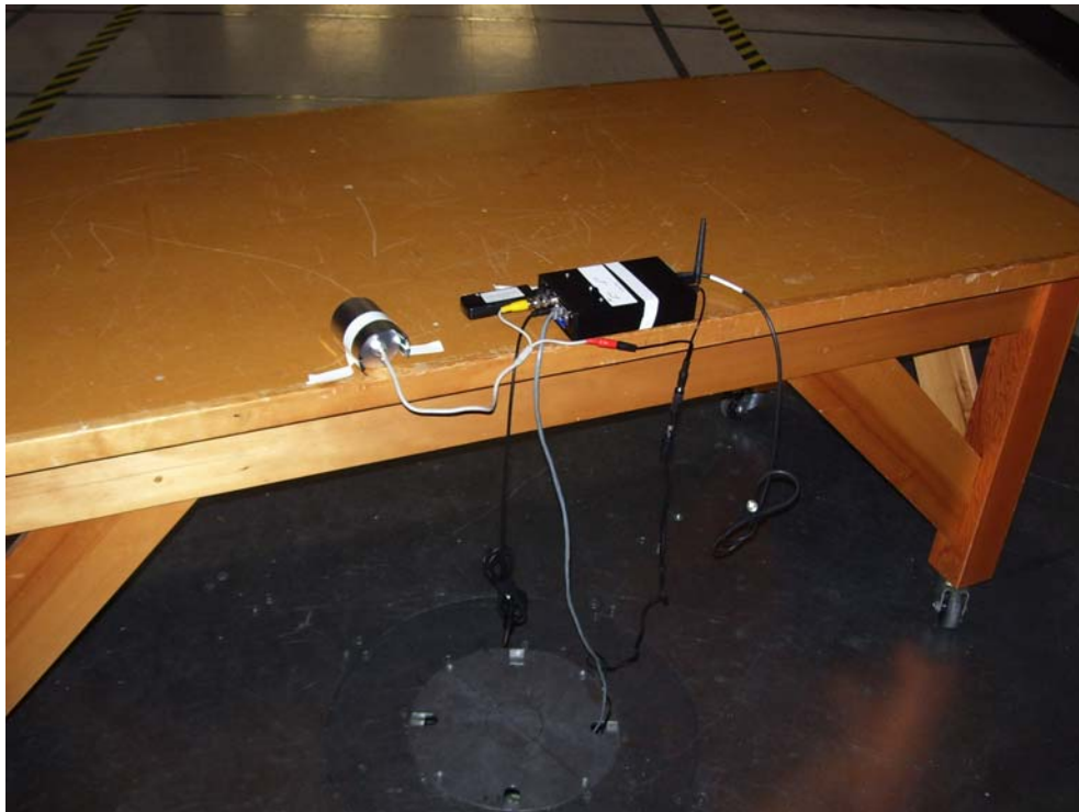
Figure 2 - Radiated Emissions Test Setup
