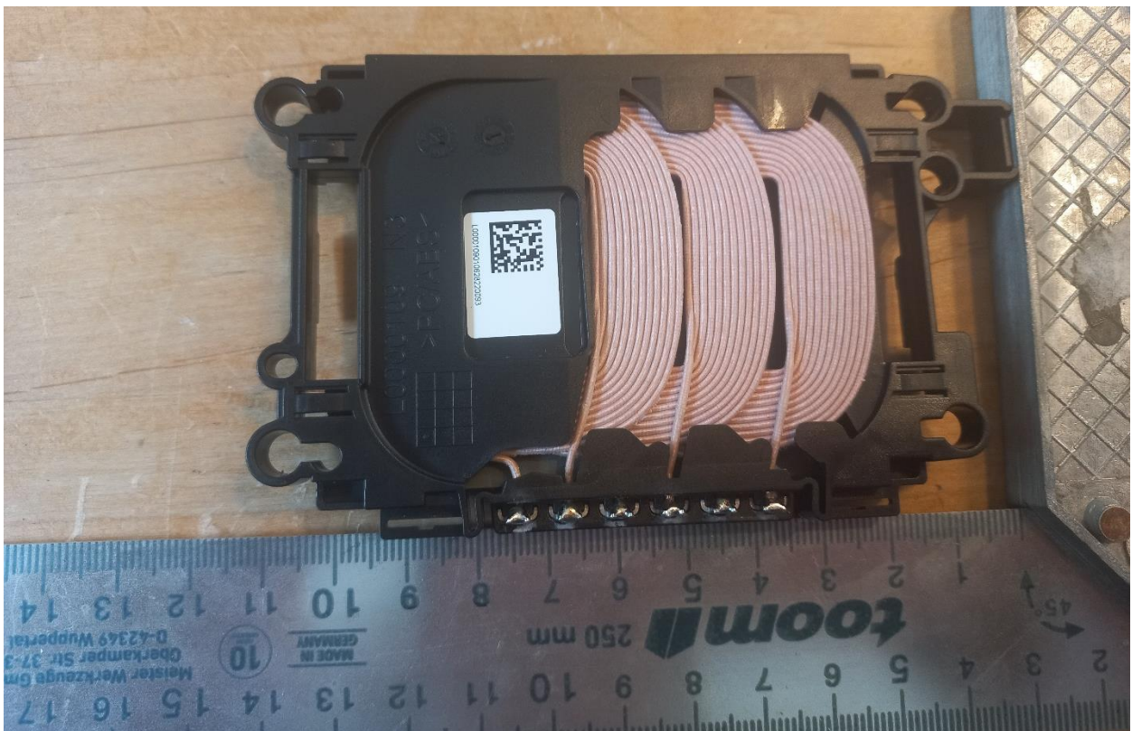
Coil board
