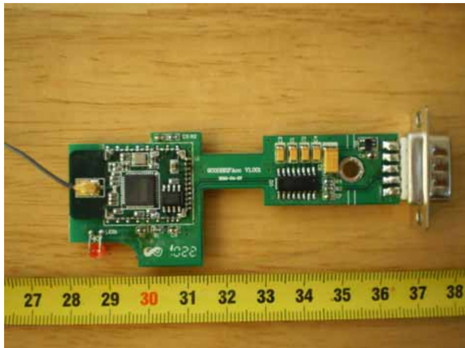
Figure 3 Main Board unshield View
