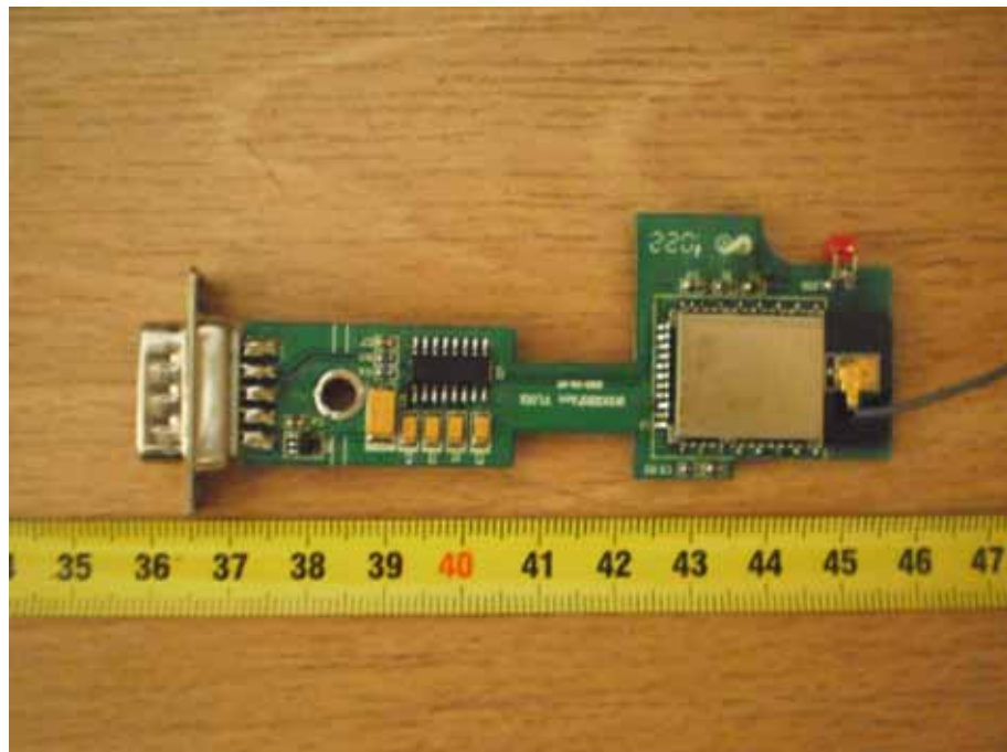
Figure 2 Main Board Top Components View
