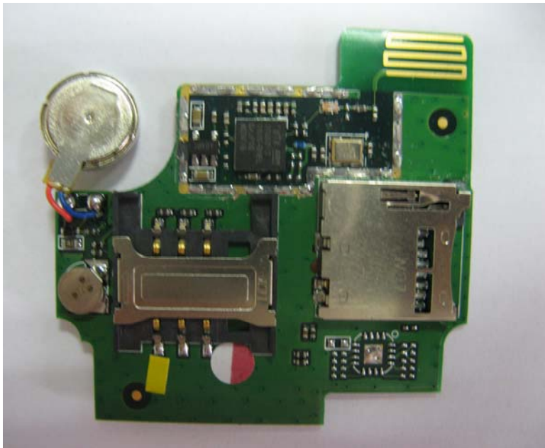
Picture 3: The sample with the shielding cover removed
