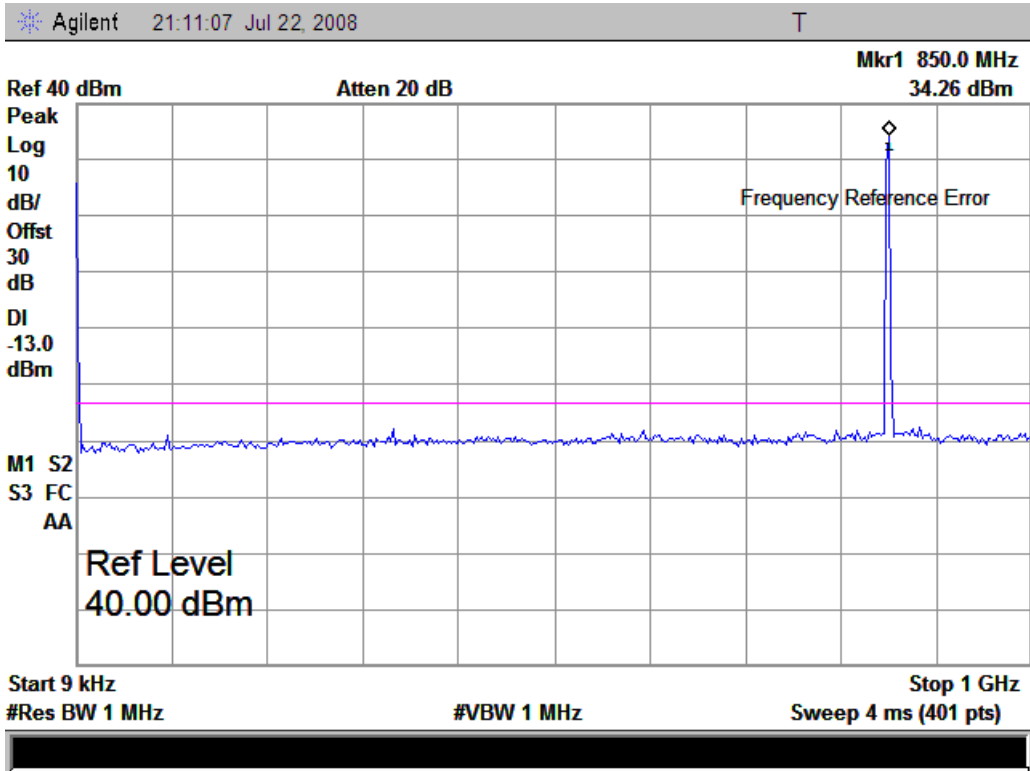
(9 KHz-1 GHz)
