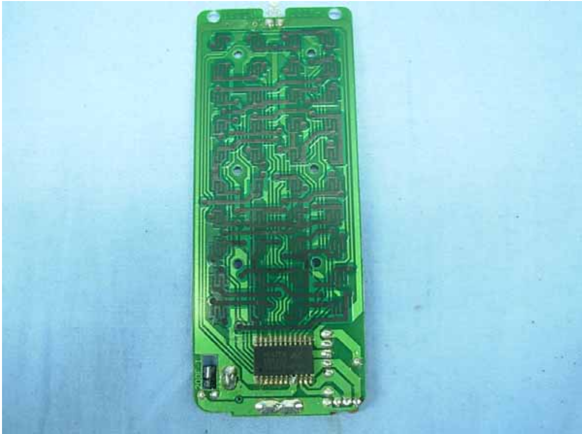
Figure 54 Internal (Back View)
