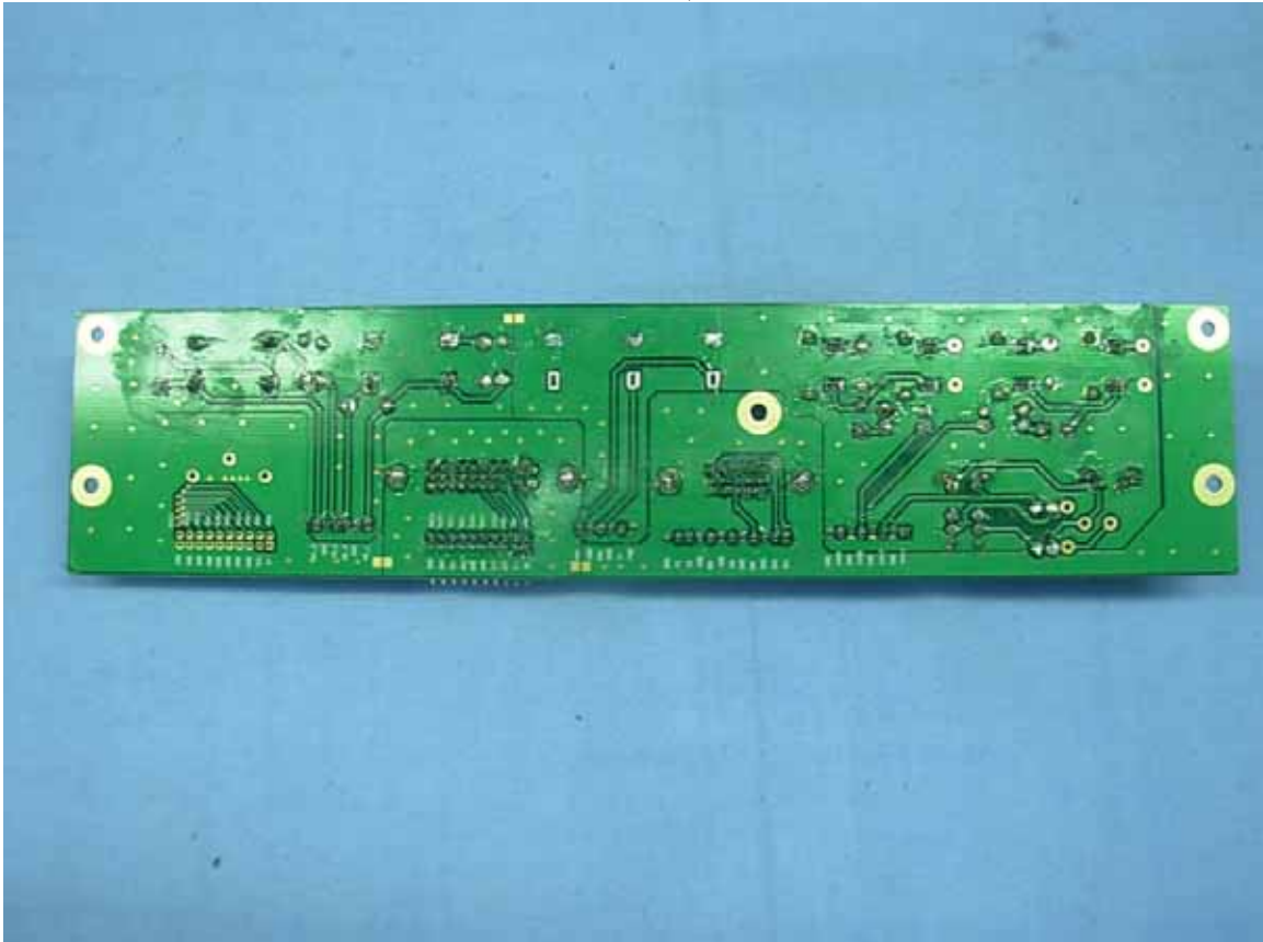
Figure 22 I/O Ports Board (Solder Side, for KA42U2CN& KB42U2CN))
