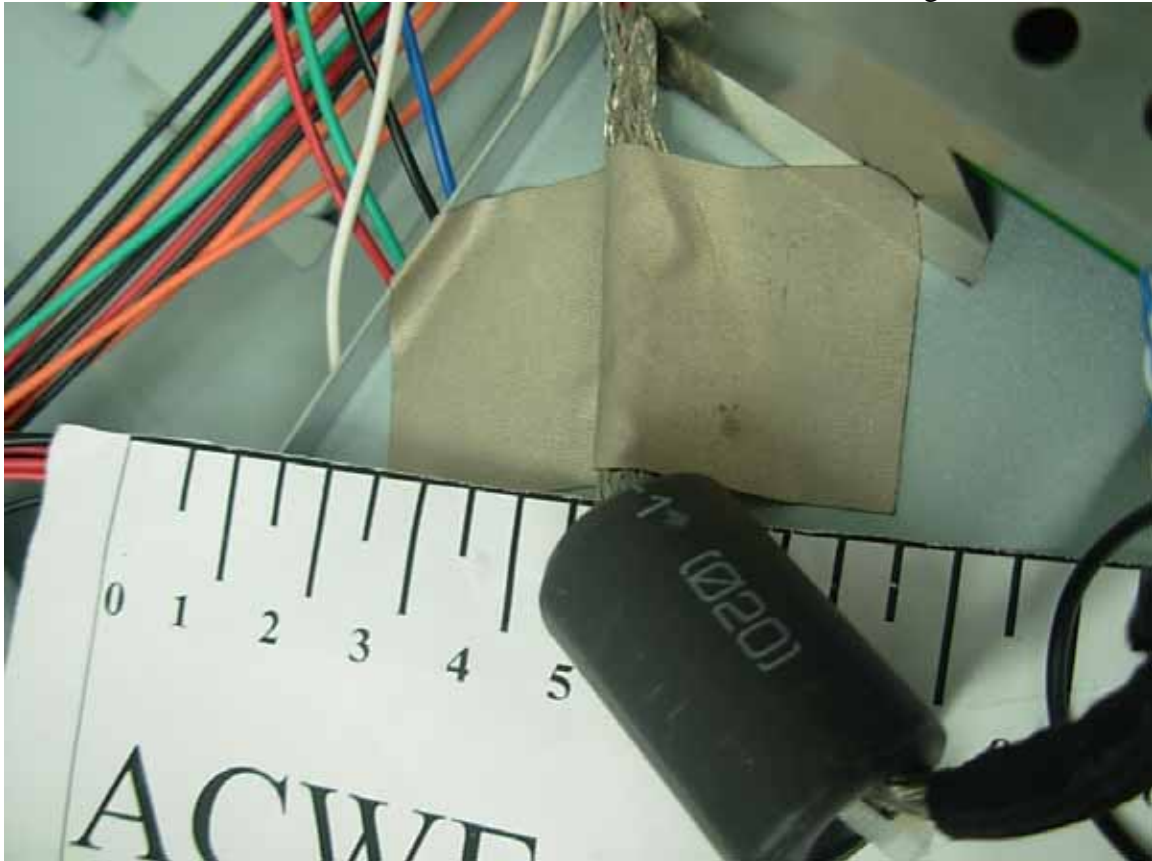
Figure 38 Conducting Copper Foil
