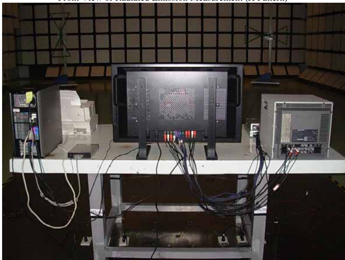
Back View of Radiated Emission Measurement (H Pattern)
