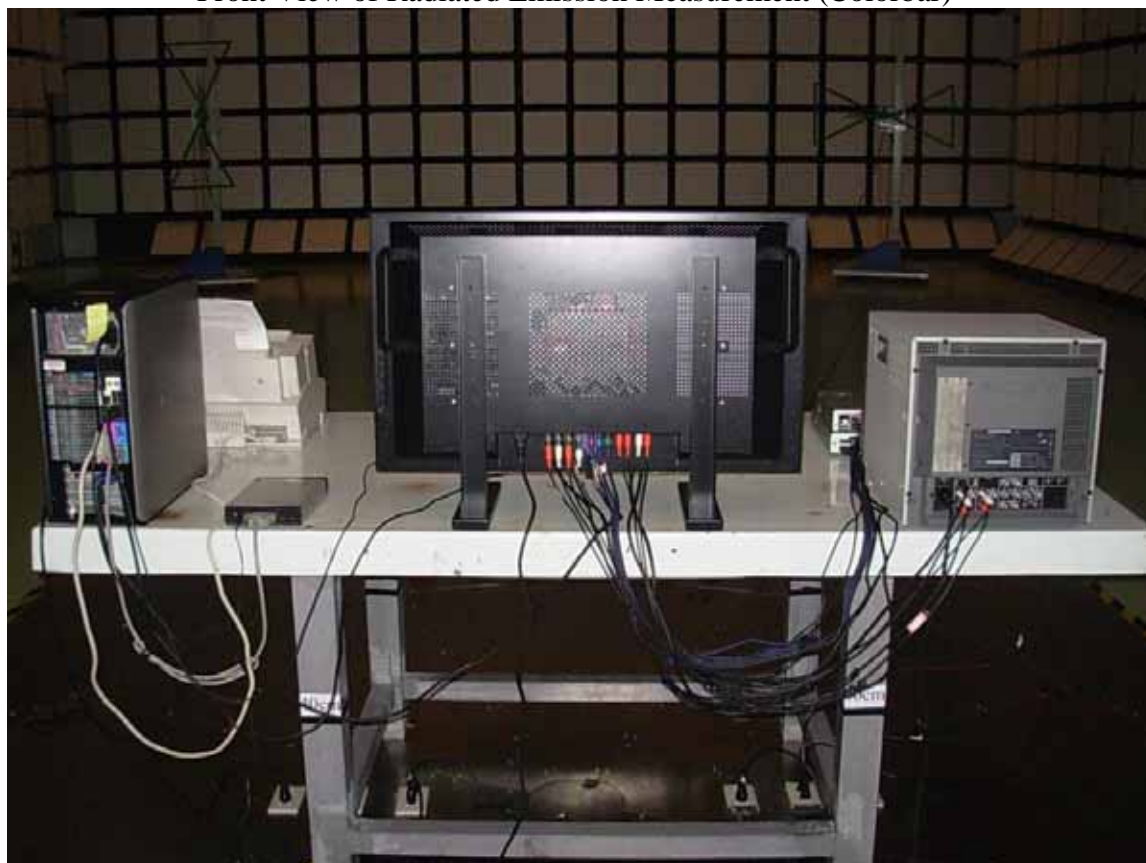
Back View of Radiated Emission Measurement (Colorbar)
