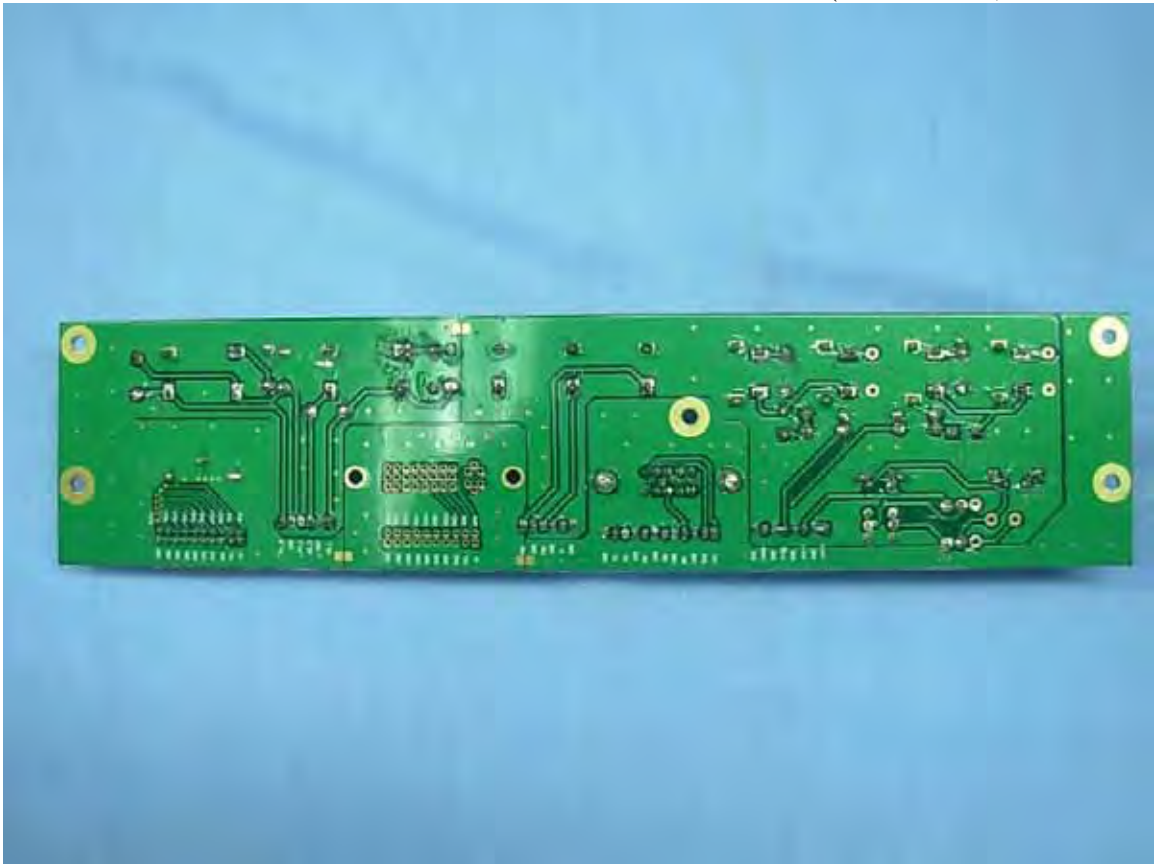
Figure 20 I/O Ports Board (Solder Side, for KA32T2CN)
