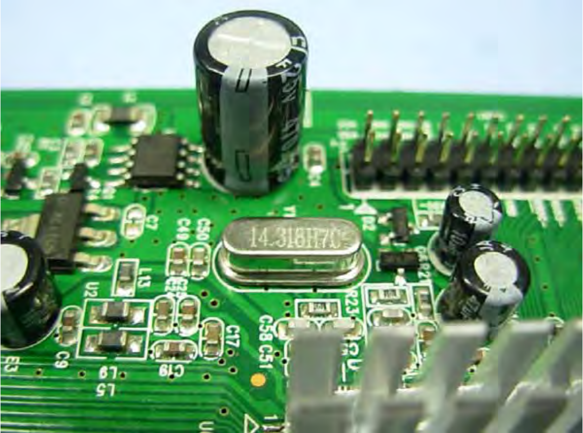
Figure 12 Crystal Oscillator
