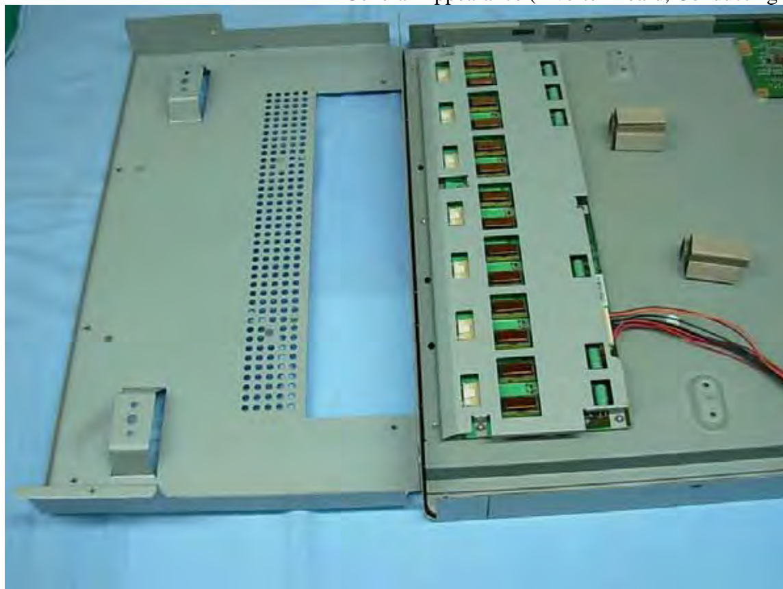
Figure 44 General Appearance (Inverter Board, Conducting Sponge)
