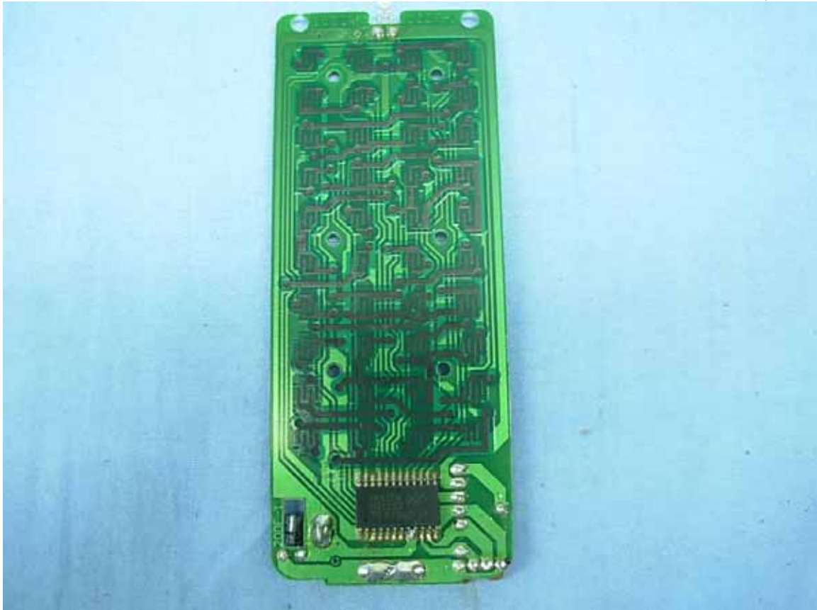
Figure 48 Internal View (Back View)
