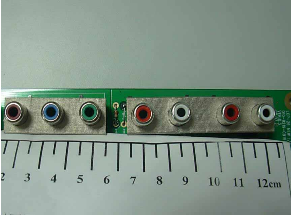
Figure 28 I/O Port Board (Conducting Sponge)
