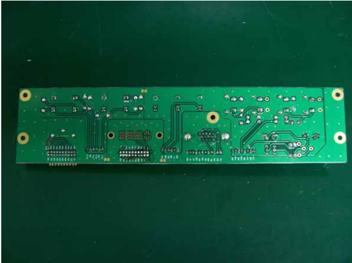
Figure 28 I/O Port Board (Conducting Sponge)
