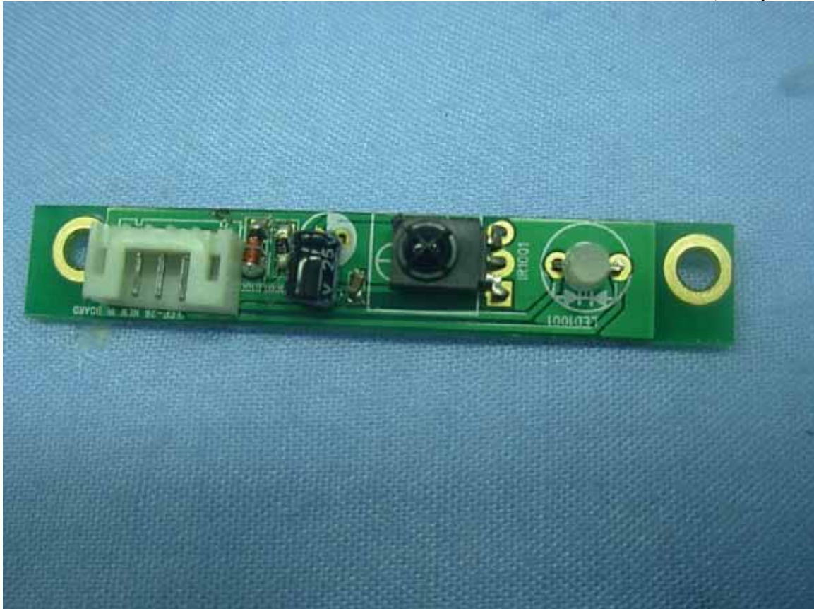
Figure 38 LED Board (Component Side)
