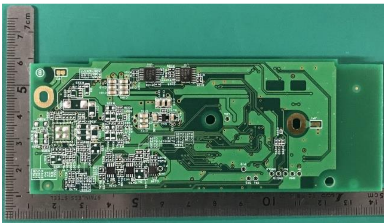
Cable Relay Board (Back side)
