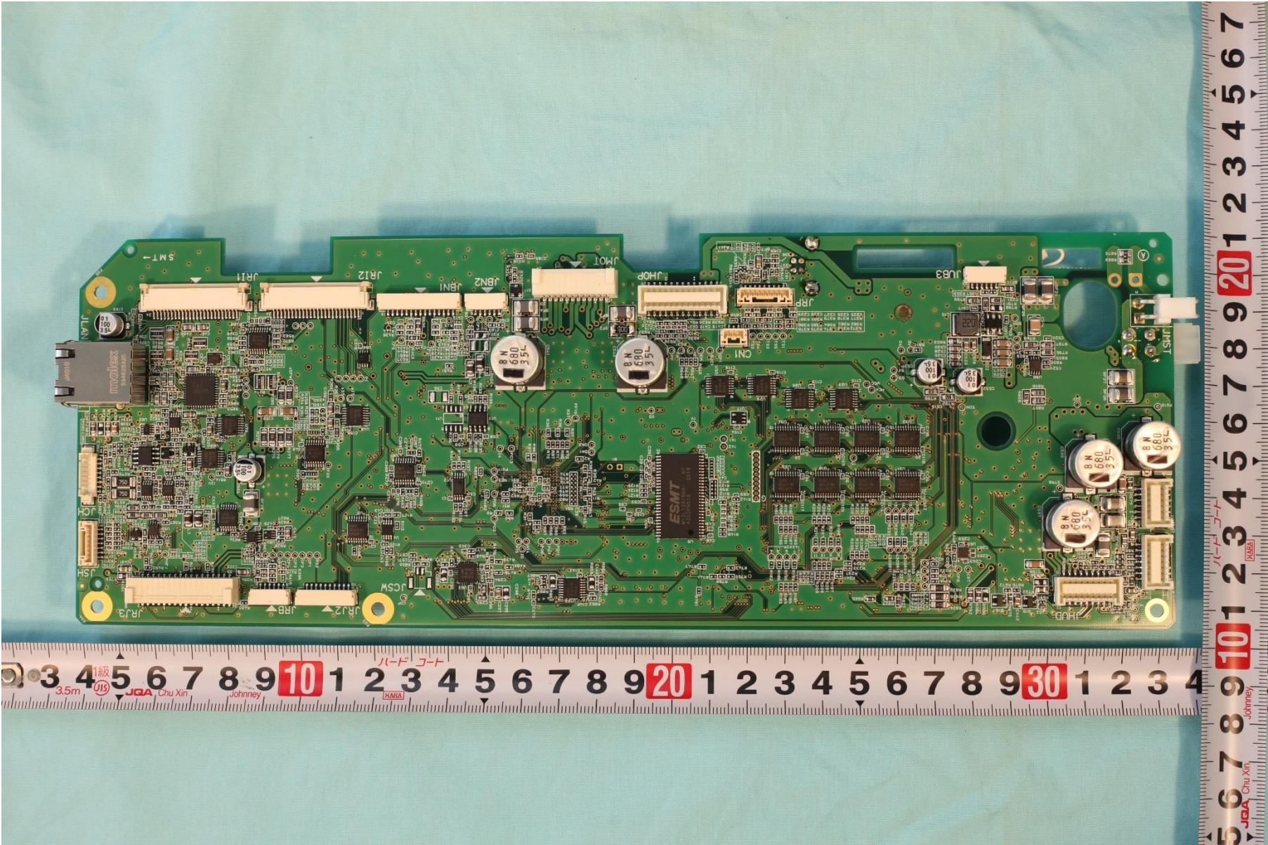
Main Circuit board (Back side)
