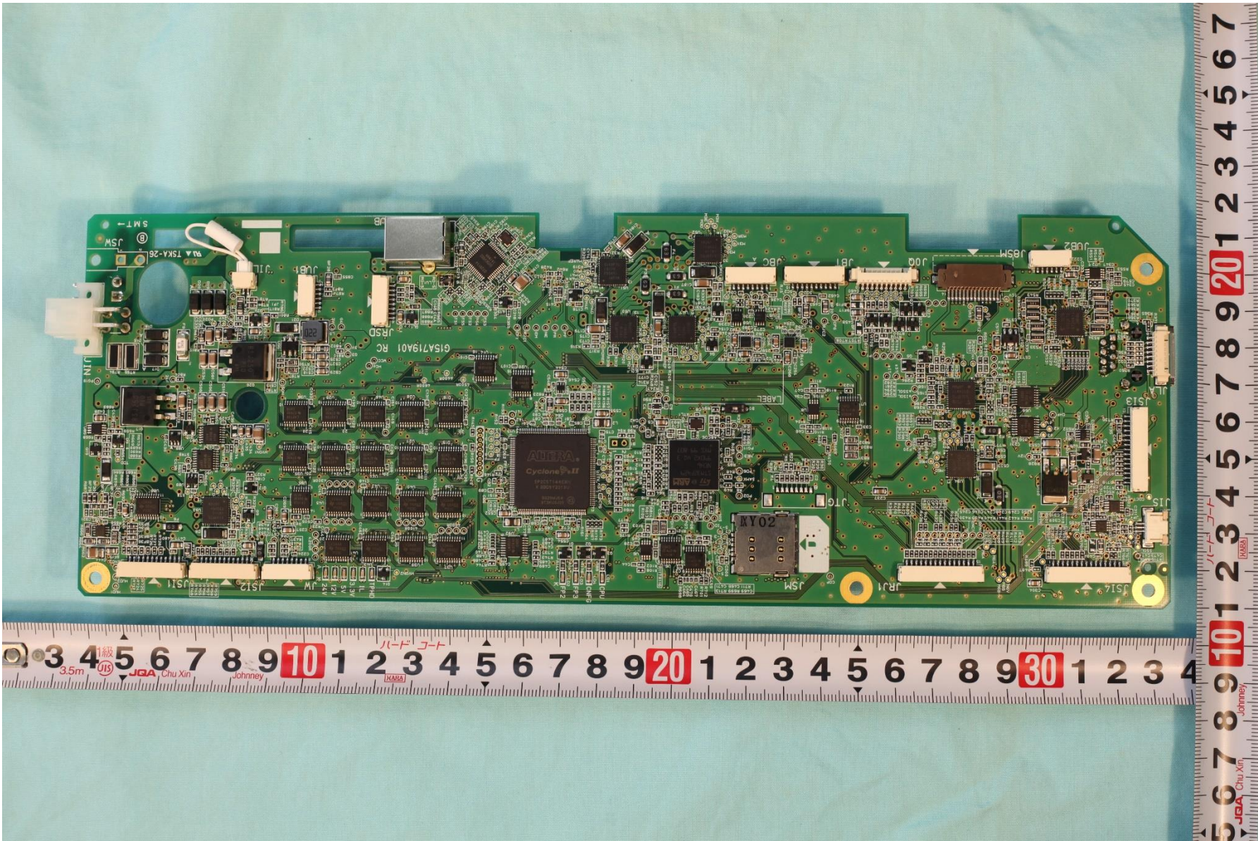
Main Circuit board (Front side)
