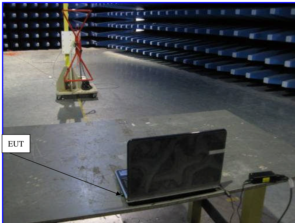
Radiated Emission Setup Rear View below 1GHz
