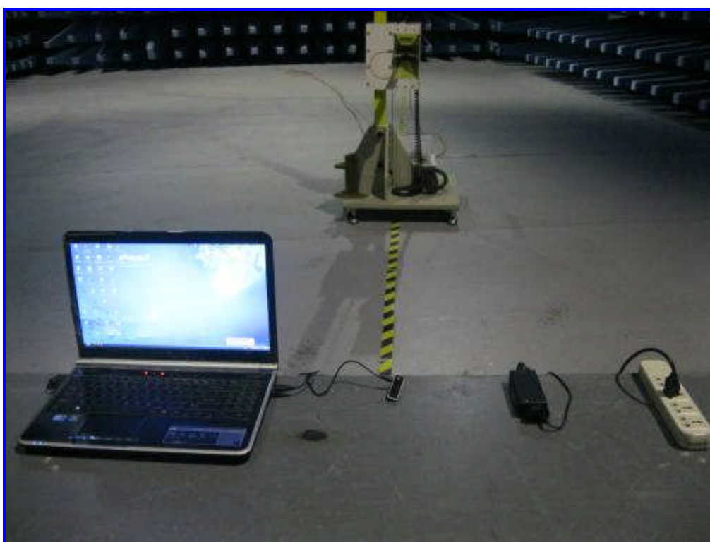
Front View of Radiated Emissions Test Setup above 1GHz
