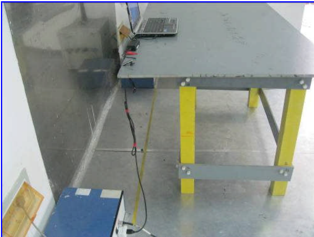
Rear View of Conducted Emissions Test Setup
