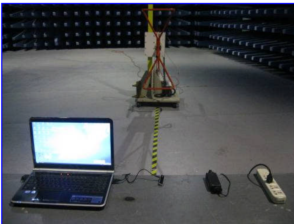
Front View of Radiated Emissions Test Setup below 1GHz
