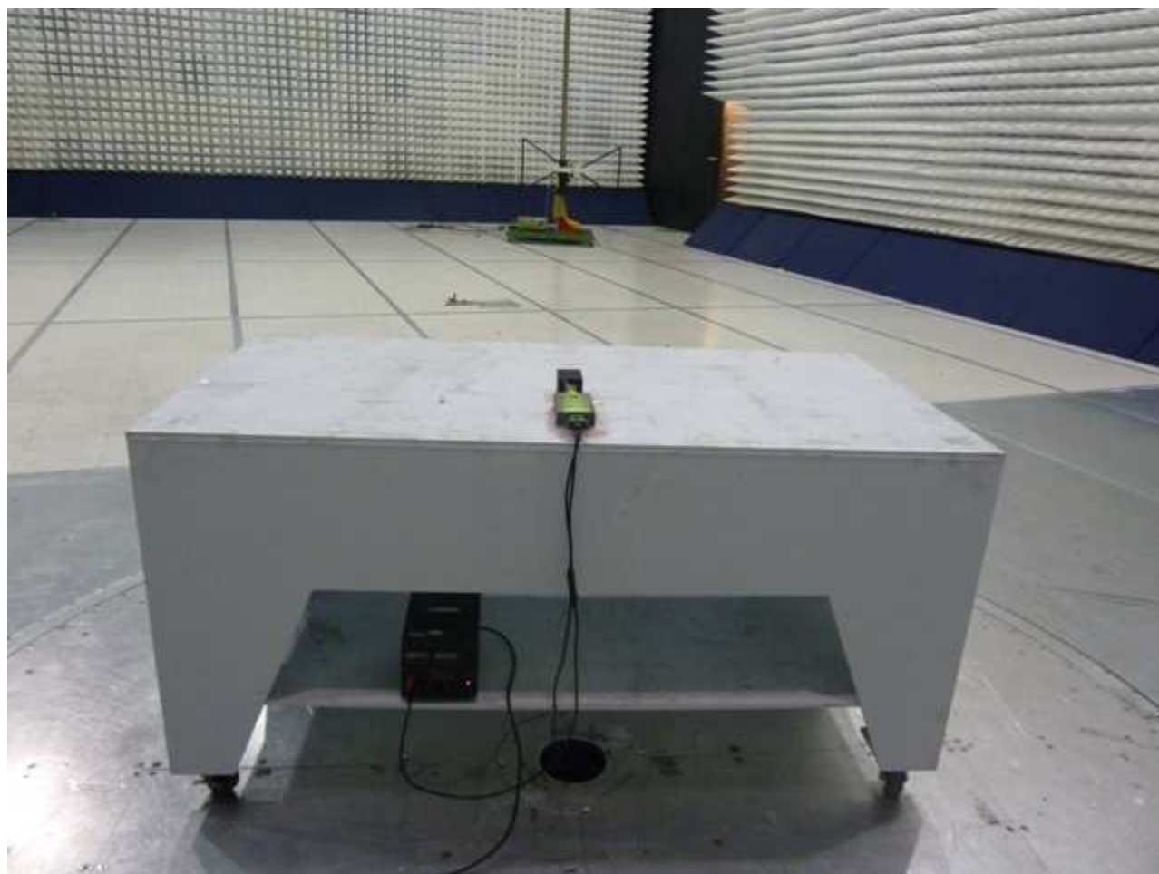
Radiated Emissions at 10 m (Transmitter spurious)
