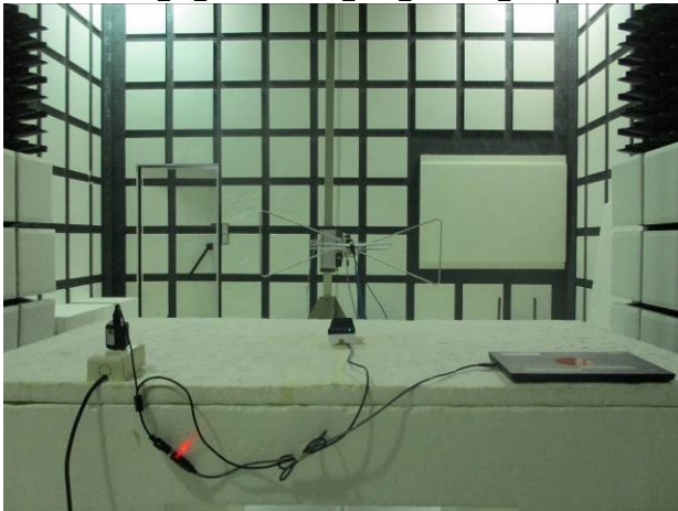
Part_15_225+RSS 210_NFC_Radiated_Setup
