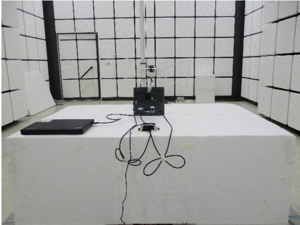
Part_15_407+RSS-247_5G_Radiated_Setup
