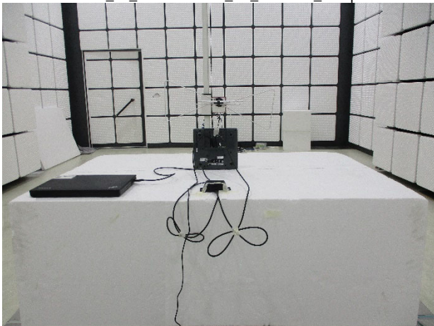
Part_15_247+RSS-247_BT_Radiated_Setup
