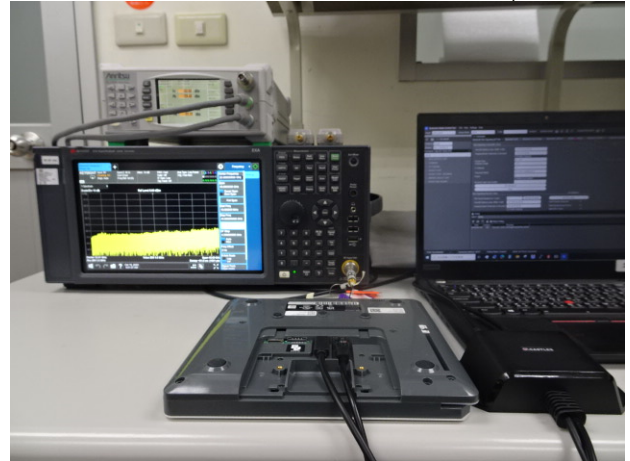
Part_15_407+RSS-247_5G_Radiated_Setup
