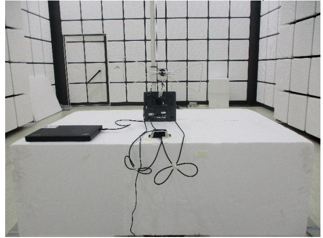
Part_15_247+RSS-247_2.4G_Radiated_Setup
