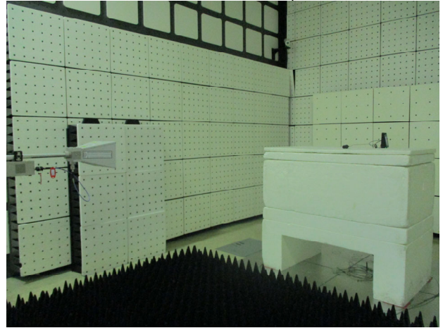
2G_3G_Radiated_Setup
