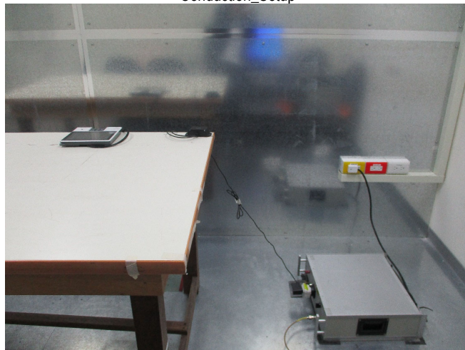
Conduction_Setup
