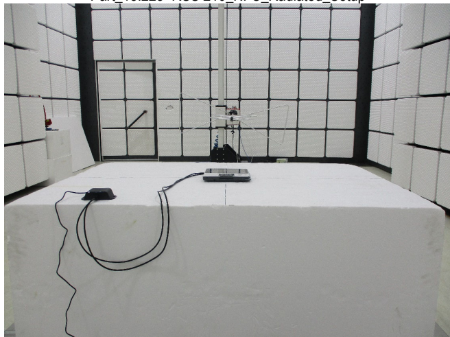
Part_15.225+RSS 210_NFC_Radiated_Setup
