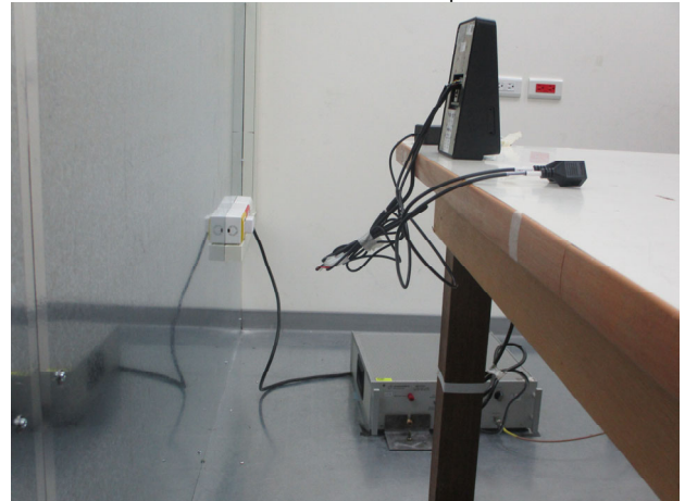
NFC_Conduction_Setup
