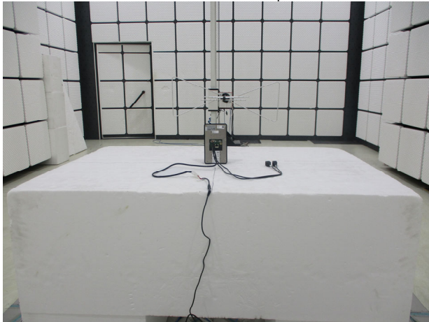
NFC_Radiated_Setup
