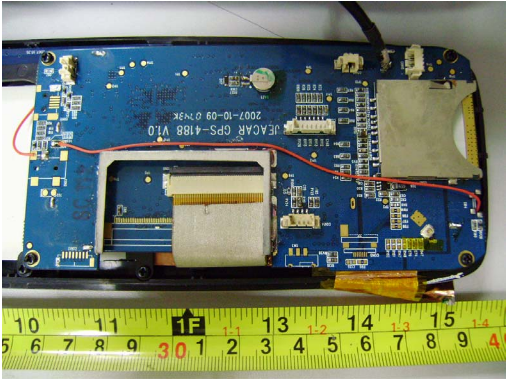
Solder Board-Component View 4
