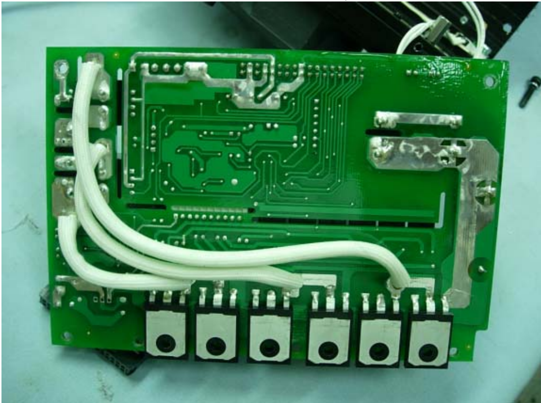
Figure 16 Internal View (Servo/Device Board, Back View)
