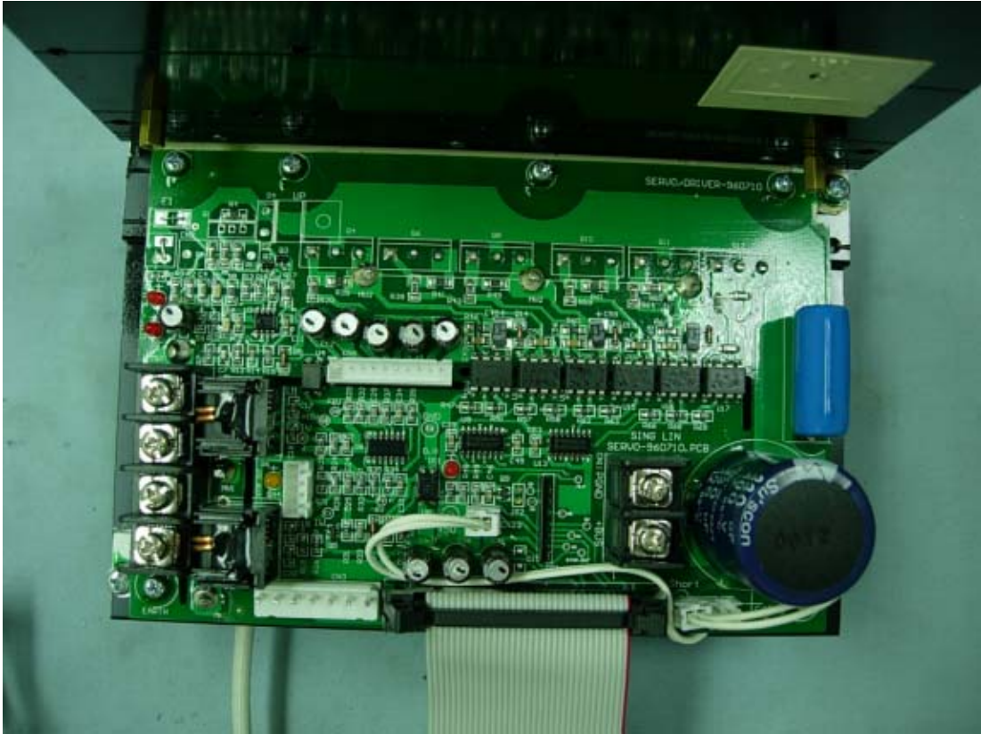
Figure 15 Internal View (Servo/Device Board, Front View)
