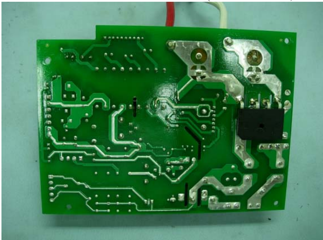
Figure 14 Internal View (Servo/Power Board, Back View)
