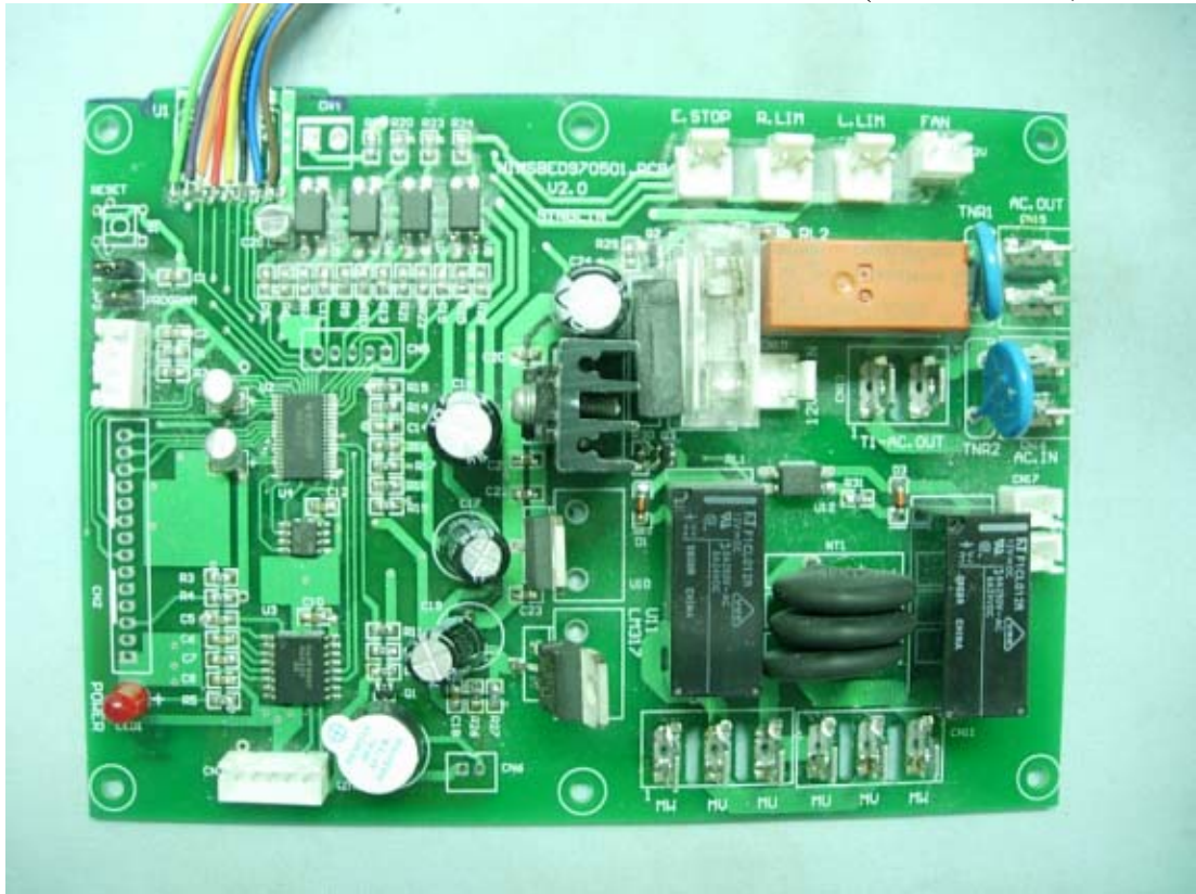
Figure 5 Internal View (Power Board, Front View)
