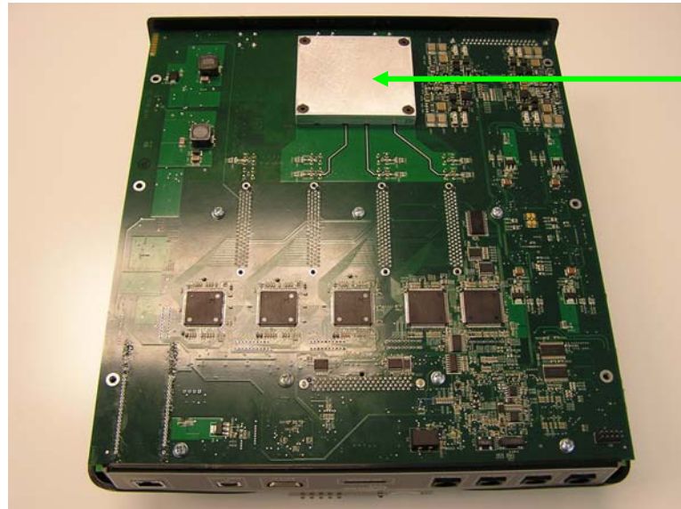
Enclosure Bottom Removed; Bottom of Main Board
