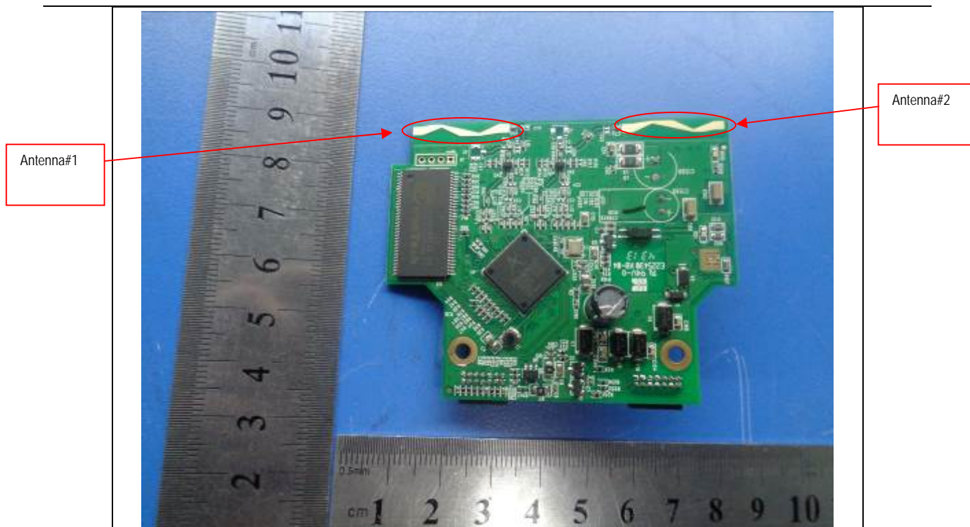
EUT – PCBA 1 Rear View
