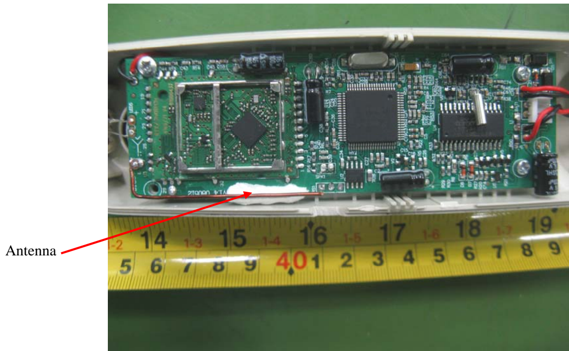
EUT- Main Board Components Top View
