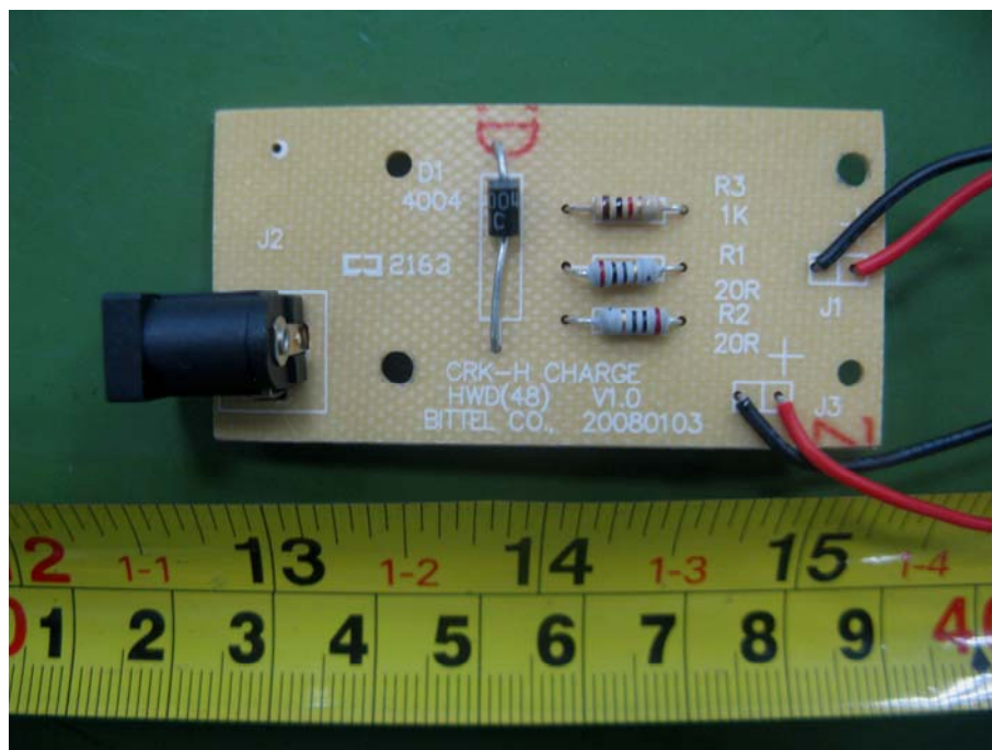
Charger - PCB Components Top View
