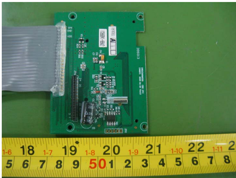
EUT – Display Control Board Components View
