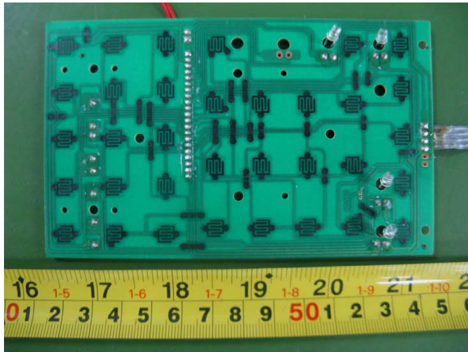
EUT – Button Control Board Circuit View
