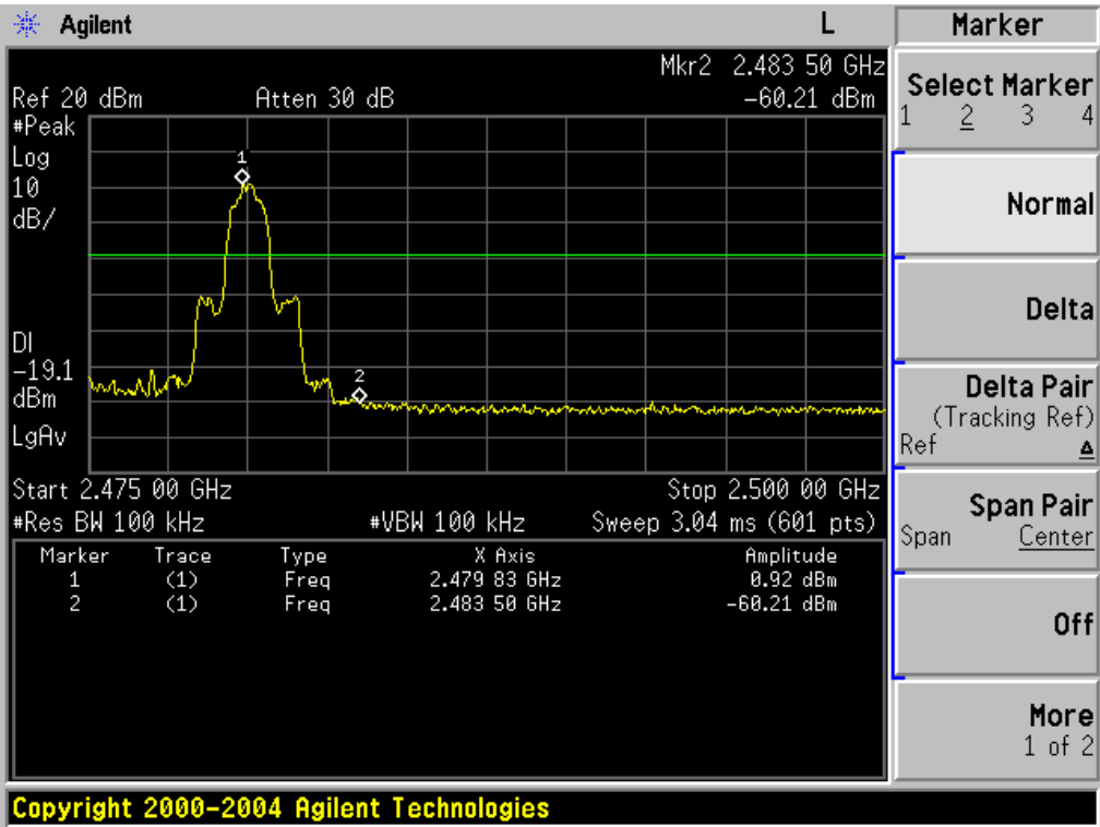
EDR mode(8DPSK): Band Edge-Right Side
