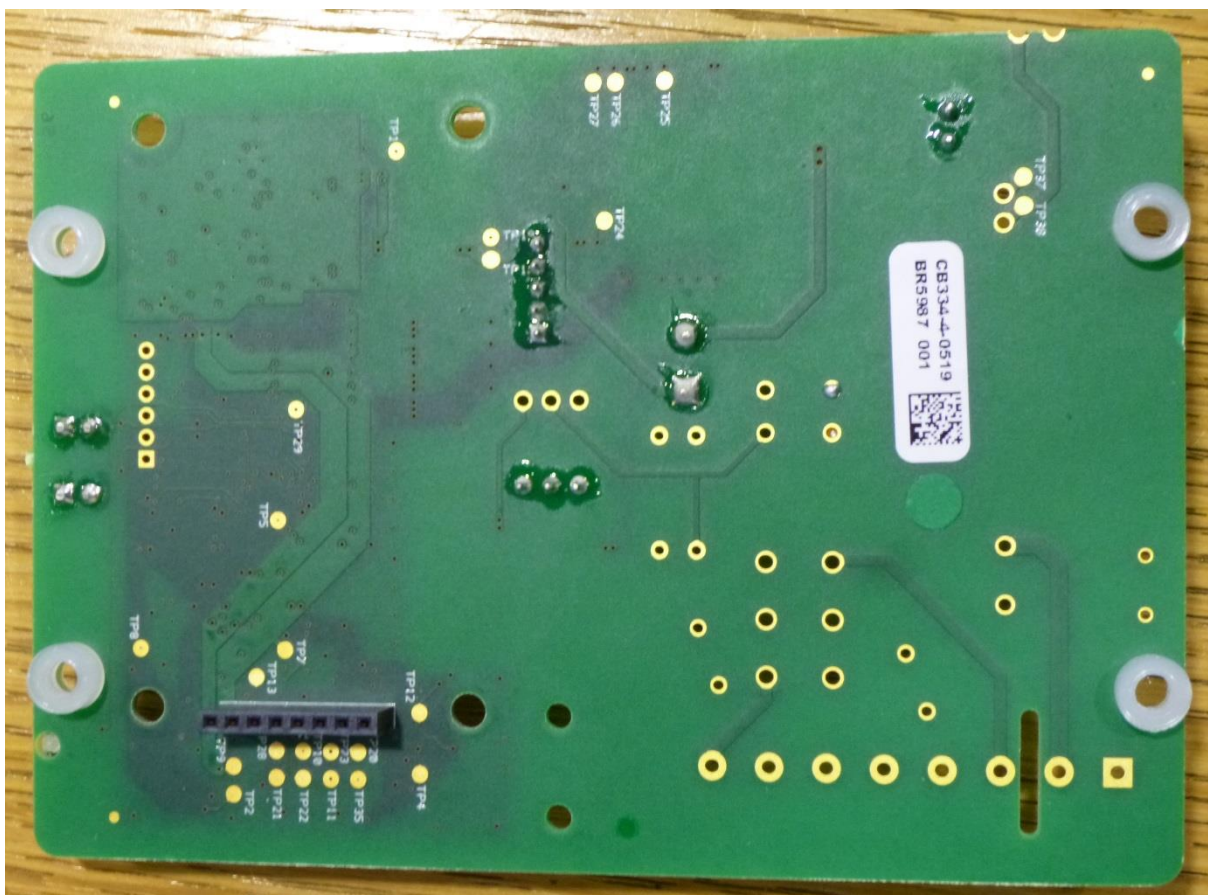
Figure 2 CB-334 Bottom side (module removed)
