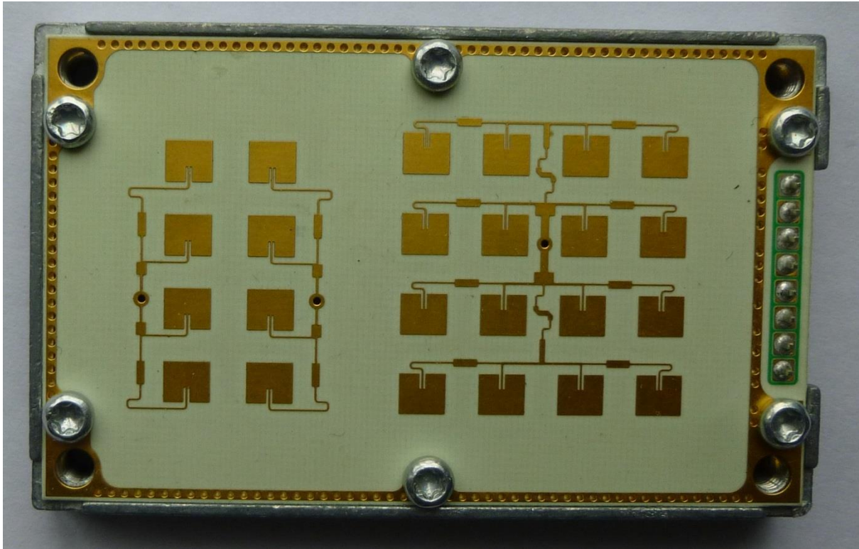
Figure 5MC-135 Front View (antenna side)
