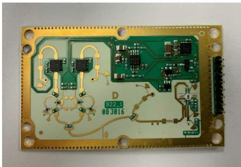
Figure 7 MC-135 PCB Component side
