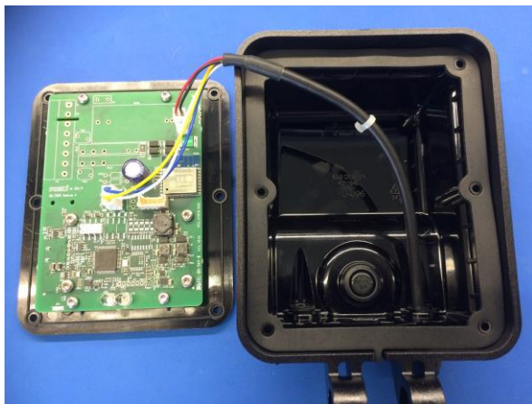
Figure 9 326 -5xx internal assembly
