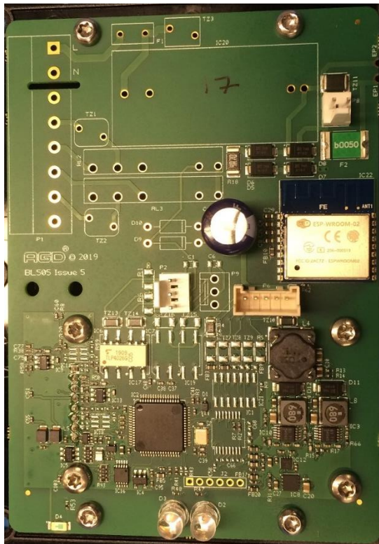
Figure 1 CB-334 top view (low voltage)
