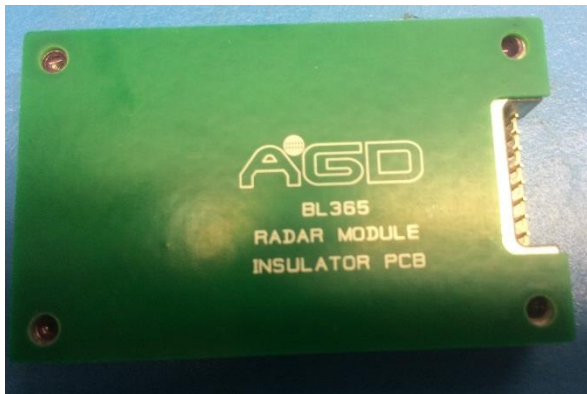
Figure 8 MC-135 with Insulator Fitted
