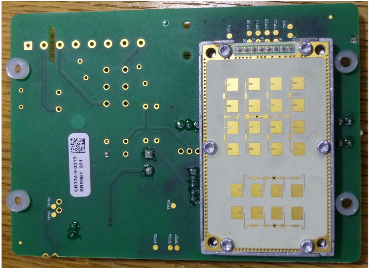
Figure 3 CB-334 Bottom side
