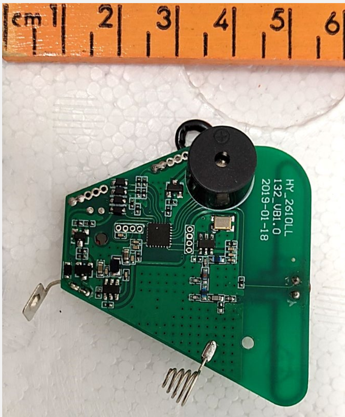
PCB FRONT
