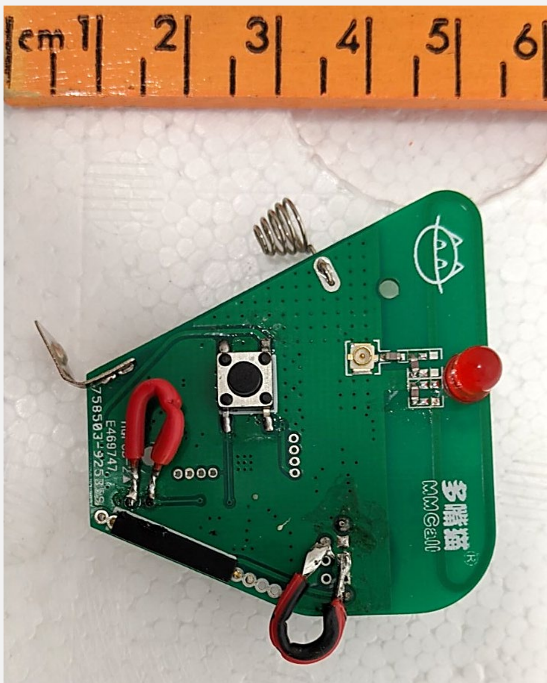
PCB BACK
