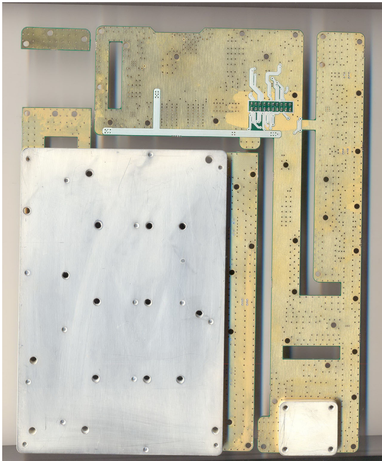
<Photograph 3: (AMP) REAR view>
