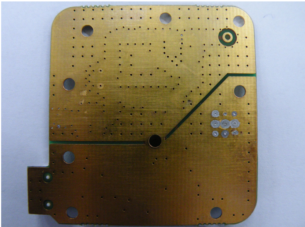
&lt;Photograph 16: (LNA) REAR view&gt;
