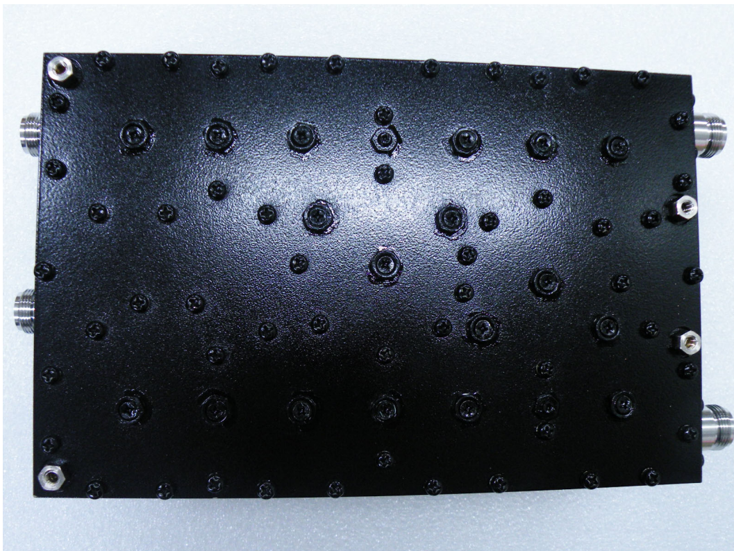
<Photograph 13: (Duplexer) FRONT view>
