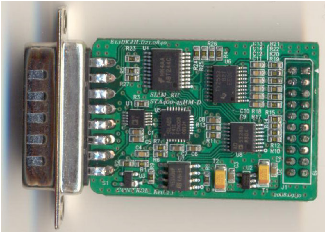
<Photograph 4: (AMP - control board) FRONT view>
