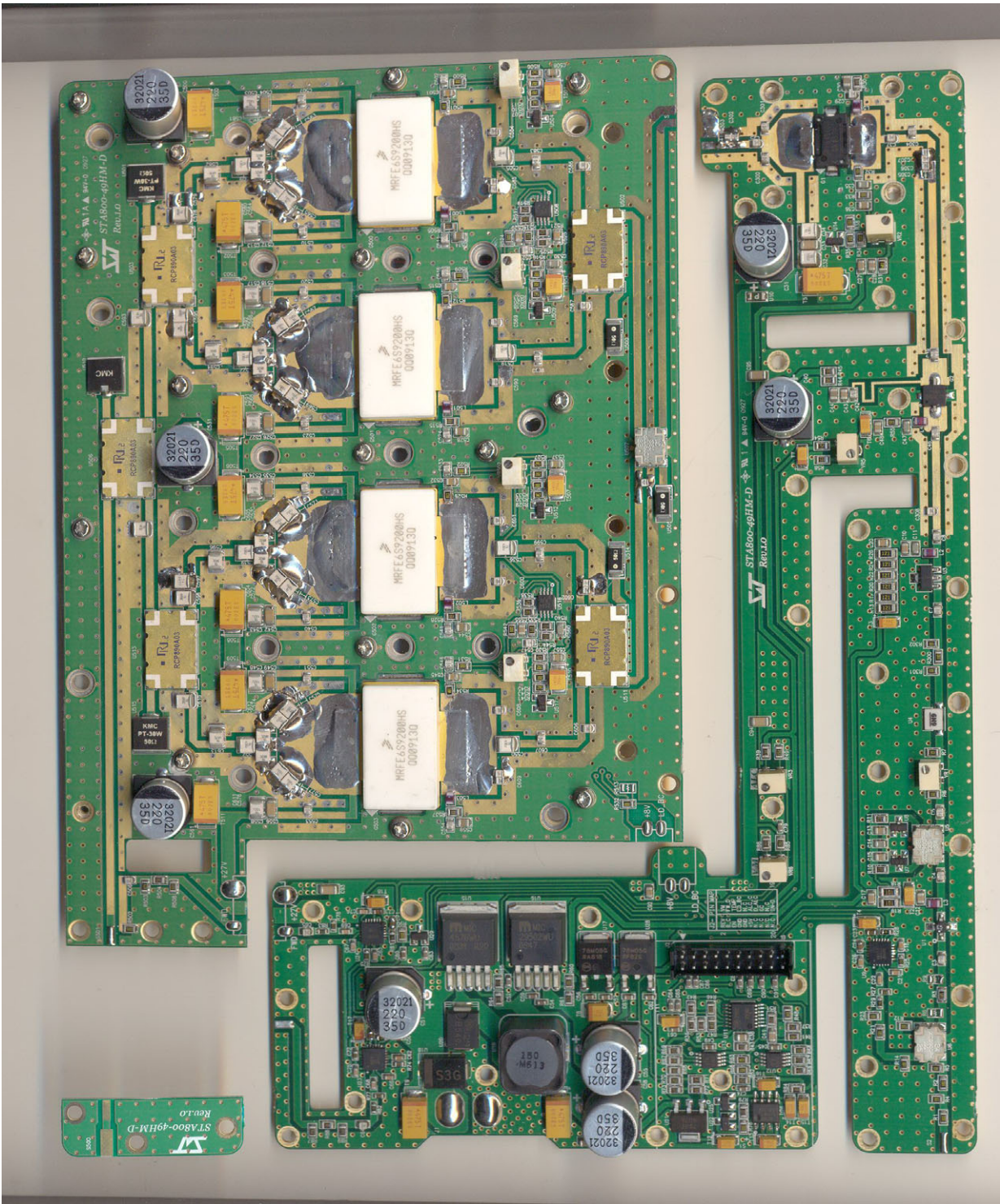
<Photograph 2: (AMP) FRONT view>
