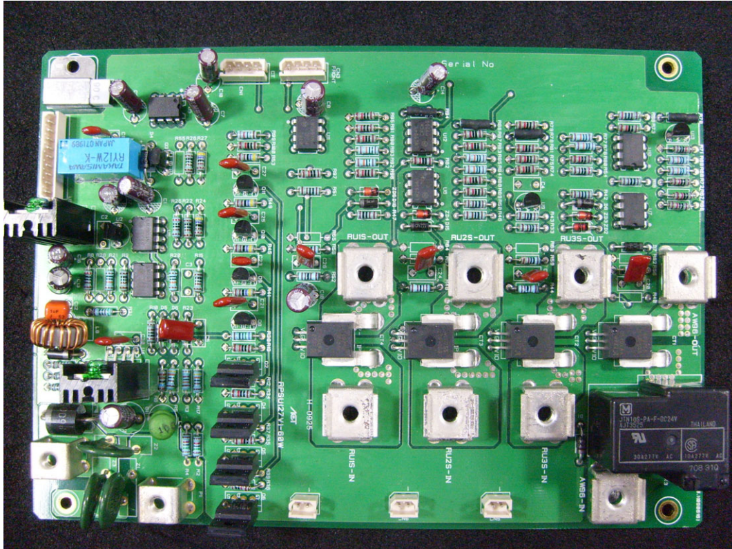
&lt;Photograph 18: (RPSU board) FRONT view&gt;
