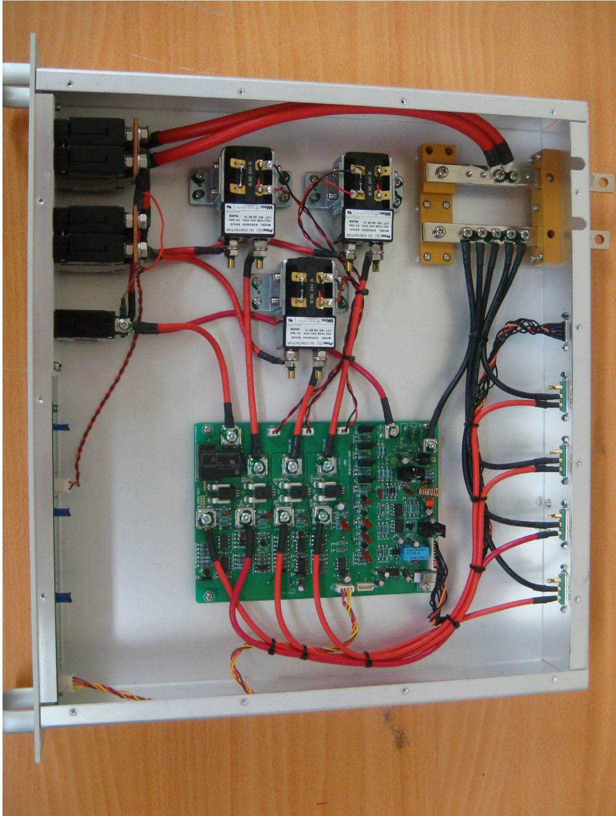
<Photograph 17: RPSU - Cover removed>
