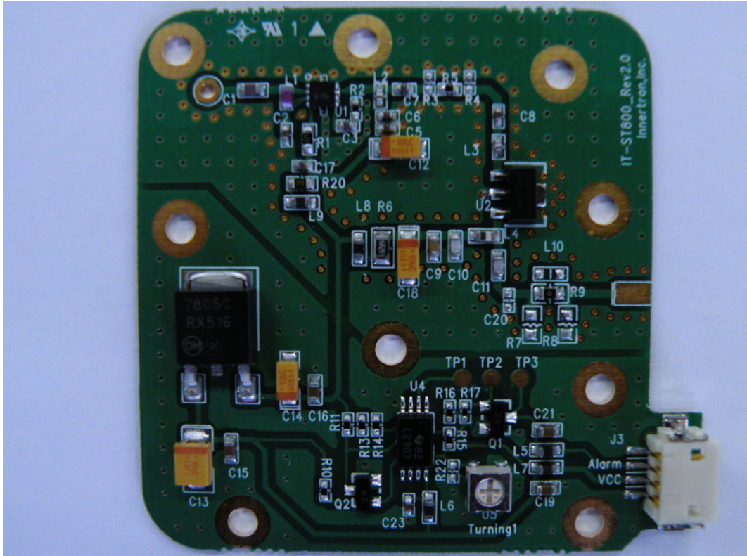
&lt;Photograph 15: (LNA) FRONT view&gt;
