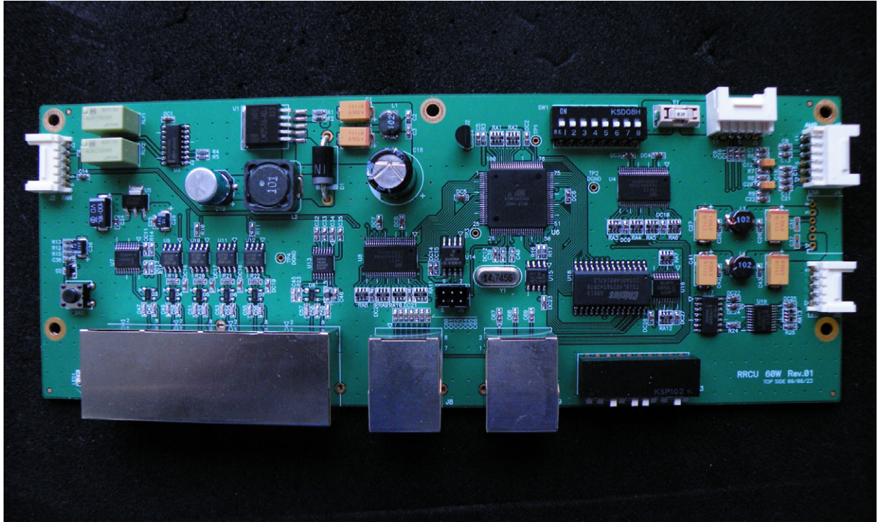
&lt;Photograph 6: (RRCU) FRONT view&gt;
