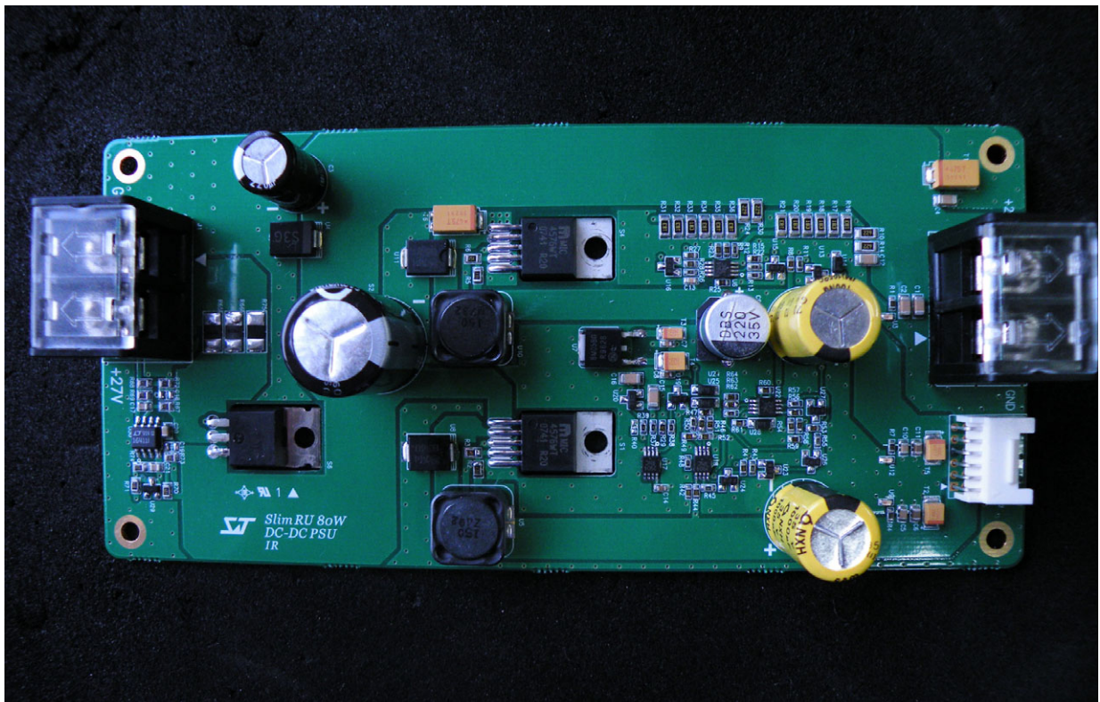
&lt;Photograph 9: (DC-DC converter) REAR view&gt;
