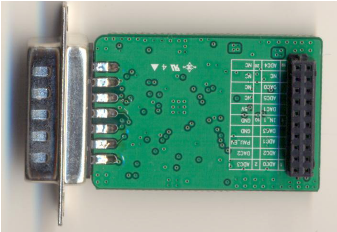
<Photograph 5: (AMP - control board) REAR view>
