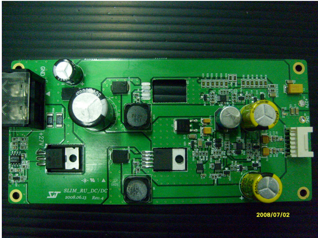
<Photograph 6: Internal - (DC-DC converter) FRONT view>
