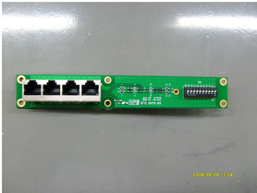
&lt;Photograph 12: Internal - (RJ45) FRONT view&gt;
