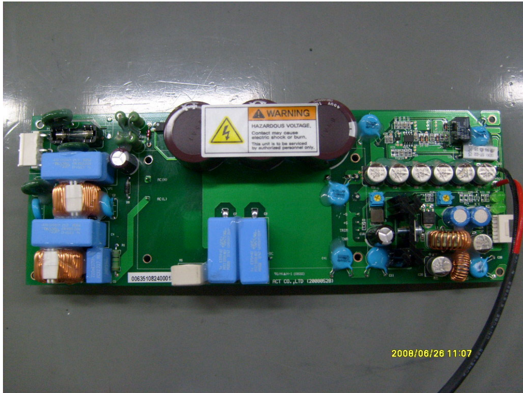
&lt;Photograph 6: Internal - (AC-DC converter) FRONT view&gt;
