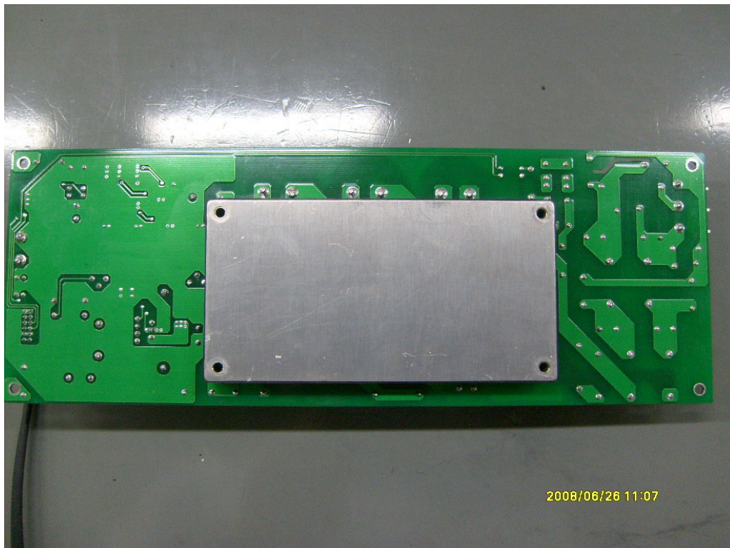
&lt;Photograph 7: Internal- (AC-DC converter) REAR view&gt;
