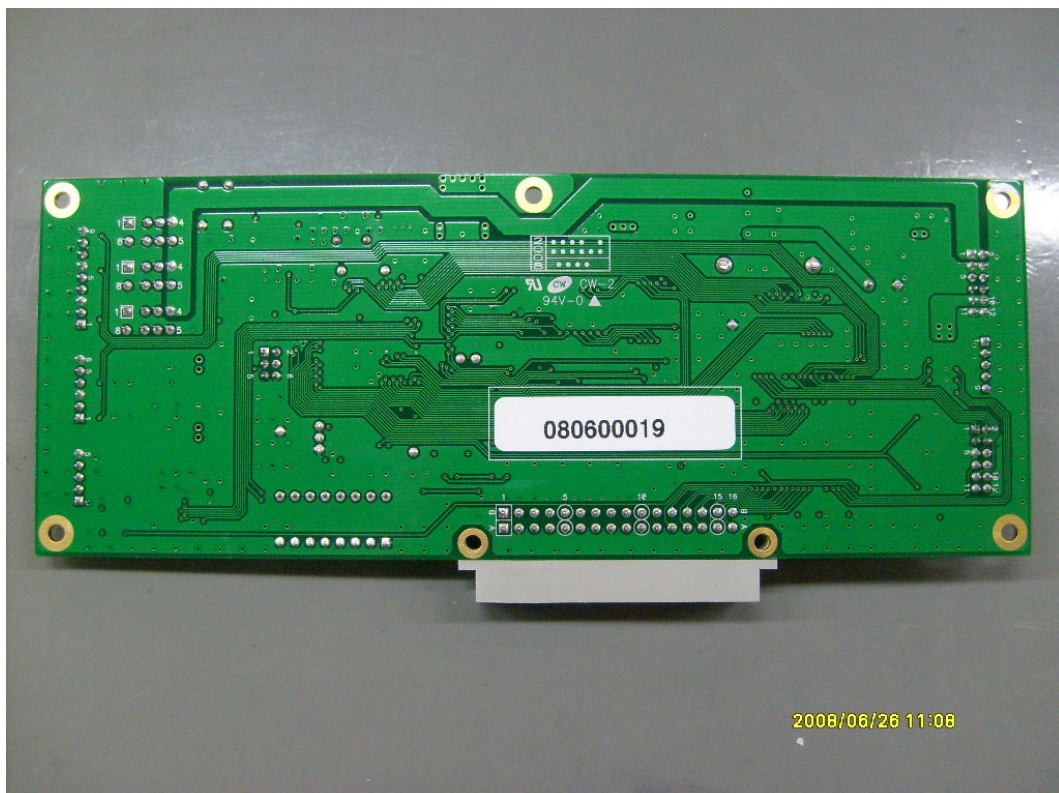
&lt;Photograph 11: Internal- (RRCU) REAR view&gt;
