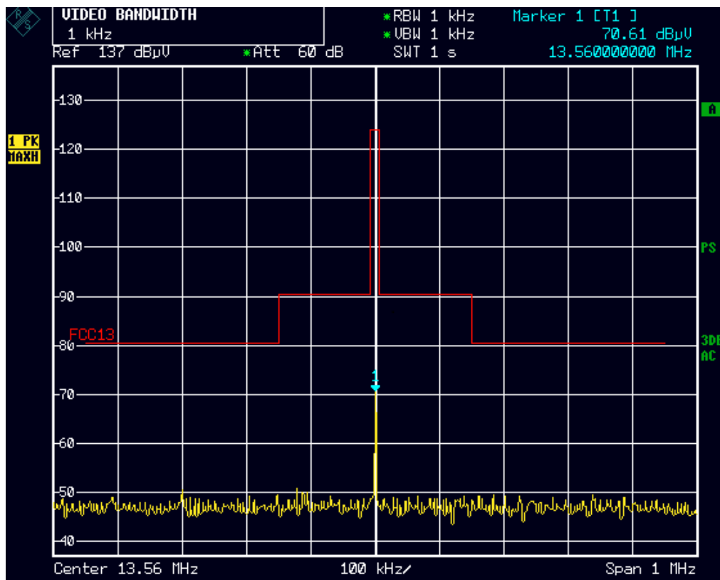
Figure 4: Spectrum Mask
