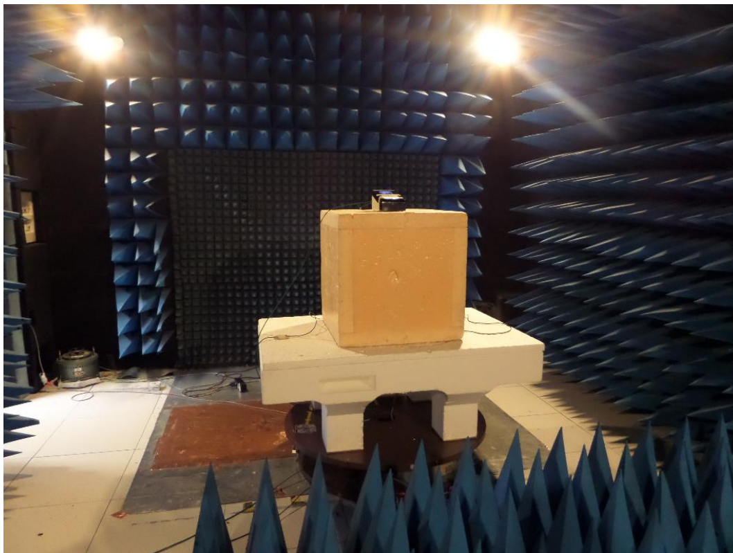
Anechoic chamber setup
