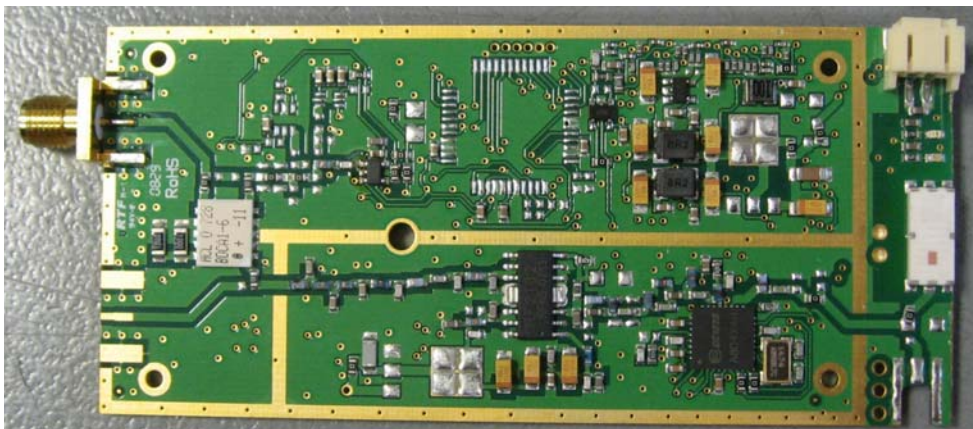
Radio board: front view
