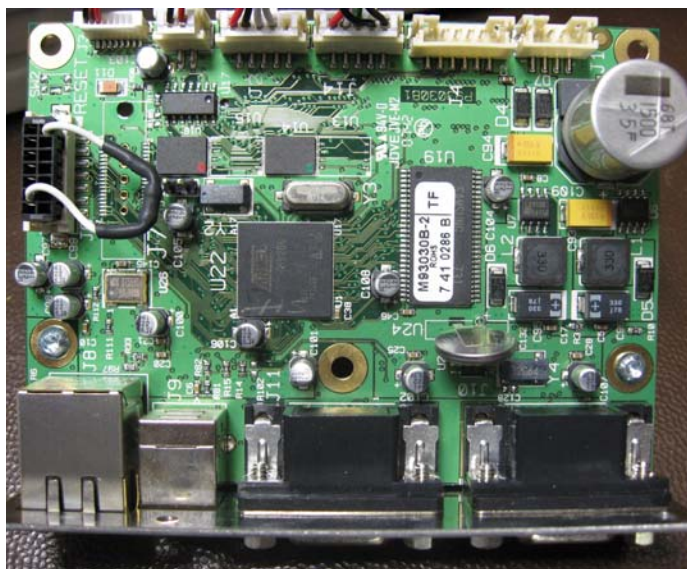
Link board: rear view
