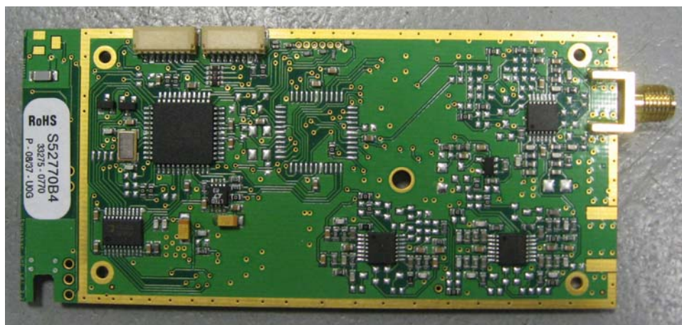
Radio board: rear view
