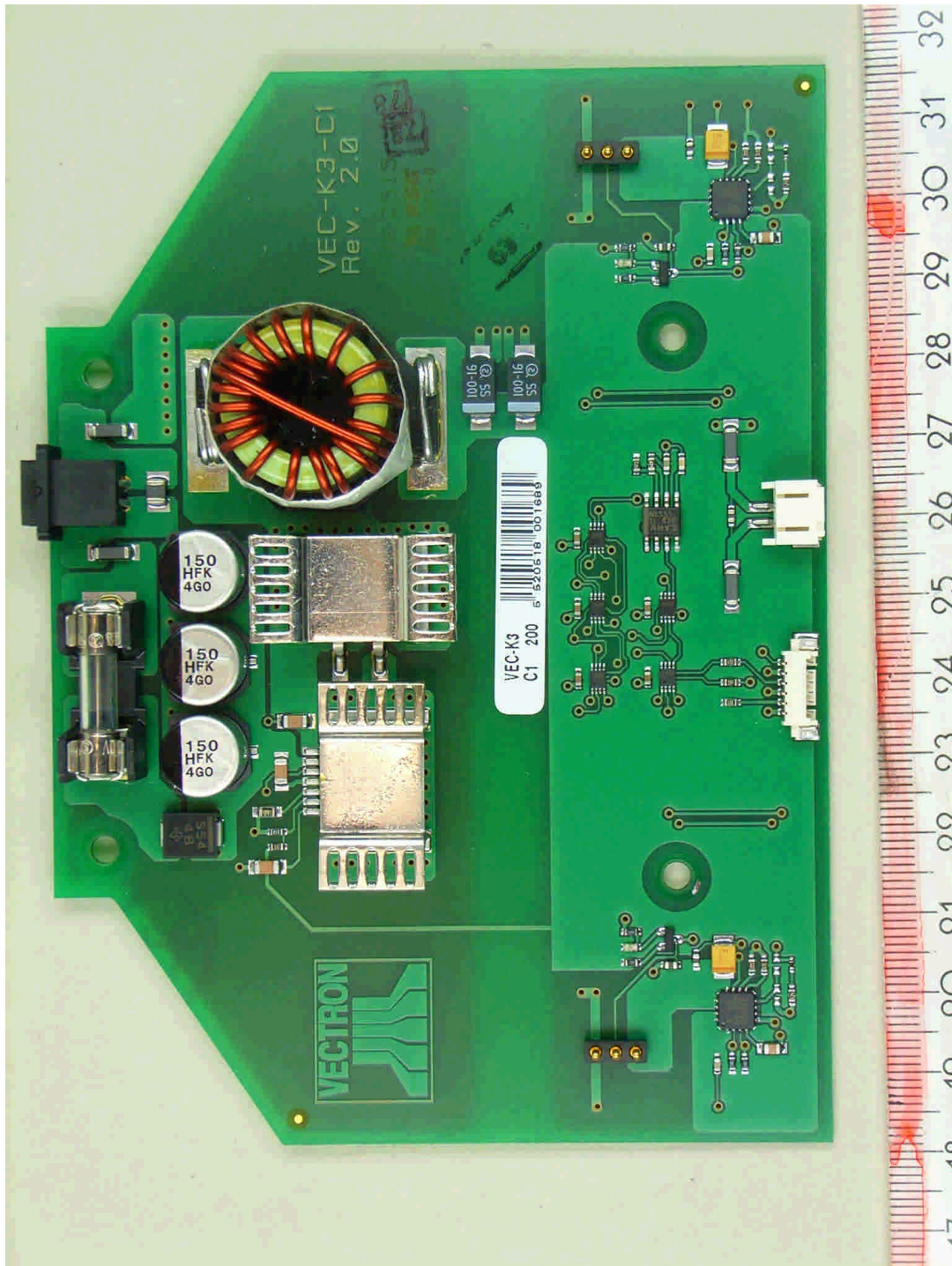
80804_g2.jpg POS MobilePro charging station, PCB, top view
