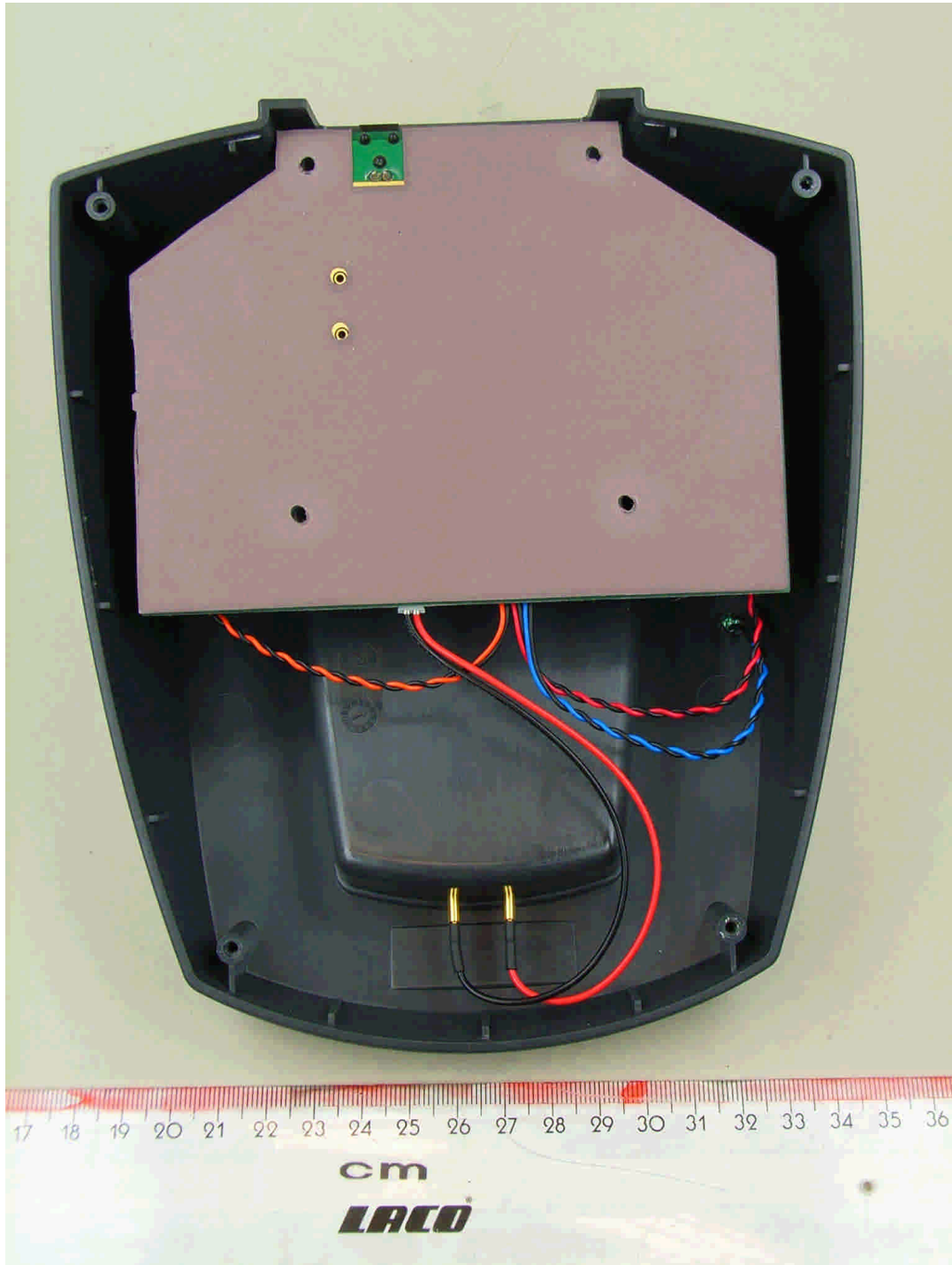
80804_e2.jpg POS MobilePro charging station, internal view, metal plate removed
