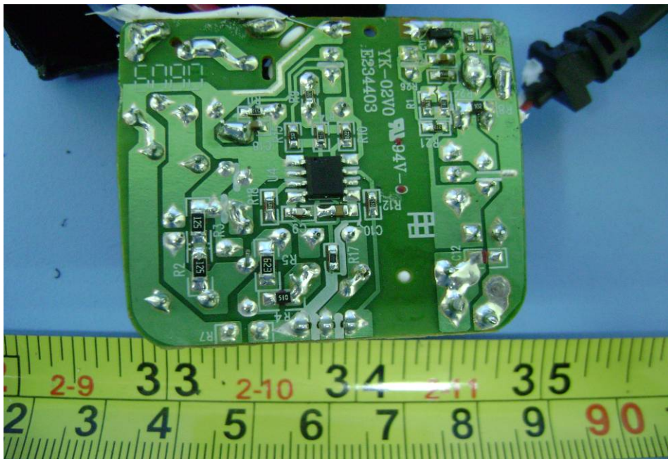
Adapter PCB– Back View
